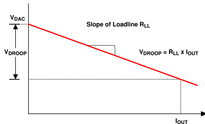
✎ 7. Load Line
