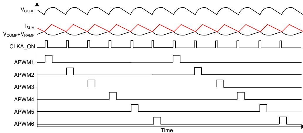
✎ 6. D-CAP+ Mode Basic Waveforms
