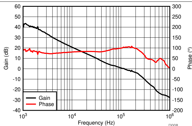
Figure 95. Bode Plot
