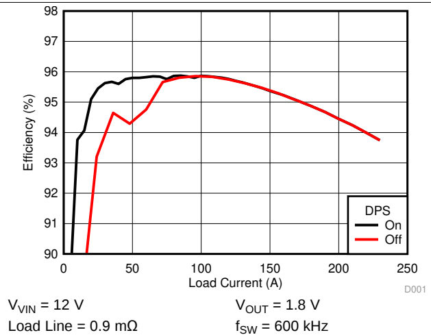
FIG 3. Efficiency
