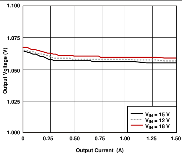
FIG 6-3. 1.05-V Output Voltage vs. Output Current
