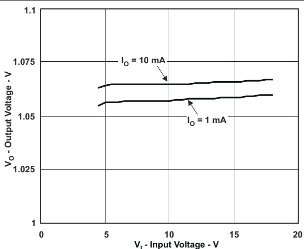
FIG 6-4. 1.05-V Output Voltage vs. Input Voltage
