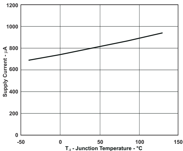
FIG 6-1. V CC Supply Current vs. Junction Temperature
