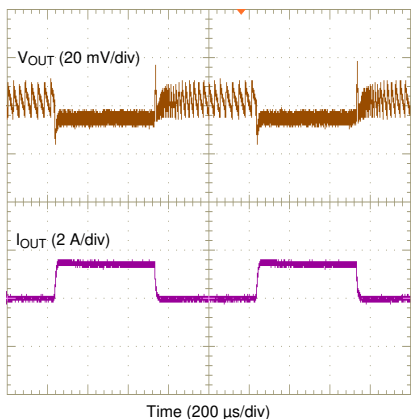
FIG 6-5. Load Transient Response, 1.05 V, 0 A to 1.5 A
