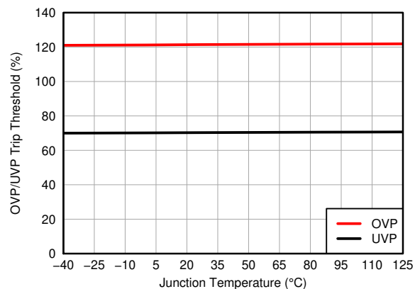
6-4. OVP/UVLP Trip Threshold vs Junction Temperature
