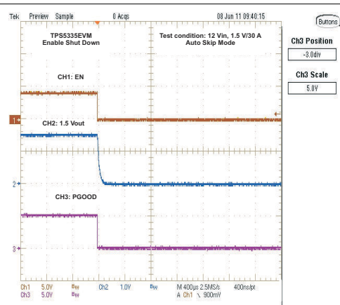
8-4. Enable Turn-off
