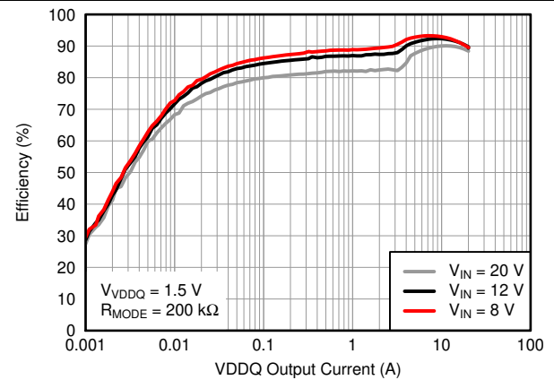
Figure 24. Efficiency
