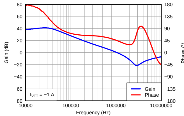
Figure 31. VTT Bode Plot (Sink)
