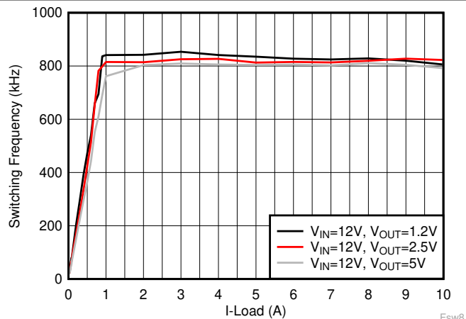
FIG 6-20. Switching Frequency vs Load Current, F_{SW} = 800 kHz, Eco-mode
