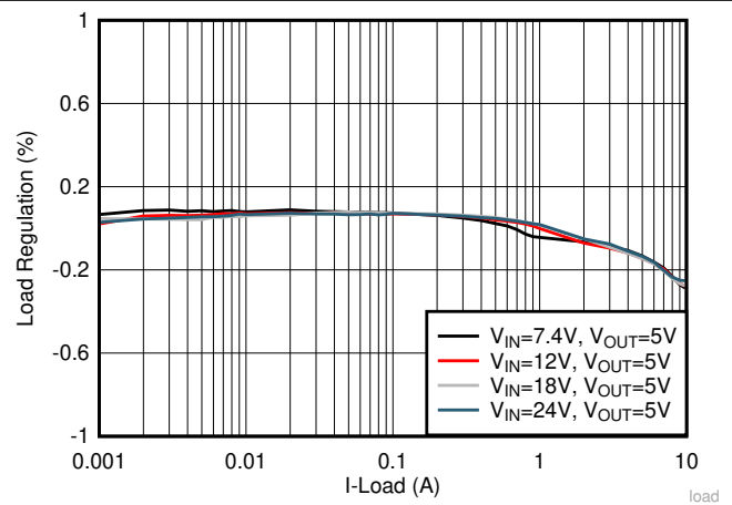
8-3. Load Regulation
