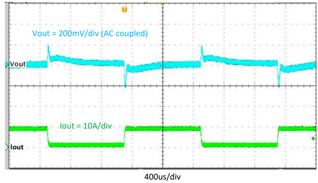
8-15. Transient Response, 1 A to 9 A, Slew Rate = 2.5\text{ A}/\mu\text{s}
