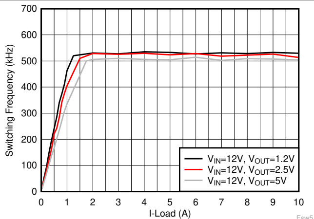
FIG 6-19. Switching Frequency vs Load Current, F_{SW} = 500 kHz, Eco-mode
