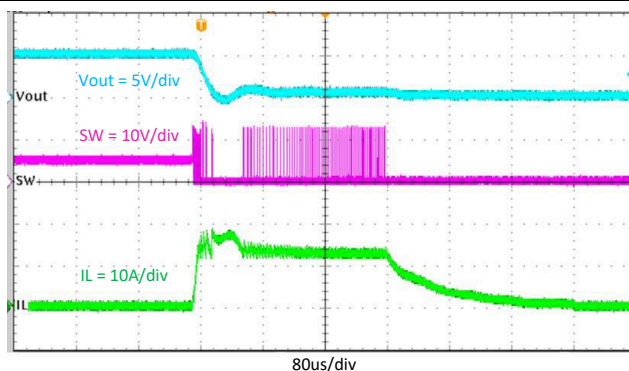
8-17. Normal Operation to Output Hard Short
