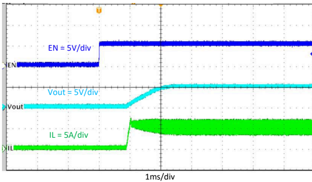
8-8. Start-Up Through EN, I_{OUT} = 5\text{ A}
