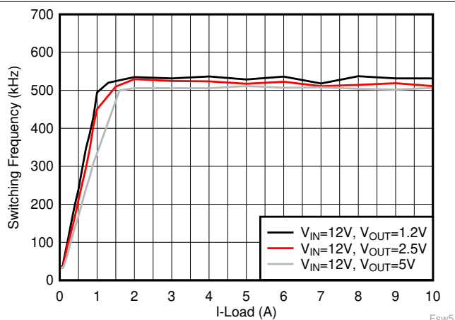
FIG 6-21. Switching Frequency vs Load Current, F_{SW} = 500 kHz, OOA
