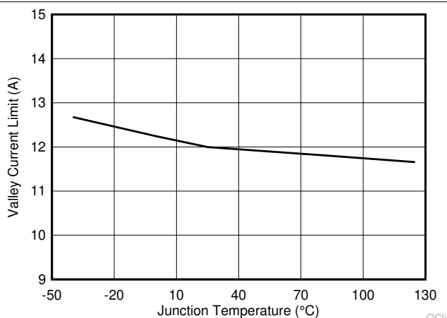
FIG 6-11. Valley Current Limit vs Junction Temperature
