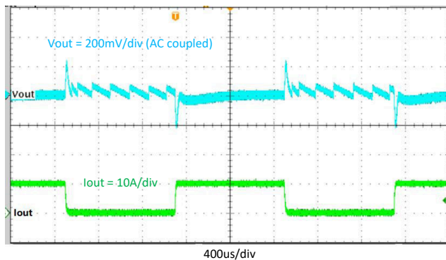
8-16. Transient Response, 0 A to 10 A, Slew Rate = 2.5\text{ A}/\mu\text{s}
