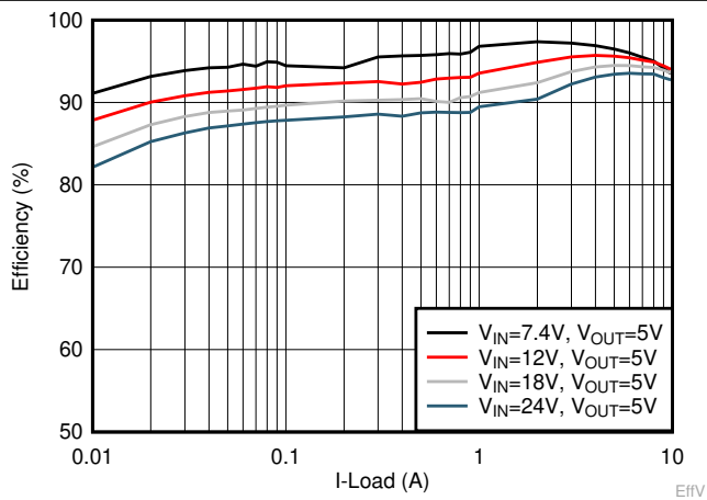
8-2. Efficiency Curve
