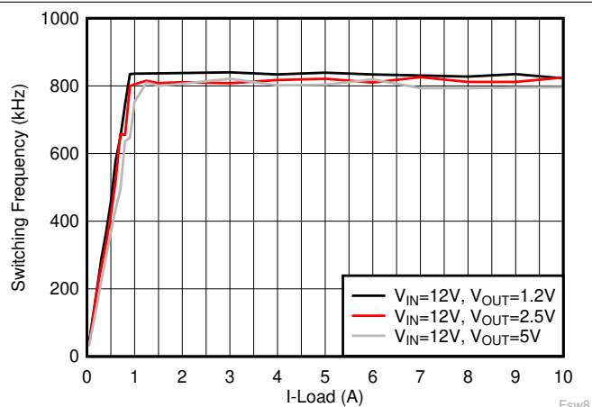
FIG 6-22. Switching Frequency vs Load Current, F_{SW} = 800 kHz, OOA
