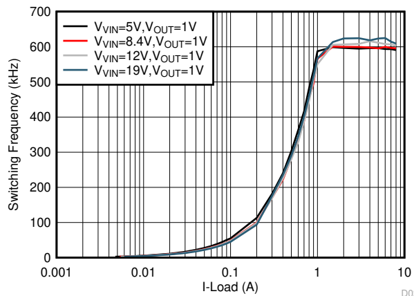
Figure 6-17. F_{SW} Load Regulation, Eco-mode, F_{SW} = 600 \text{ kHz}
