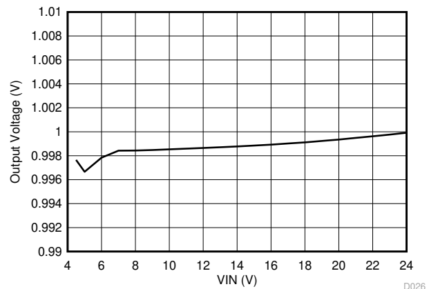
8-7. Line Regulation, I_{OUT} = 8\text{ A}
