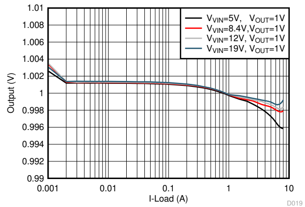
8-3. Load Regulation, F_{sw} = 600\text{ kHz}
