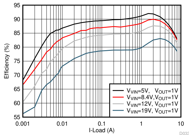
8-2. Efficiency Curve, F_{sw} = 600\text{ kHz}
