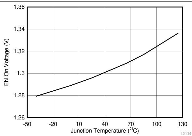
6-4. Enable On Voltage vs Junction Temperature
