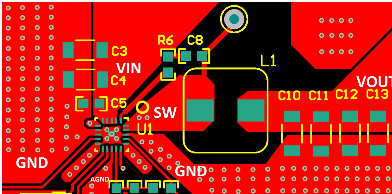
✕ 10-1. Top-Layer Layout
