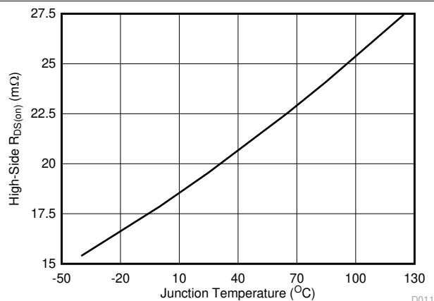
6-6. High-Side R_{DS(on)} vs Junction Temperature
