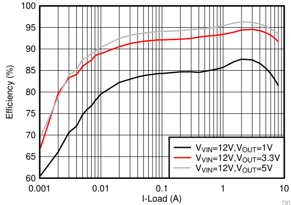
Figure 6-13. Efficiency, Eco-mode, F_{SW} = 600 \text{ kHz}
