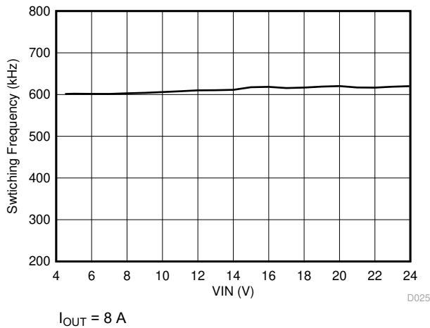
8-4. Switching Frequency vs Input Voltage
