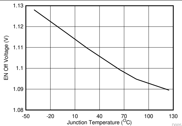
6-5. Enable Off Voltage vs Junction Temperature
