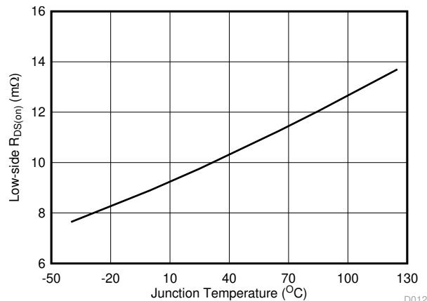
6-7. Low-Side R_{DS(on)} vs Junction Temperature
