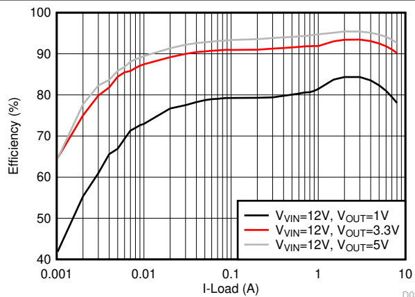
Figure 6-15. Efficiency, Eco-mode, F_{SW} = 1 \text{ MHz}
