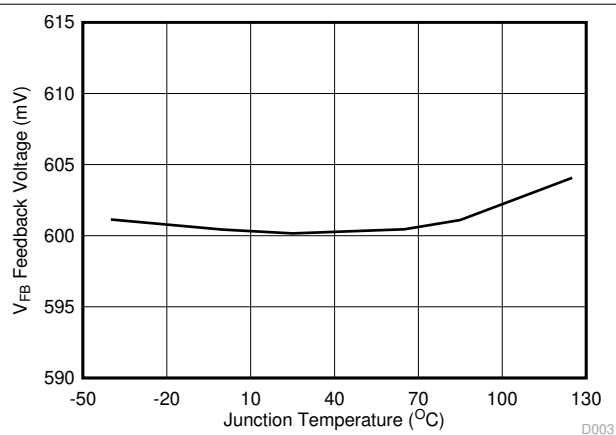
6-3. Feedback Voltage vs Junction Temperature
