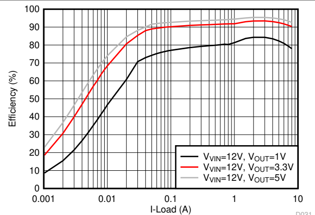
Figure 6-16. Efficiency, OOA-mode, F_{SW} = 1 \text{ MHz}
