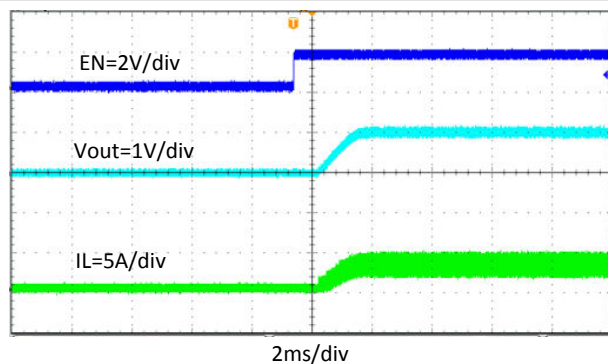
8-10. Start-Up Through EN, I_{OUT} = 4 \text{ A}
