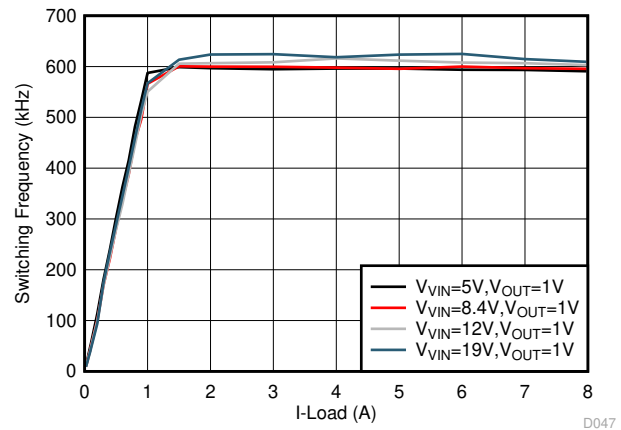
8-5. Switching Frequency vs Output Load
