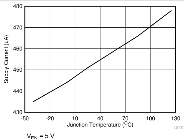
6-1. Supply Current vs Junction Temperature
