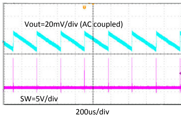
8-8. Output Voltage Ripple, I_{OUT} = 0.01 \text{ A}
