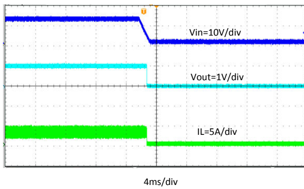
8-13. Start Up Relative to V_{IN} Falling, I_{OUT} = 4 \text{ A}
