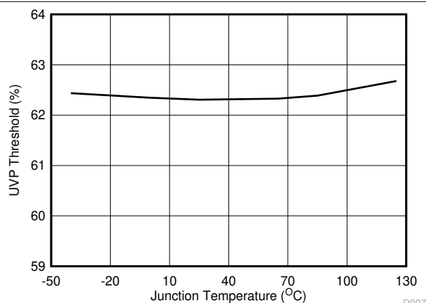
6-9. UVP Threshold vs Junction Temperature
