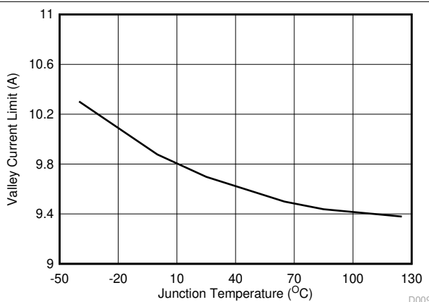
6-11. Valley Current Limit vs Junction Temperature
