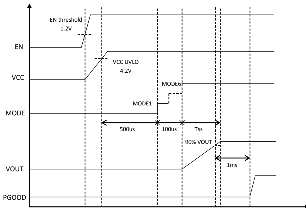
7-1. Power-Up Sequence
