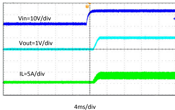
8-12. Start Up Relative to V_{IN} Rising, I_{OUT} = 4 \text{ A}
