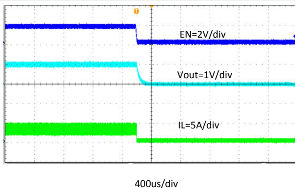
8-11. Shut-down Through EN, I_{OUT} = 4 \text{ A}
