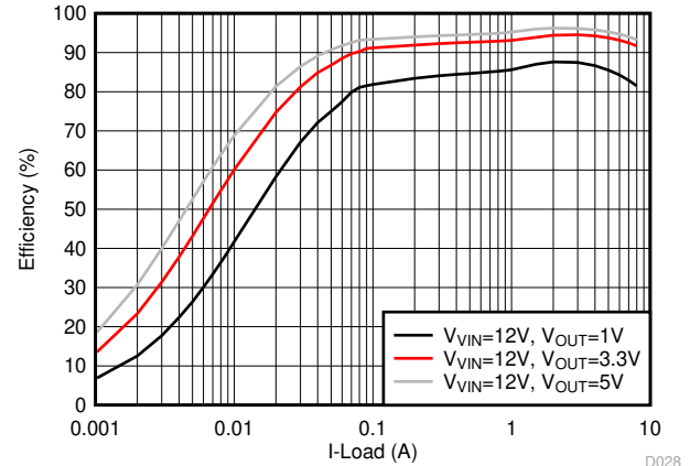
Figure 6-14. Efficiency, OOA-mode, F_{SW} = 600 \text{ kHz}
