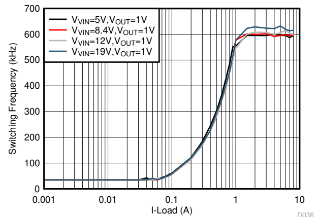
Figure 6-18. F_{SW} Load Regulation, OOA-mode, F_{SW} = 600 \text{ kHz}
