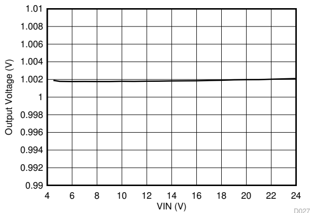
8-6. Line Regulation, I_{OUT} = 0.01\text{ A}
