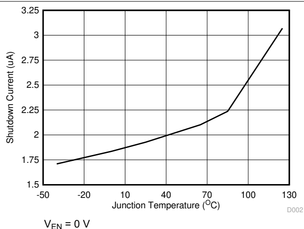
6-2. Shutdown Current vs Temperature
