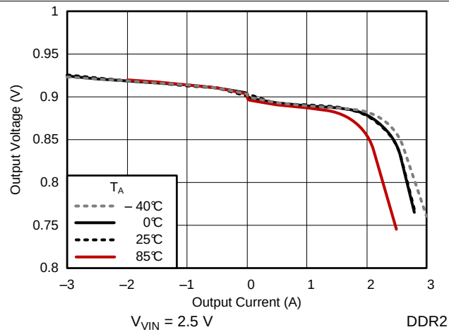
Figure 7. Output Voltage vs Output Current
