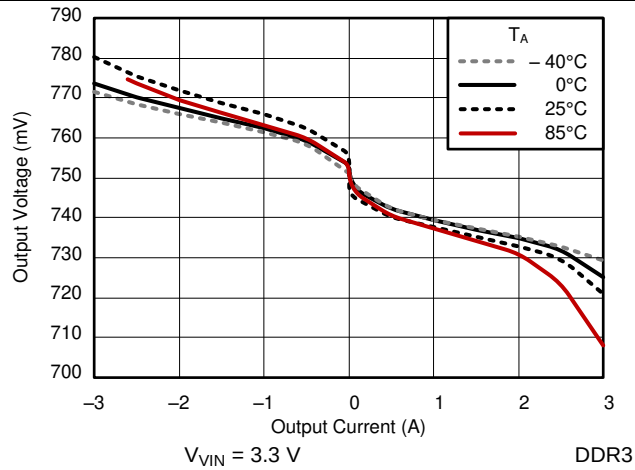
Figure 3. Load Regulation
