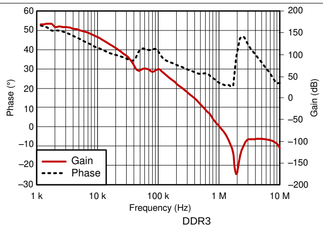
Figure 18. Bode Plot
