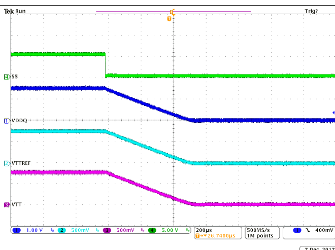
Figure 45. Shutdown Waveforms
