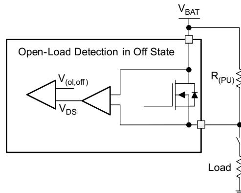
Figure 30. Open-Load Detection in Off-State
