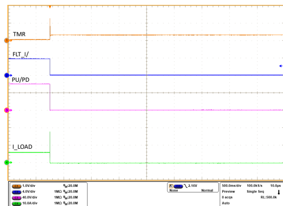
図 9-11. Latch-off Response of TPS48110-Q1 for an Overcurrent Fault
