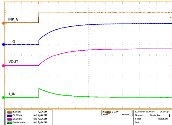
9-15. Pre-charge Profile of the Output Capacitance (VIN = 48 V, C OUT = 440 \mu F, No Load)
