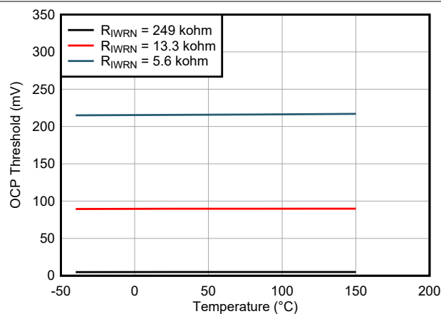
Figure 6-7. Overcurrent Threshold ( V_{SNS\_WRN} ) vs Temperature
