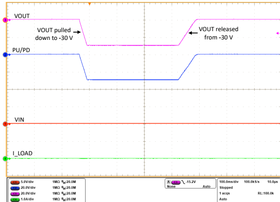
Figure 8-14. Output Short to -30 V Response with VIN = 0 V and INP = LOW
