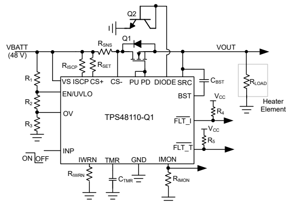
図 9-1. Typical Application Schematic: Driving HVAC PTC Heater
