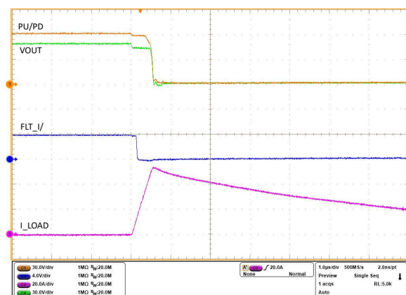
図 9-13. Output Hot-Short Response of the TPS48110-Q1 Device
