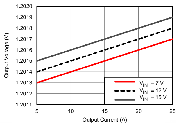
Figure 25. Load Regulation
