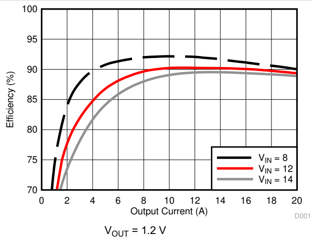
Figure 9-2. Efficiency vs Output Current
