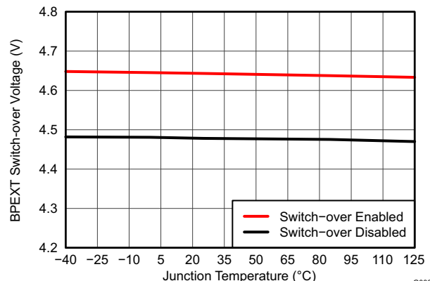
7-1. BPEXT Switch-over Voltage vs. Junction Temperature
