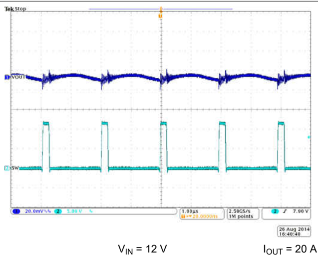
Figure 9-6. Output Voltage Ripple
