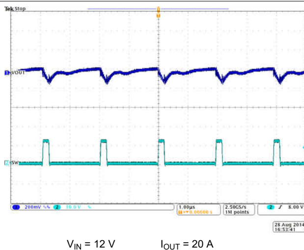
Figure 9-7. Input Voltage Ripple
