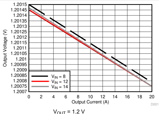
Figure 9-3. Line Regulation
