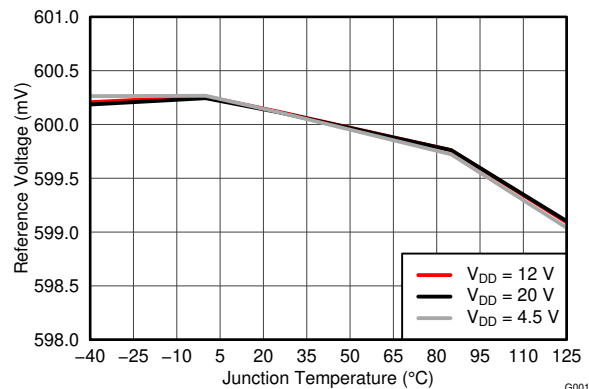
7-2. Reference Voltage vs. Junction Temperature
