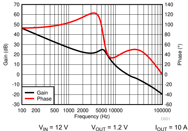
Figure 9-4. Bode Plot
