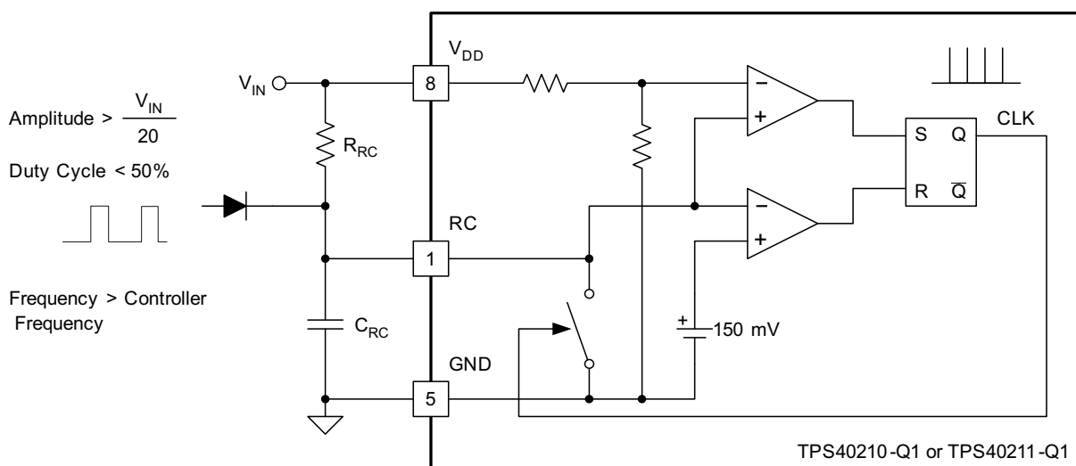
7-10. Diode Connected Synchronization
