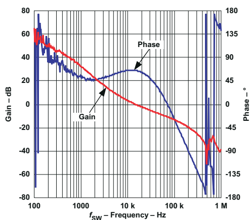
Figure 8-2. Gain and Phase vs Frequency
