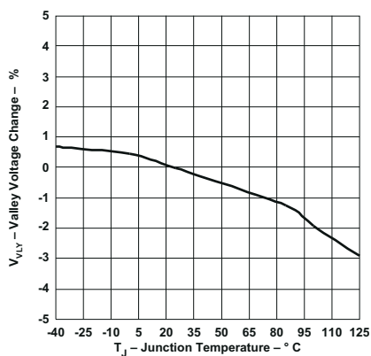
6-16. Valley Voltage Change vs Junction Temperature
