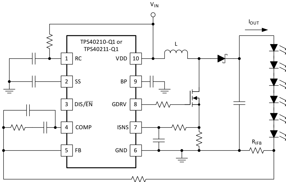
7-8. Typical LED Drive Schematic
