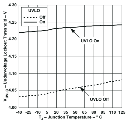
6-7. Undervoltage Lockout Threshold vs Junction Temperature
