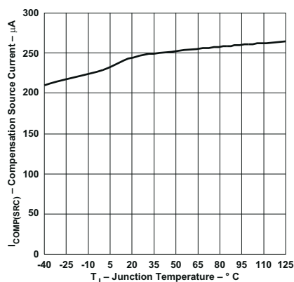
6-14. Compensation Source Current vs Junction Temperature
