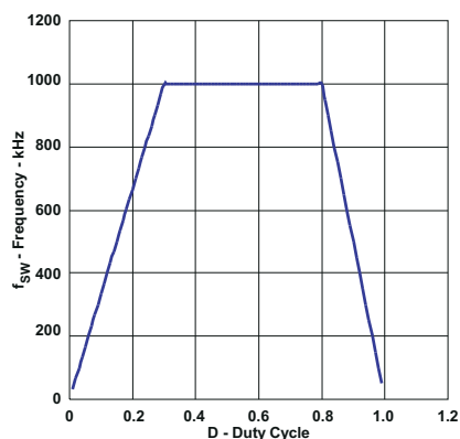
6-2. Switching Frequency vs Duty Cycle
