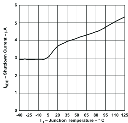
6-4. Shutdown Current vs Junction Temperature
