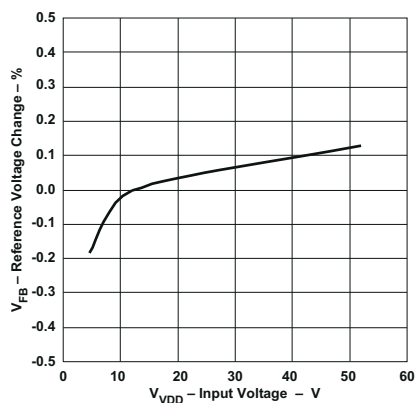
6-6. Reference Voltage Change vs Input Voltage
