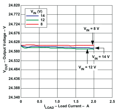
Figure 8-6. Output Voltage vs Load Current
