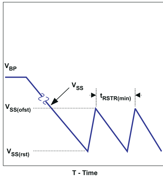
図 7-5. Soft Start During Overcurrent
