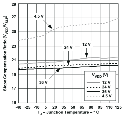
6-11. Oscillator Amplitude vs Junction Temperature
