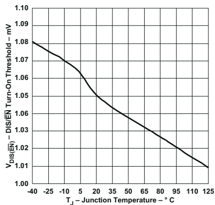
6-18. DIS/EN Turn-On Threshold vs Junction Temperature
