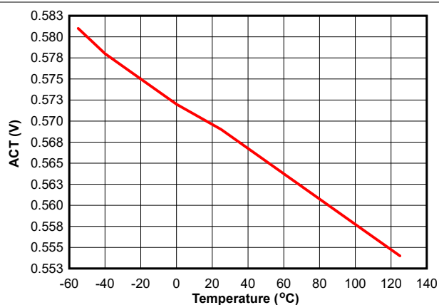
図 6-2. ACT Logic Low Threshold Voltage vs. Temperature
