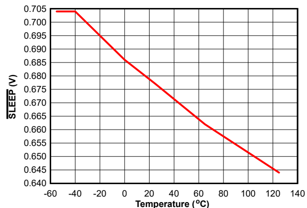
図 6-6. SLEEP Logic High Threshold Voltage vs. Temperature
