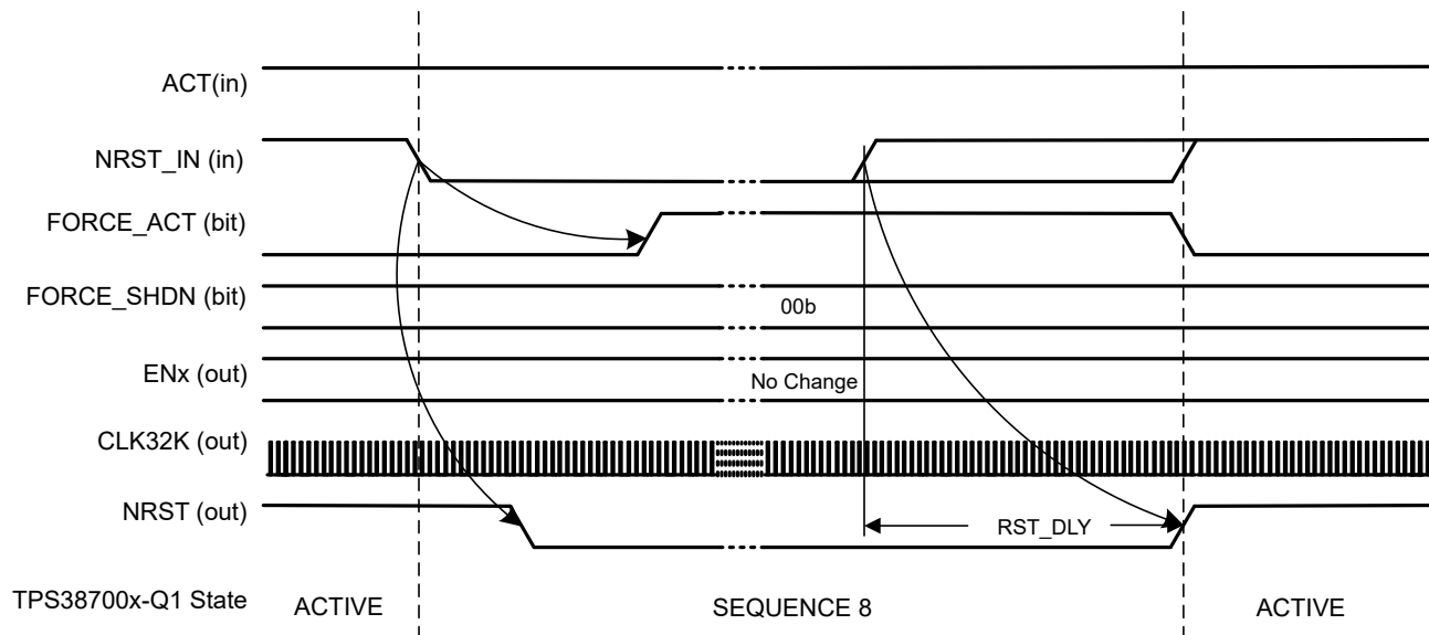
図 7-14. RESET due to NRST_IN
