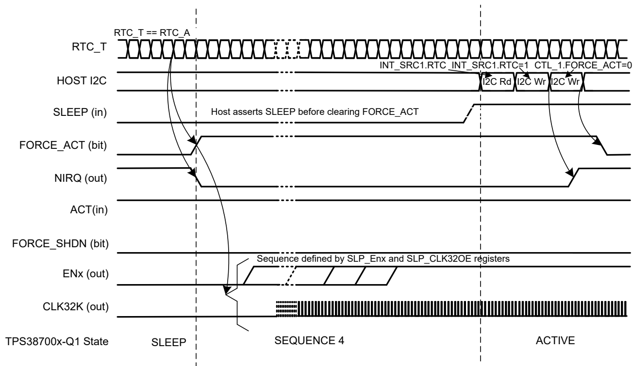
図 7-11. Sleep Exit RTC Triggered - Autonomous Sequencing
