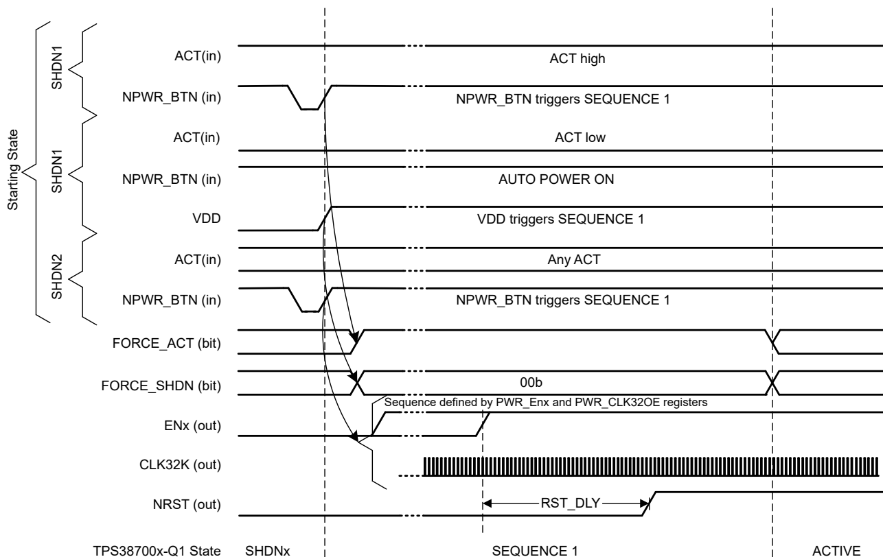
図 7-5. Power Up with NPWR_BTN Enabled
