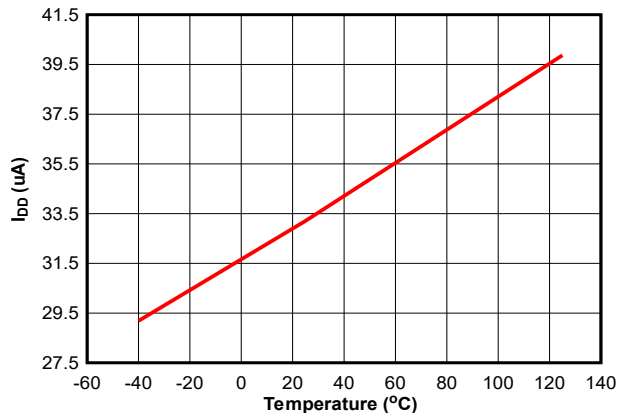
図 6-4. I_{DD} Shutdown Current vs. Temperature
