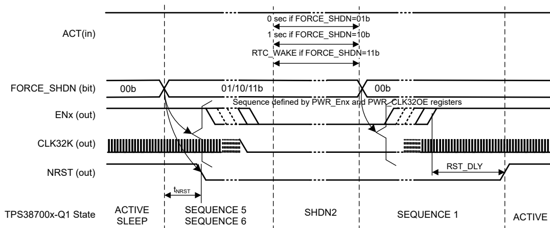
図 7-6. Power Up from SHDN2 - Software Shutdown with FORCE_SHDN ≠ 00b
