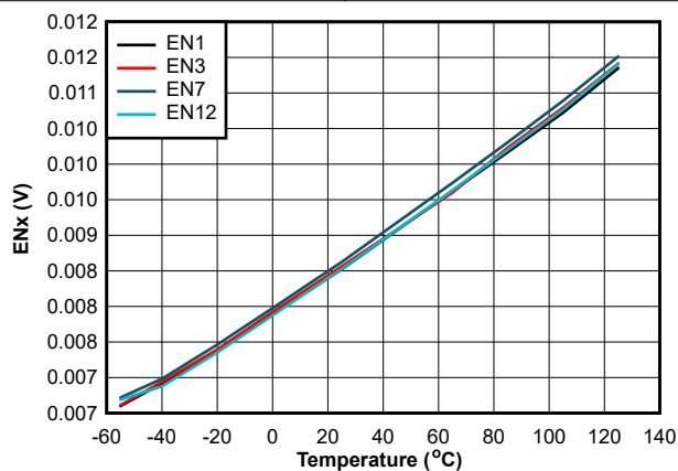
図 6-9. ENx Logic Low Output Voltage vs. Temperature
