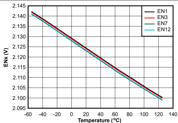
図 6-8. ENx Logic High Output Voltage vs. Temperature
