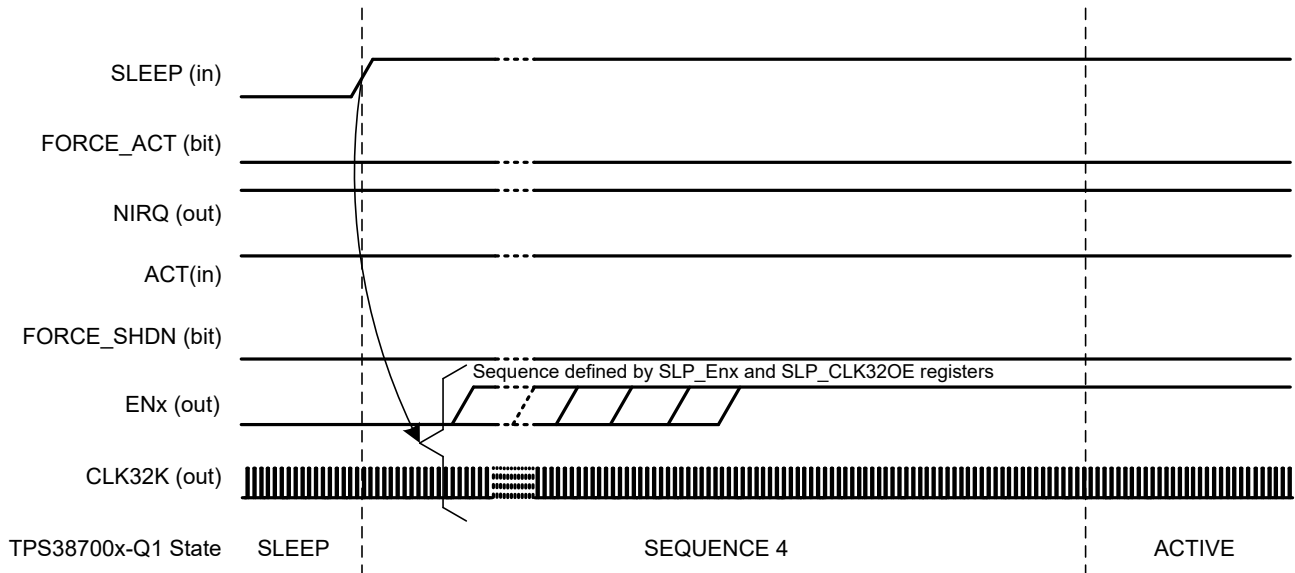
図 7-9. Sleep Exit \overline{\text{SLEEP}} Triggered
