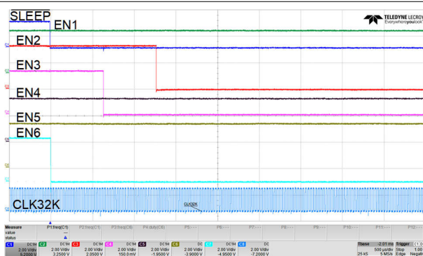
図 8-4. Sleep Entry Sequence
