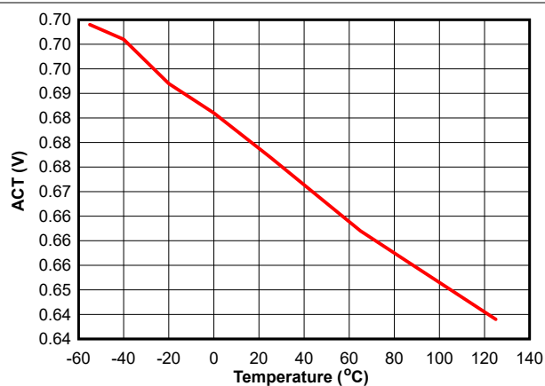
図 6-1. ACT Logic High Threshold Voltage vs. Temperature
