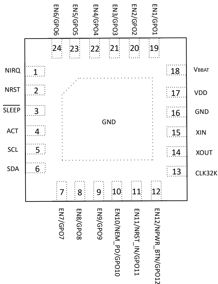
図 5-1. RGE Package 24-Pin VQFN TPS38700 Top View
