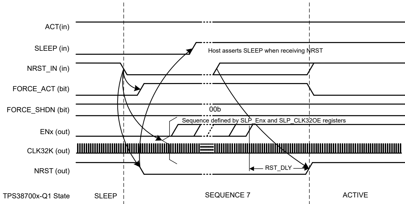
図 7-13. Sleep Exit due to NRST_IN
