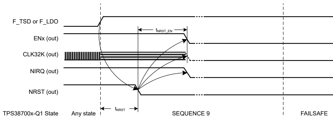
図 7-15. Failsafe Power Down
