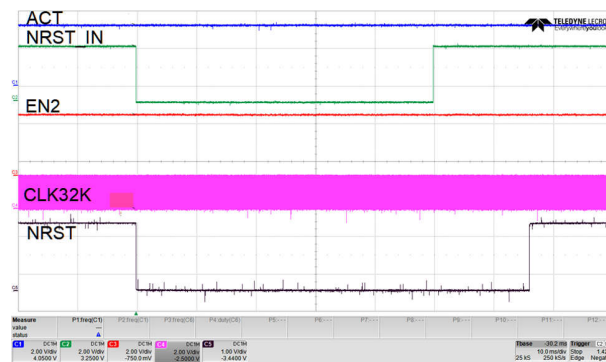
図 8-6. RESET Triggered by NRST_IN
