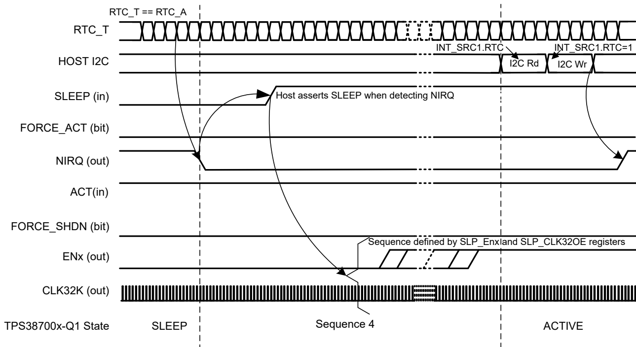
図 7-10. Sleep Exit RTC Triggered - \overline{\text{SLEEP}} Sequencing
