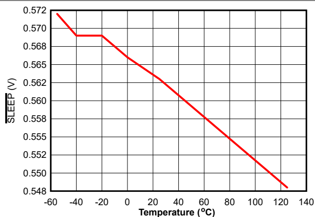
図 6-7. SLEEP Logic Low Threshold Voltage vs. Temperature
