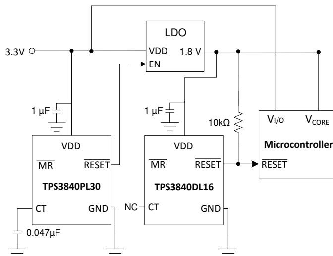
図 47. TPS3840-Q1 Voltage Rail Monitor and Power-Up Sequencer Design Block Diagram
