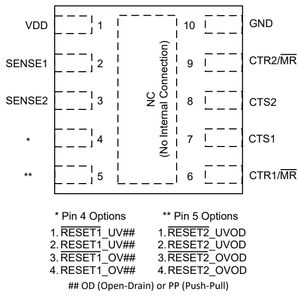
6-1. DSK Package, 10-Pin WSON, TPS38-Q1 (Top View)
