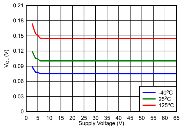
図 7-19. Open-Drain Active High V_{OL} vs V_{DD}
