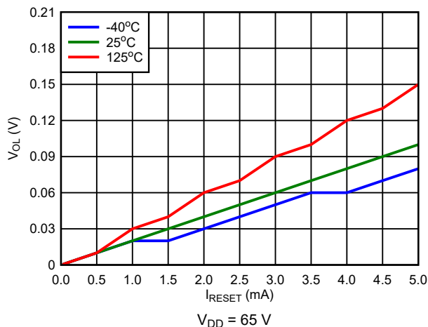
図 7-17. Push-Pull Active High V_{OL} vs I_{RESET}
