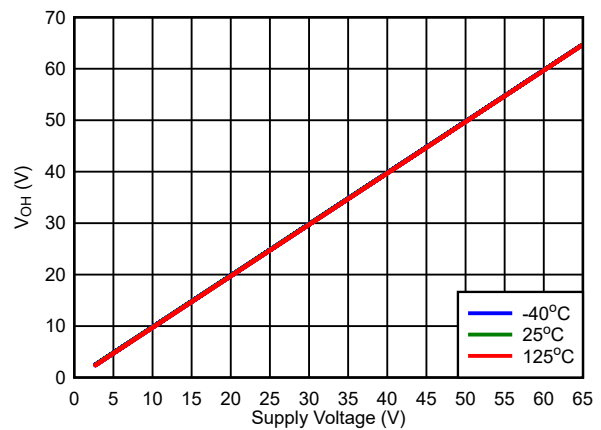
7-23. Push-Pull Active High V_{OH} vs V_{DD}
