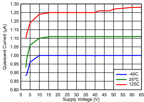
図 7-6. V_{DD} vs I_{DD} (RESET = High, V_{IT} = 2.7\text{ V} )
