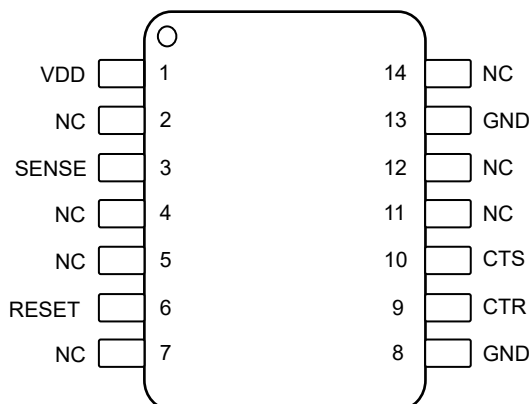
図 6-1. DYY Package, 14-Pin SOT-23, TPS3760-Q1 (Top View)
