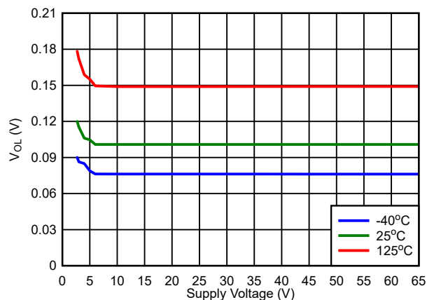
図 7-18. Open-Drain Active Low V_{OL} vs V_{DD}
