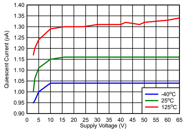
図 7-7. V_{DD} vs I_{DD} (RESET = Low, V_{IT} = 2.7\text{ V} )
