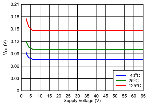
図 7-21. Push-Pull Active High V_{OL} vs V_{DD}
