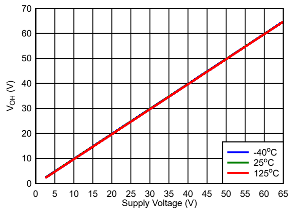
7-22. Push-Pull Active Low V_{OH} vs V_{DD}
