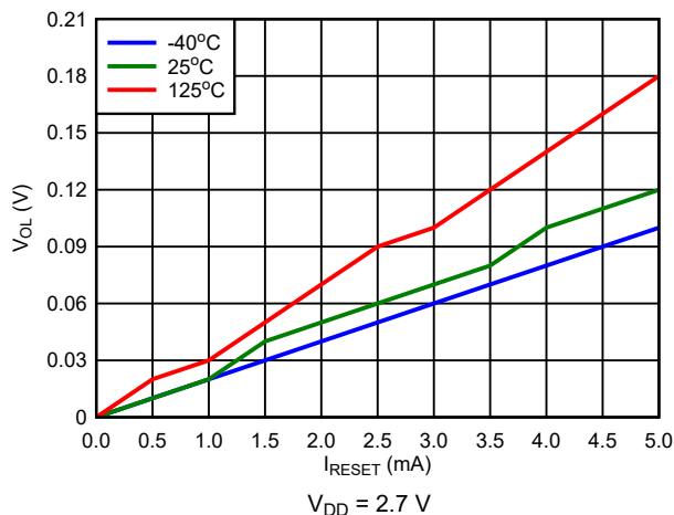
図 7-16. Push-Pull Active High V_{OL} vs I_{RESET}
