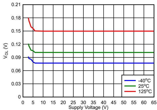
図 7-20. Push-Pull Active Low V_{OL} vs V_{DD}
