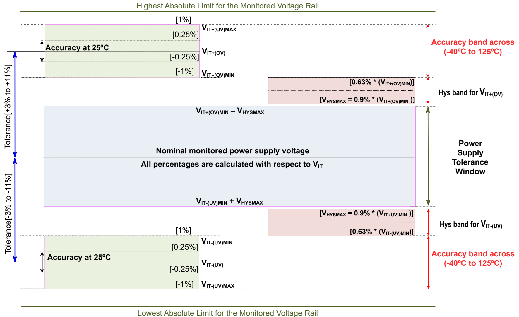
図 7-1. Voltage Threshold and Hysteresis Accuracy
