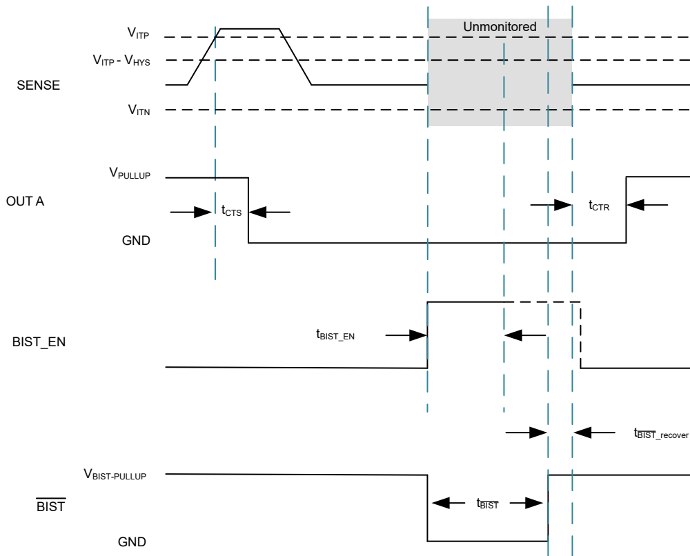
図 7-8. TPS37102 Latch Disable
