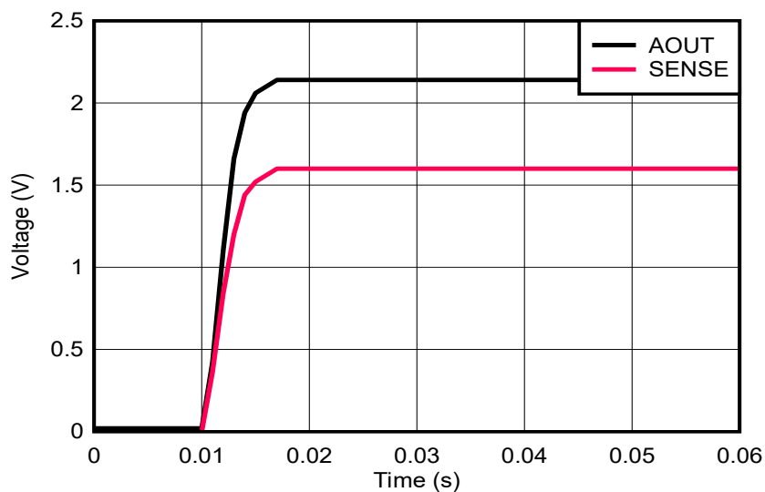
図 7-7. AOOUT following SENSE pin.
