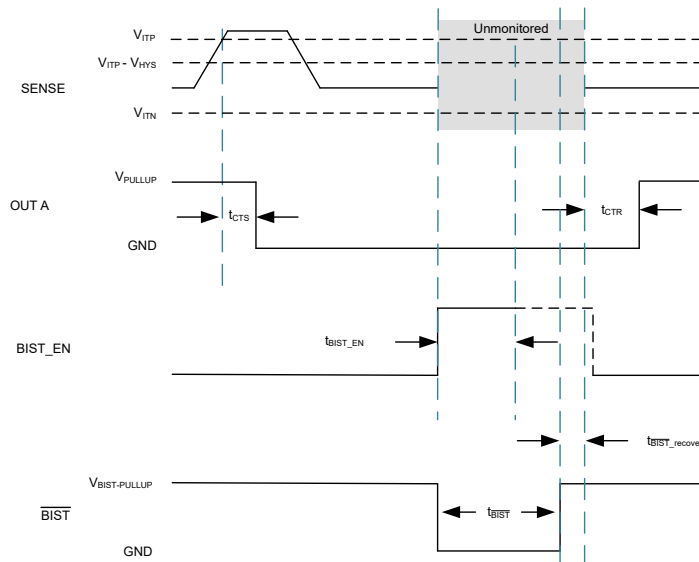
図 7-6. OUT A Latch and Unlatch
