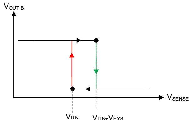
図 7-5. Hysteresis (Undervoltage Active-Low)
