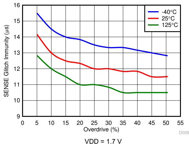
7-11. SENSE Glitch Immunity (VIT-) vs Overdrive
