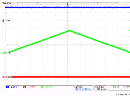
9-12. TPS3703-Q1 SENSE Ramp Latch Function
