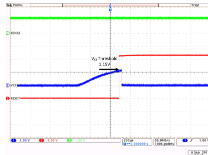
9-13. TPS3703-Q1 CT Bias Unlatch Function
