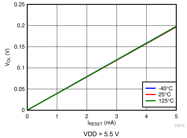
FIG 7-16. Low-Level Output Voltage vs RESET current
