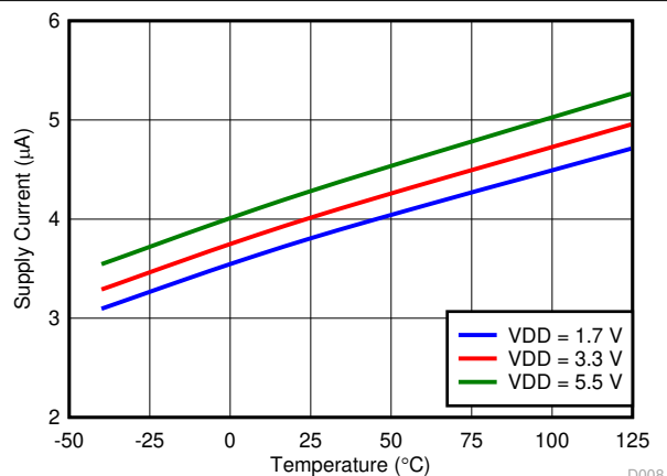
Output ( RESET Pin) = Low 7-10. Supply Current vs Temperature
