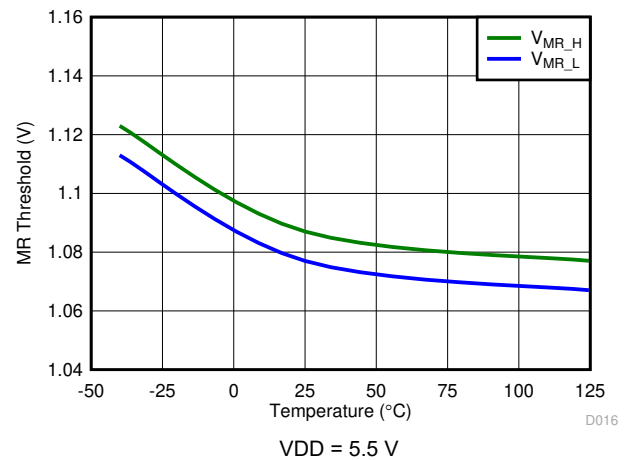
FIG 7-18. SET Threshold vs Temperature
