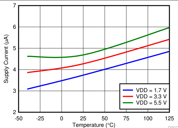
Output ( RESET Pin) = High 7-9. Supply Current vs Temperature
