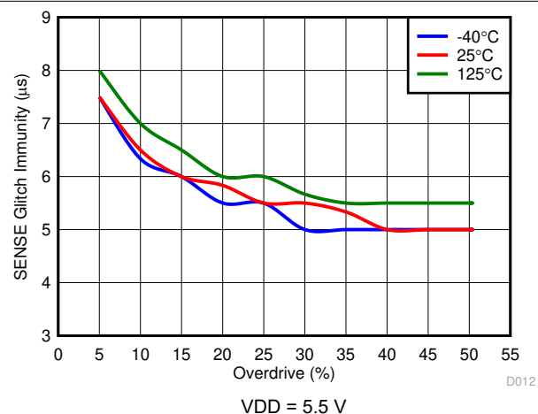
7-14. SENSE Glitch Immunity ( V_{IT+} ) vs Overdrive
