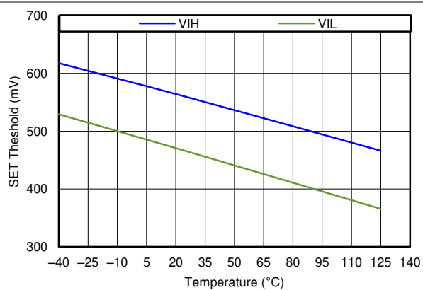
FIG 5-14. SET Threshold vs Temperature
