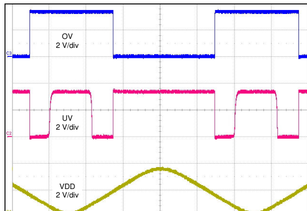
7-8. TPS3702CX33 Startup with V_{\text{PULL-UP}} = 3\text{V}
