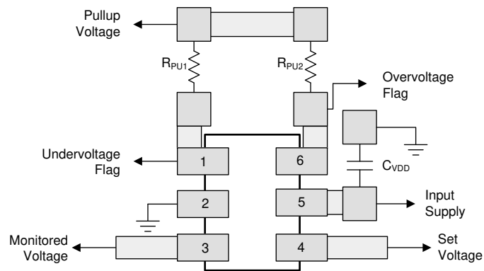
☒ 9-1. Recommended Layout
