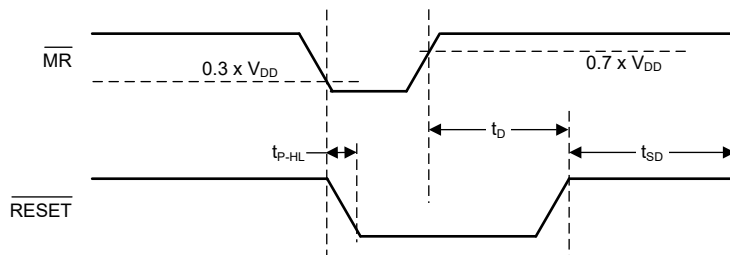
8-12. \overline{MR} Pin Response
