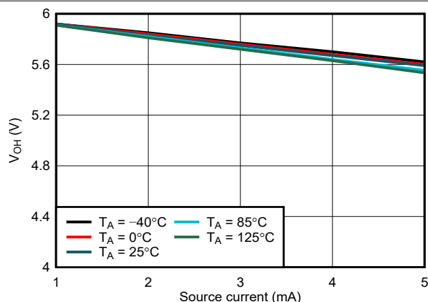
7-17. WDO V_{OH} vs I_{source} , V_{DD} = 6.0\text{ V}
