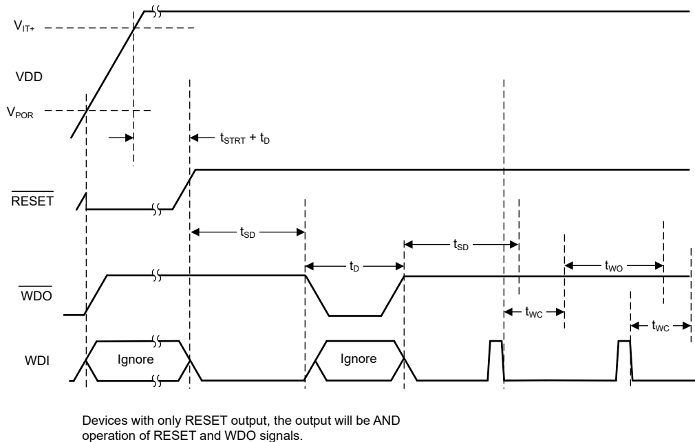
図 8-8. t_{SD} Frame Behavior
