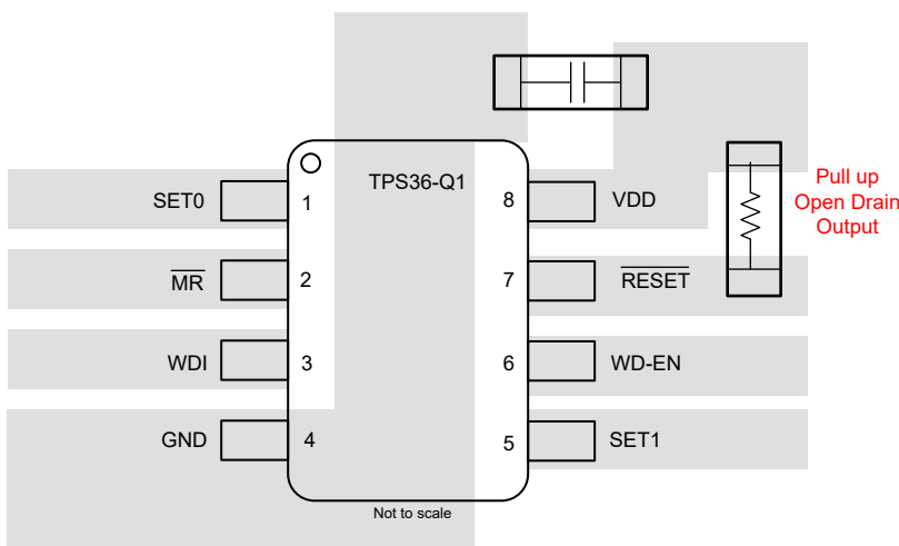
✎ 9-3. Typical Layout for the pinout C of TPS36-Q1
