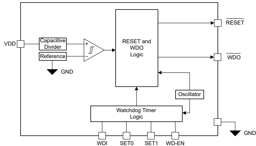
8-4. Pinout Option D
