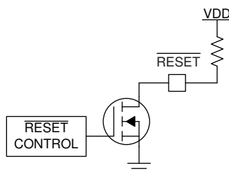
図 9-2. Open-Drain \overline{\text{RESET}} Configuration
