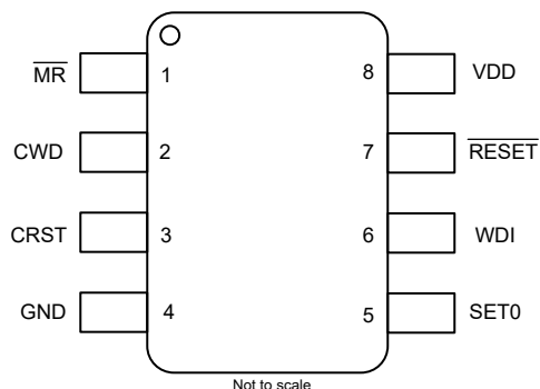
6-1. Pin Configuration Option A DDF Package, 8-Pin SOT-23, TPS36-Q1 Top View
