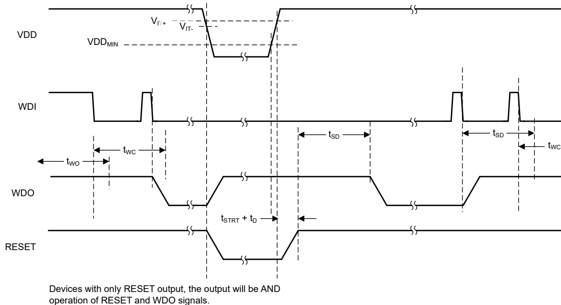
図 8-13. Output Latch Timing Behavior
