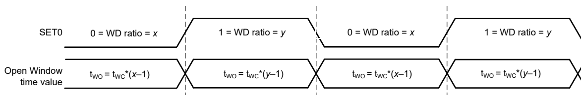
8-10. Watchdog Operation with 2 SET Pins
