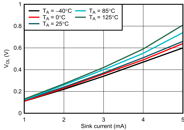
Figure 7-10. RESET V_{OL} vs I_{sink} , V_{DD} = 1.5\text{ V}
