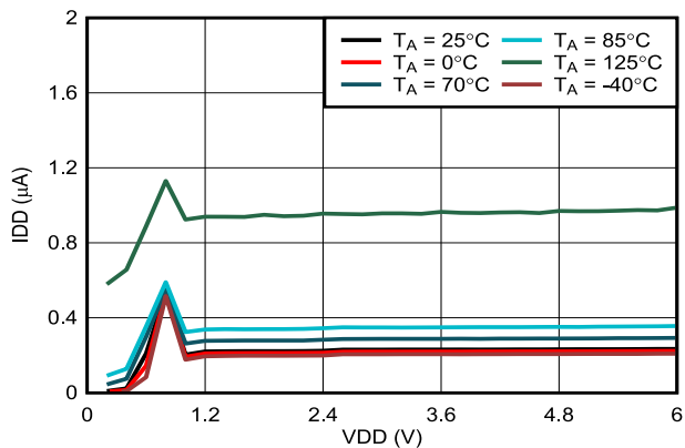
7-18. Supply Current vs Power-Supply Voltage
