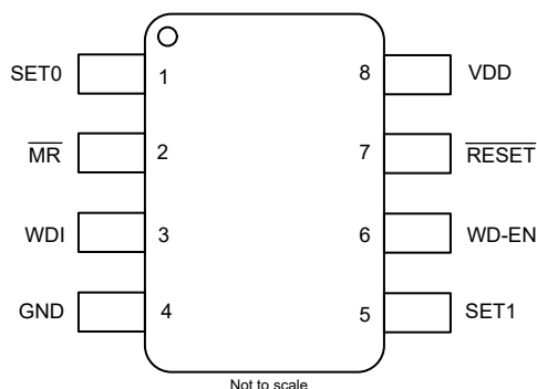
6-3. Pin Configuration Option C DDF Package, 8-Pin SOT-23, TPS36-Q1 Top View
