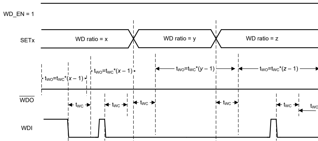
図 8-9. Watchdog Behavior with SETx Pin Status
