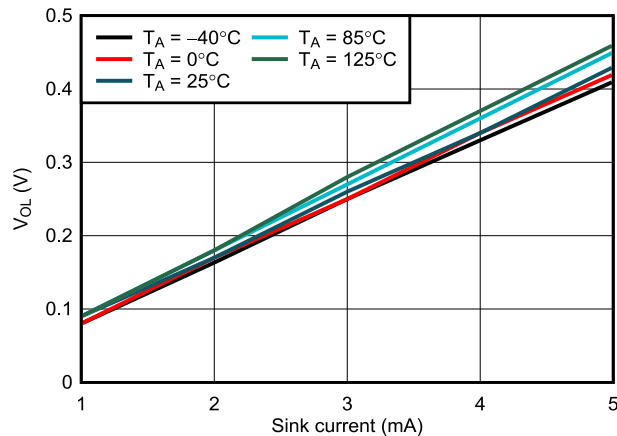
Figure 7-12. RESET V_{OL} vs I_{sink} , V_{DD} = 3.3\text{ V}
