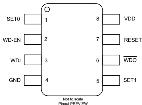
6-4. Pin Configuration Option D DDF Package, 8-Pin SOT-23, TPS36-Q1 Top View
