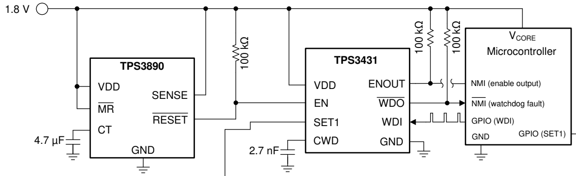
FIG 8-6. Monitoring the Supply Voltage and Watchdog Supervision of a Microcontroller
