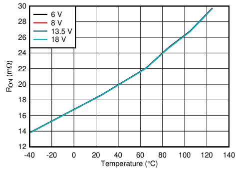
FIG 9. On Resistance ( R_{ON} ) vs Temperature
