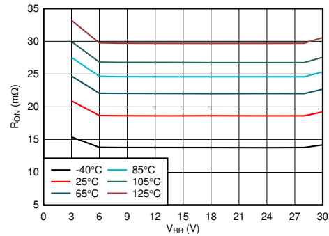
FIG 10. On Resistance ( R_{ON} ) vs V_{BB}
