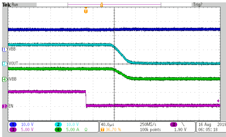
FIG 54. Turn-Off Waveform
