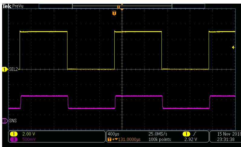
FIG 55. Toggling Between CH1 and CH2 Current Measurement
