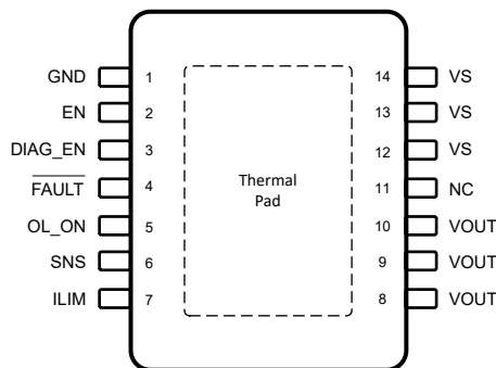
図 5-1. PWP Package, 14-Pin HTSSOP (Top View)
