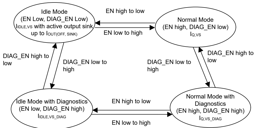
8-1. Work-Mode State Machine
