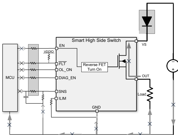
図 8-17. Reverse Protection With Blocking Diode
