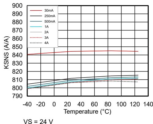
図 6-8. Current Sense Ratio ( KSNS ) vs Temperature vs Load Current
