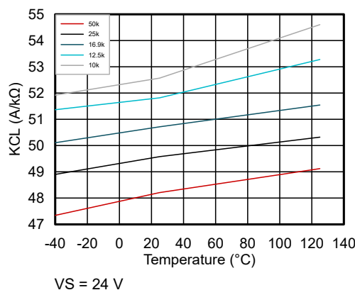
図 6-10. Current Limit Ratio ( K_{CL} ) vs Temperature vs R_{ILIM}
