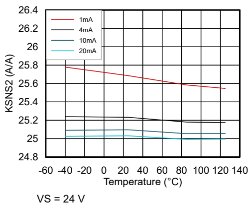
図 6-9. Current Sense Ratio ( KSNS_2 ) vs Temperature vs Load Current
