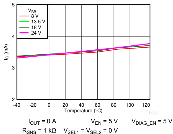
7-4. Quiescent Current ( I_Q ) vs Temperature
