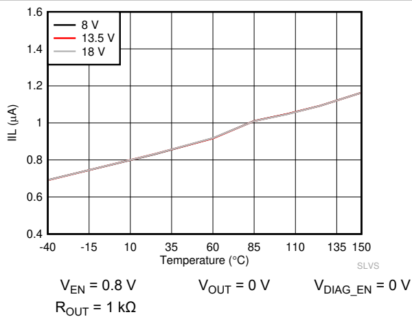
Figure 7-25. I_{IL} vs Temperature
