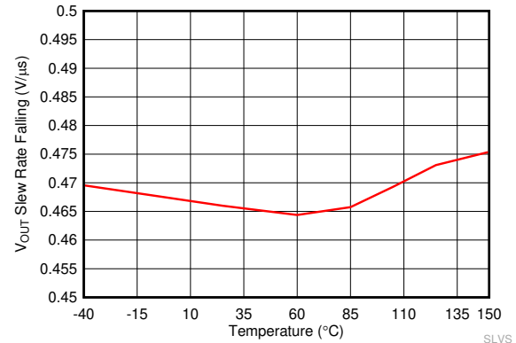
Figure 7-10. V_{OUT} Slew Rate Falling ( SR_F ) vs Temperature
