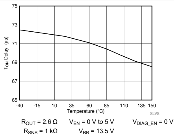
7-7. Turn-on Delay Time ( t_{DR} ) vs Temperature
