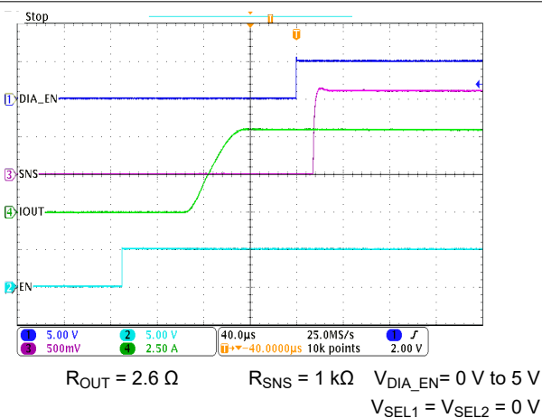
图 7-29. I_{SNS} Settling Time ( t_{SNSION1} ) on DIA_EN Transition
