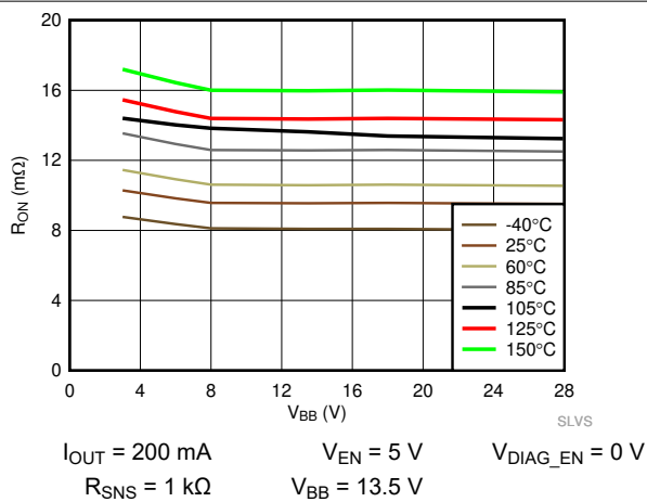
7-6. On Resistance ( R_{ON} ) vs V_{BB}
