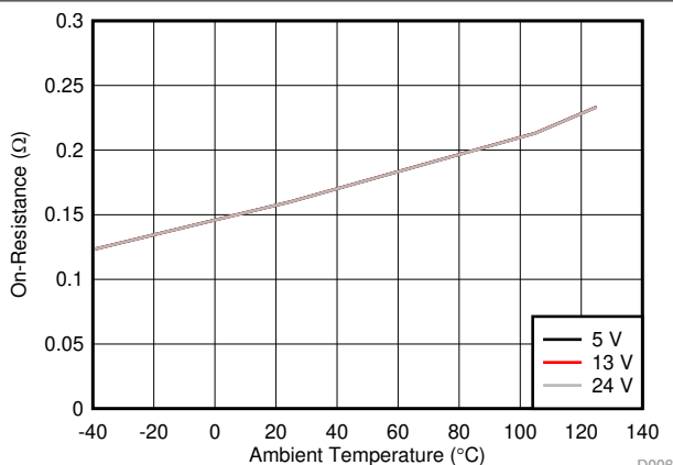
7-12. Channel-3 FET On-Resistance
