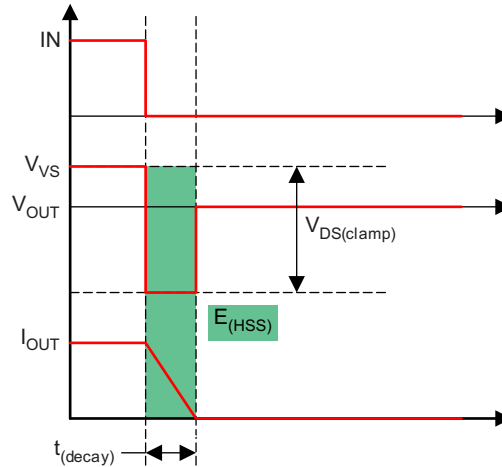
8-6. Inductive Load Switching-Off Diagram, note EN pin waveform referred to as IN
