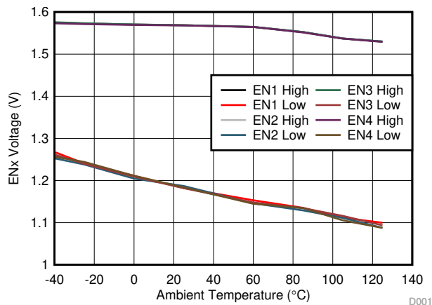
Figure 7-5. ENx Voltage Threshold
