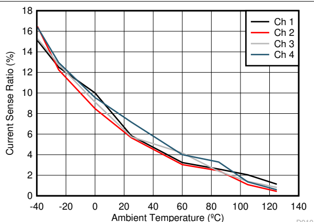
7-14. Current-Sense Ratio at 5 mA
