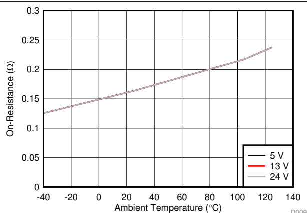
7-13. Channel-4 FET On-Resistance
