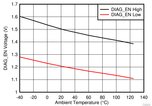
Figure 7-6. DIAG_EN Voltage Threshold
