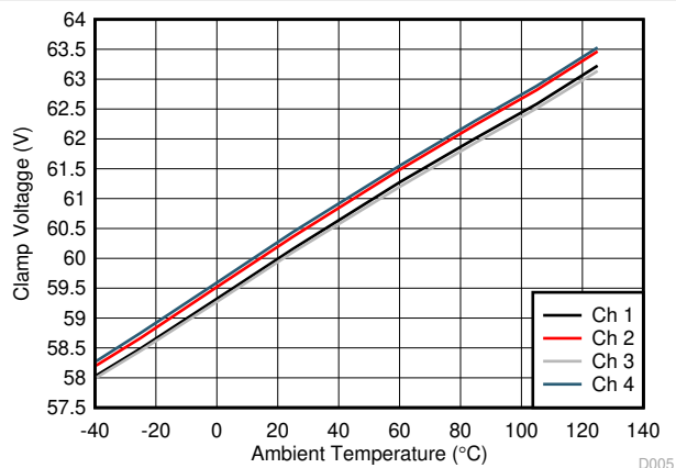
Figure 7-9. Drain-to-Source Clamp Voltage
