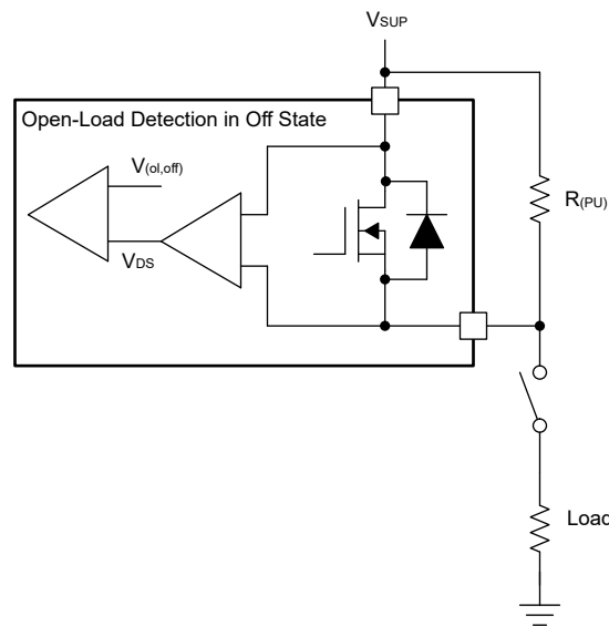
FIG 8-10. Open-Load Detection in Off-State
