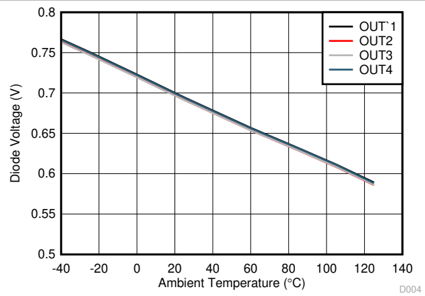
Figure 7-8. Body-Diode Forward Voltage
