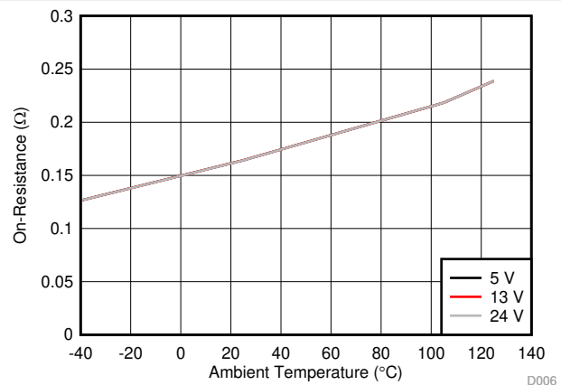
Figure 7-10. Channel-1 FET On-Resistance
