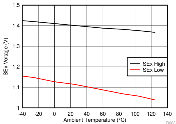
Figure 7-7. SEx Voltage Threshold
