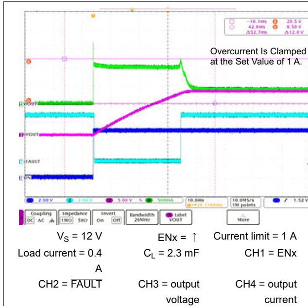
Figure 9-3. Driving a Capacitive Load With Adjustable Current Limit
