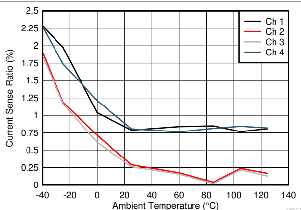
7-15. Current-Sense Ratio at 25 mA
