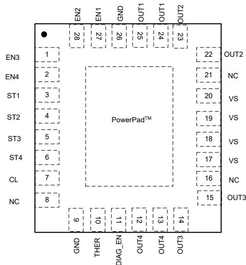
图 6-1. RLH Package 28-Pin WQFN With Exposed Thermal Pad TPS274160A Top View
