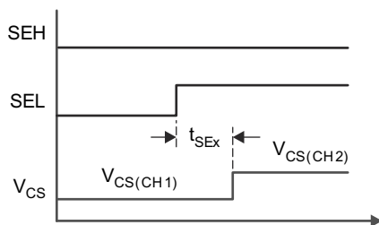
7-4. Multi-Sense Transition Delay
