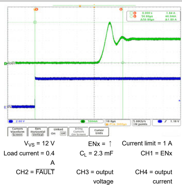
Figure 9-4. Driving a Capacitive Load, Expanded Waveform
