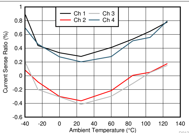
7-16. Current-Sense Ratio at 50 mA
