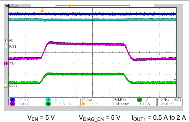
图 7-12. I_{SNS} Settling Time on Rising Load Step
