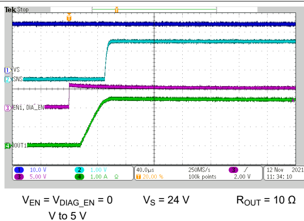
图 7-11. I_{SNS} Settling Time on DIA\_EN Transition
