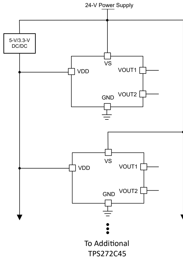
9-6. Secondary Low Voltage Supply Schematic
