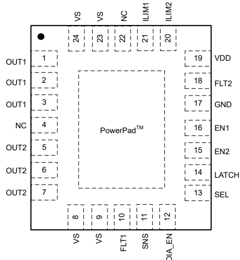
图 6-3. RHFP Package, 24-Pin QFN (Top View) Version D
