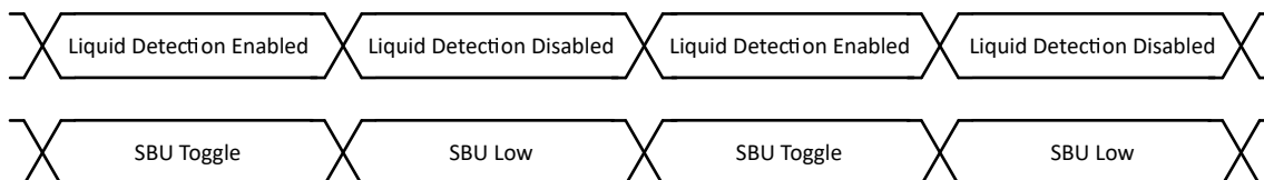
図 8-15. Liquid Detection and SBU1/2 Toggle
