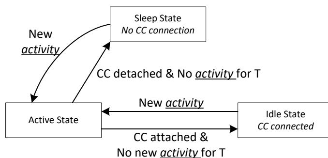
図 7-24. Flow Diagram for Power States
