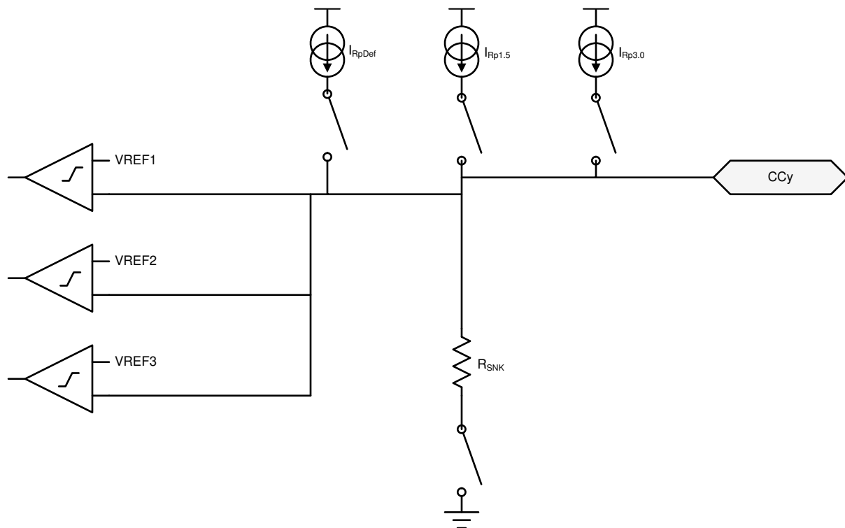
図 7-11. Plug and Orientation Detection Block
