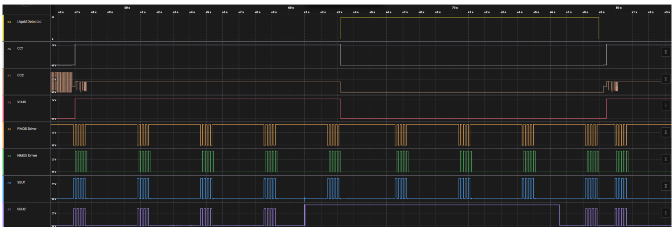
図 8-14. Liquid Detection Behavior - Corrosion Mitigation
