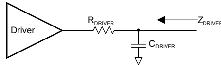
☒ 7-7. Z DRIVER Circuit
