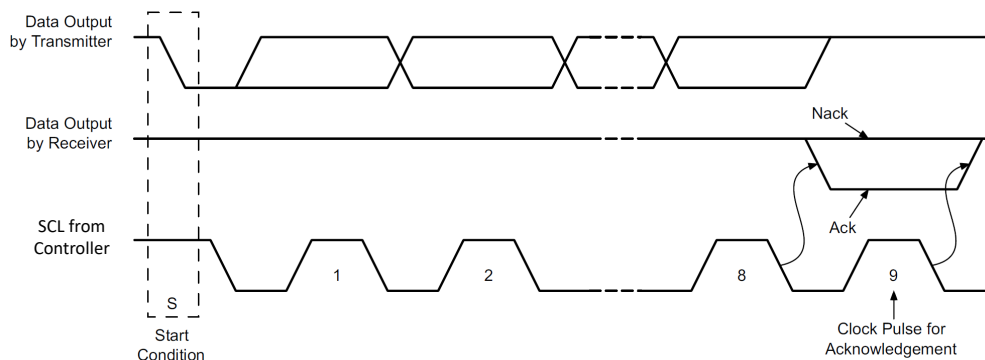
図 7-20. I²C Acknowledgment
