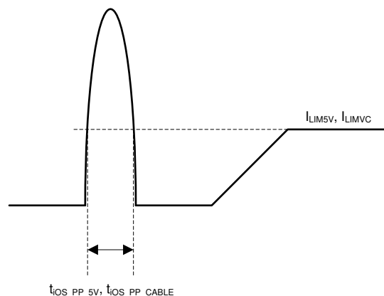
図 6-2. Short-circuit Response Time for Internal Power Paths PP_5V and PP_CABLE
