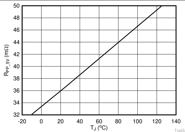
図 5-1. PP_5V Rdson vs Temperature
