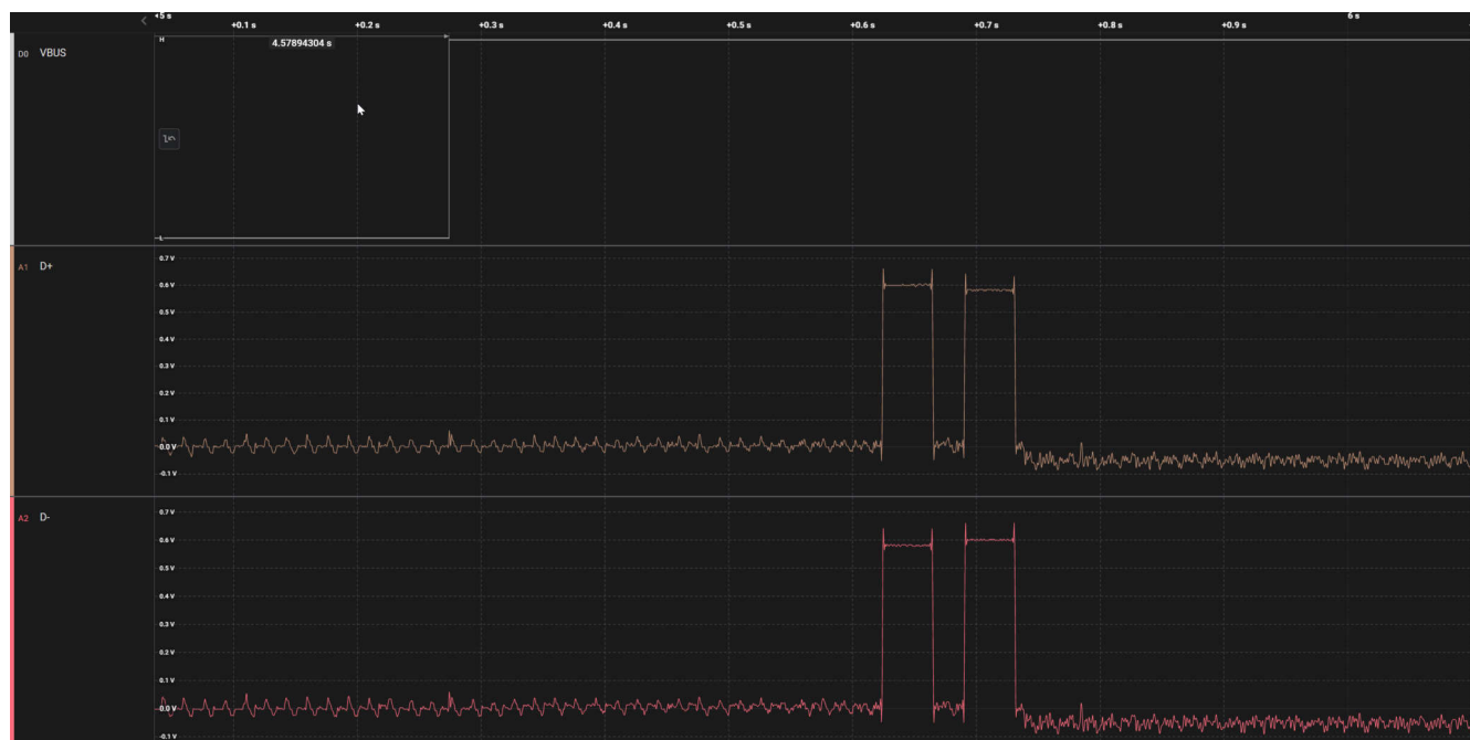
図 8-18. BC1.2 DCP Detection
