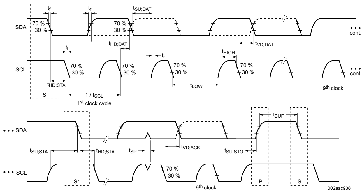
図 6-1. I 2 C Target Interface Timing
