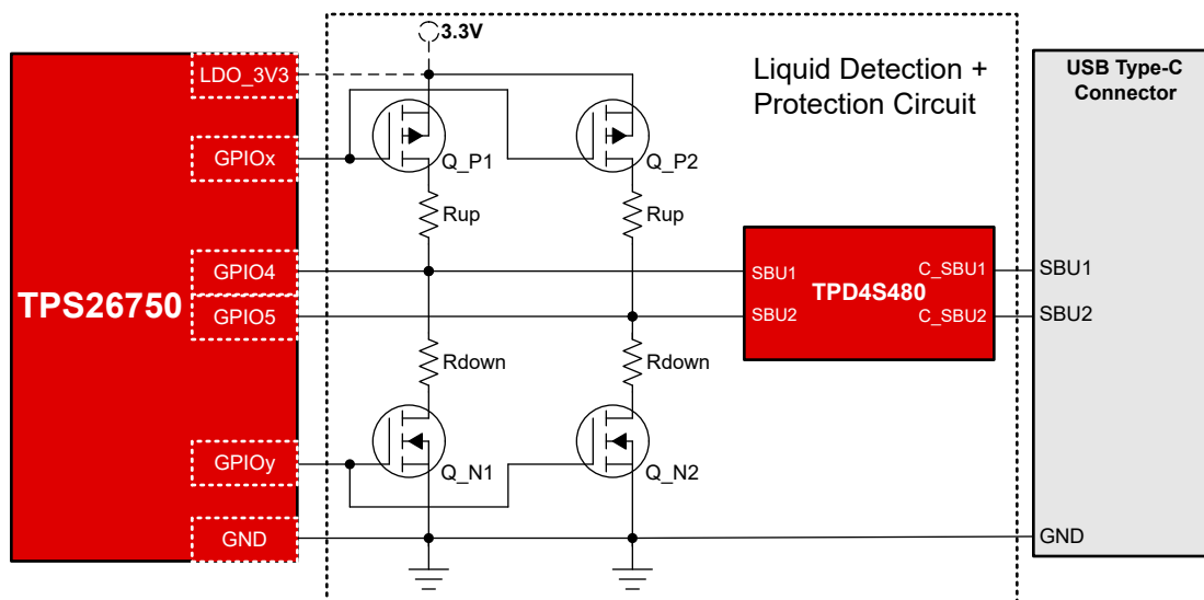
図 8-7. TPS26750 Liquid Detection Block Diagram - 2 GPIO Control
