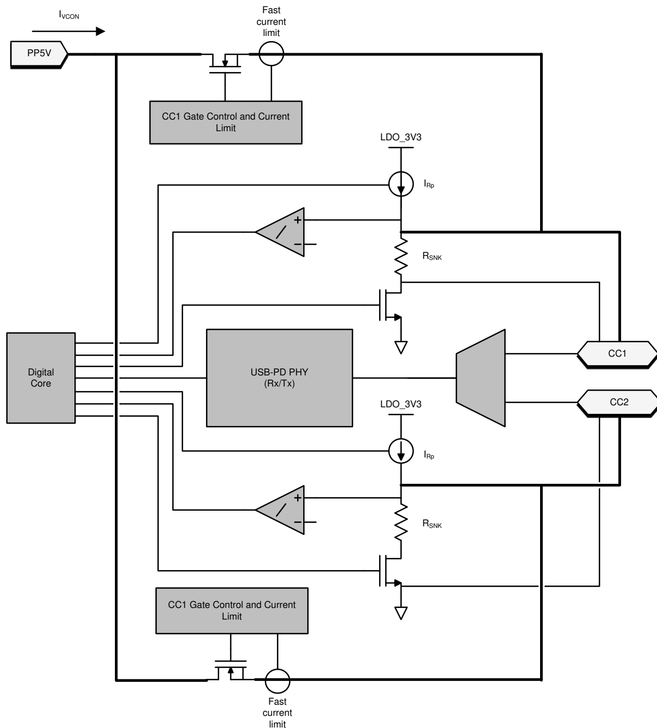
7-1. USB-PD Physical Layer and Simplified Plug and Orientation Detection Circuitry
