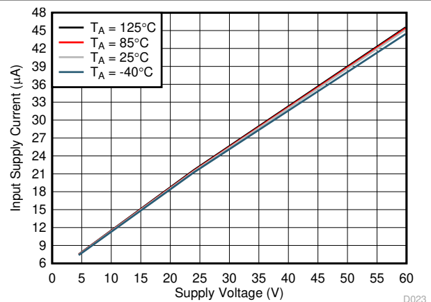
図 6-6. Input Supply Current vs Supply Voltage in Shutdown
