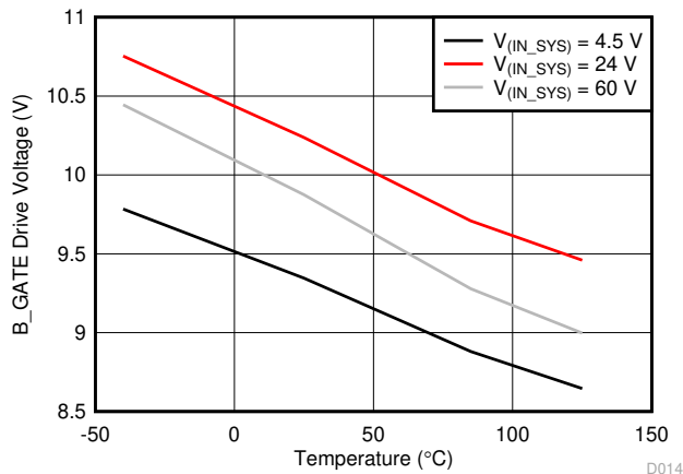
図 6-3. B_GATE Drive Voltage vs Temperature
