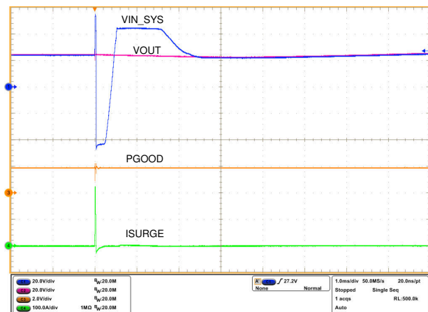
図 9-9. 500-V, 2-Ω Surge Response
