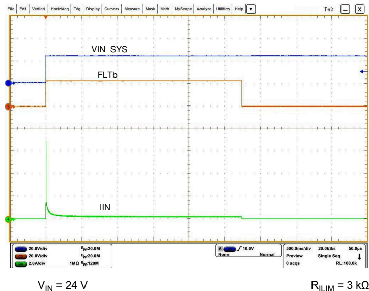
図 8-17. Start-Up With Short on Output
