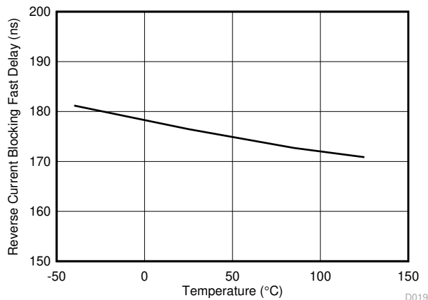
FIG 6-17. Reverse Current Blocking Response vs Temperature
