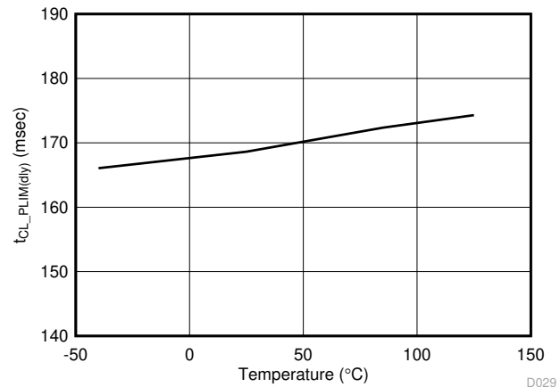
FIG 6-16. Maximum Duration in Current and Power Limiting vs Temperature
