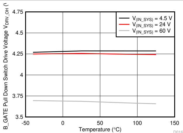
図 6-5. B_GATE Pulldown Drive Voltage vs Temperature
