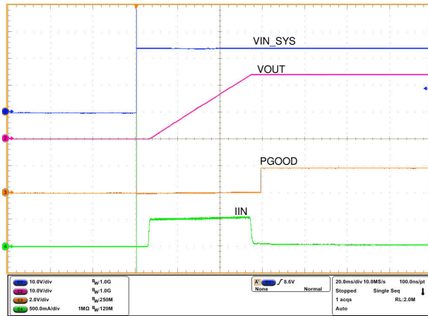
図 9-3. Hot Plug-In at 24-V Supply
