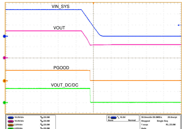
図 9-8. Power-Down Response
