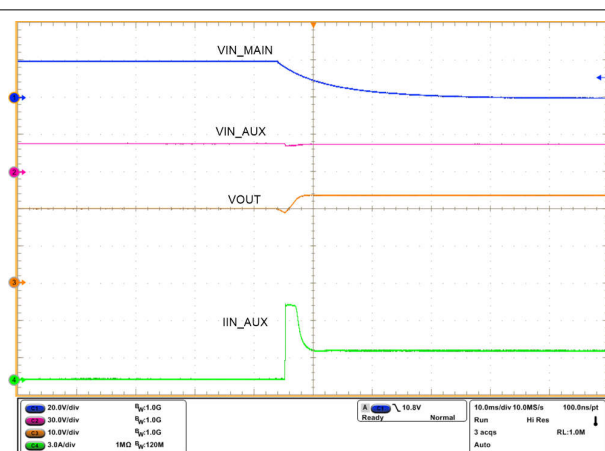
图 9-14. VIN_MAIN Brownout Condition: Change Over from Main VIN_MAIN to Auxiliary Power VIN_AUX
