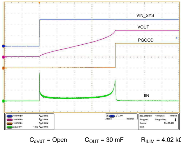
図 8-4. Thermal Regulation Loop Response During Power Up with Large Capacitive Load
