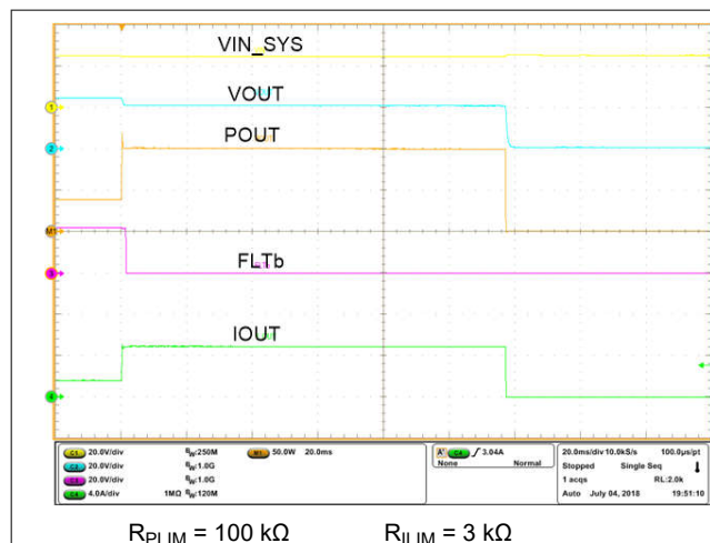
図 8-19. 100-W Class 2, Output Power Limiting Response of TPS26632
