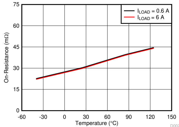
図 6-1. On-Resistance vs Temperature Across Load Current
