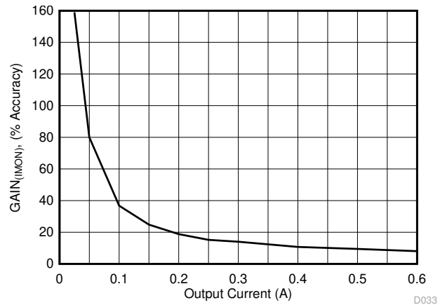
FIG 6-14. IMON Gain Accuracy at < 0.6-A Output Current
