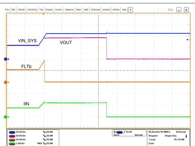
☒ 8-6. Overvoltage Clamp Response With TPS26635
