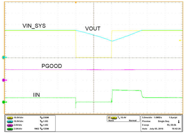
図 9-4. Voltage Interruption Response with TPS26630
