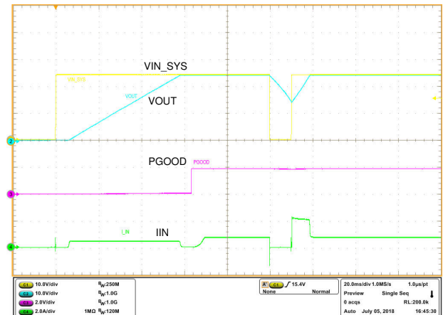
図 9-6. Power Up Followed with Voltage Interruption with TPS26630
