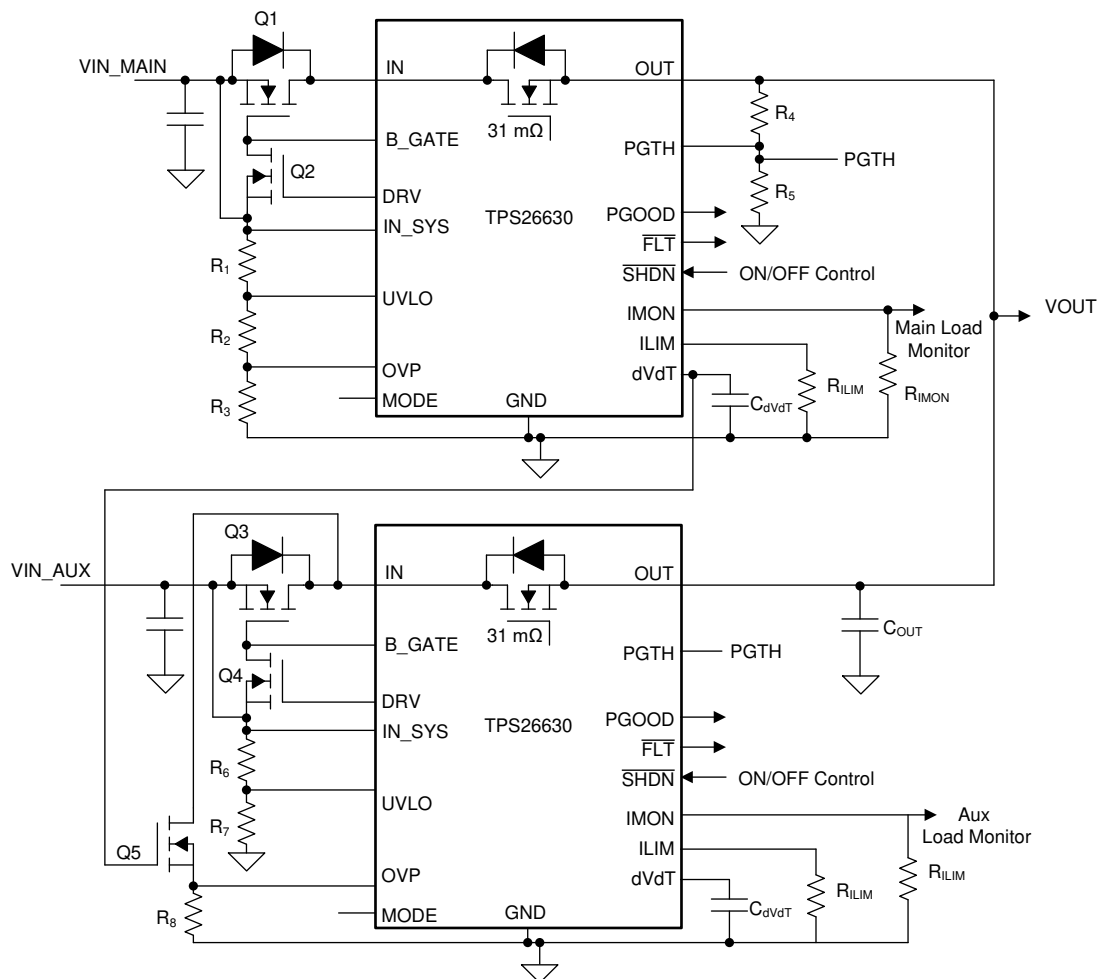
☒ 9-12. Priority Power Mux Implementation
