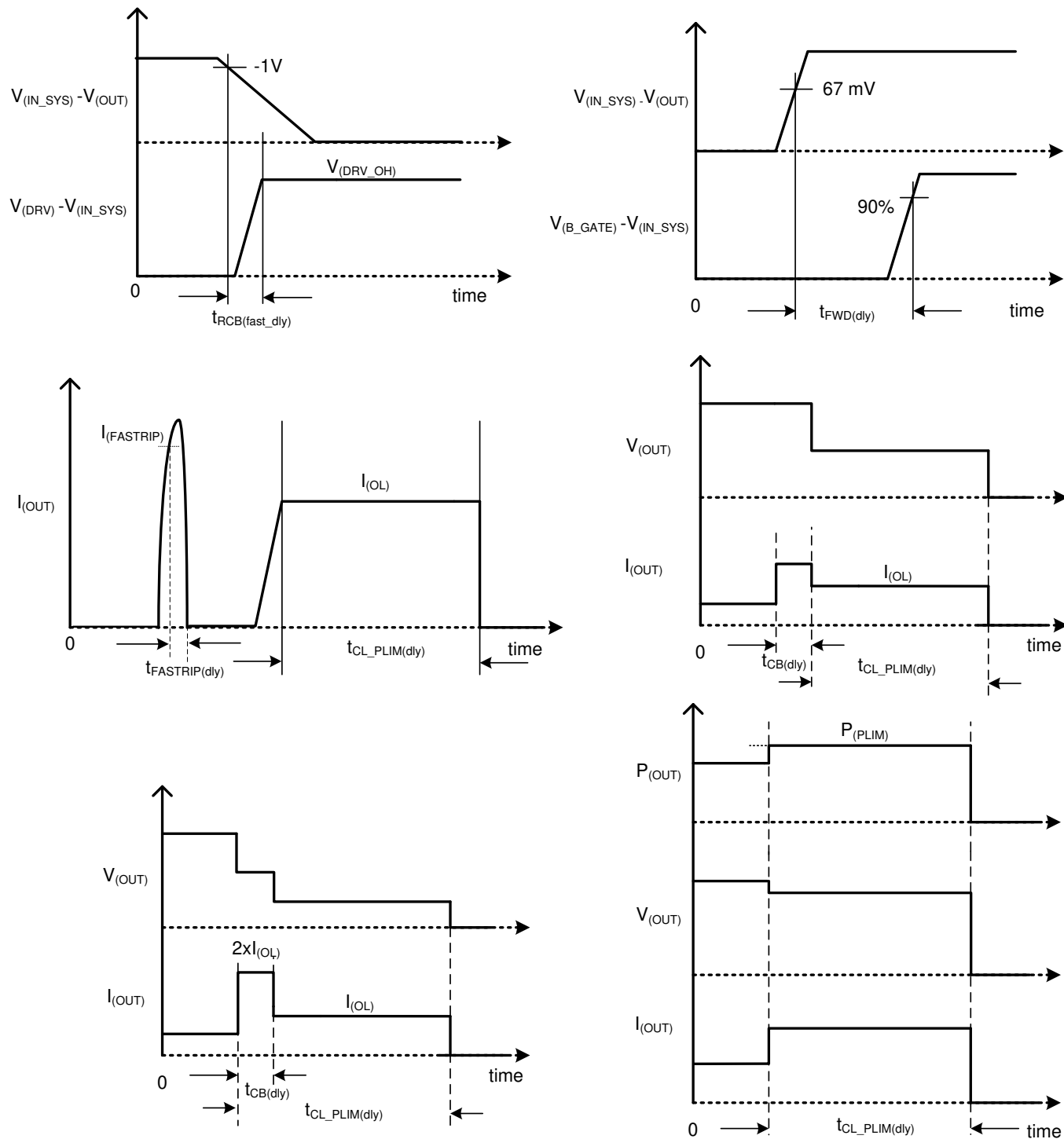
図 7-2. Timing Waveforms
