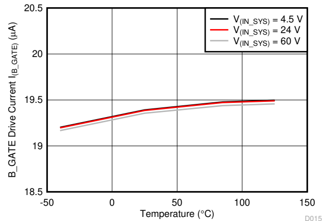
図 6-4. B_GATE Drive Current vs Temperature
