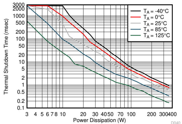
FIG 6-18. Thermal Shutdown Time vs Power Dissipation
