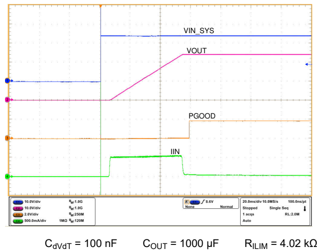
図 8-3. Hot Plug-In and Inrush Current Control at 24-V Input
