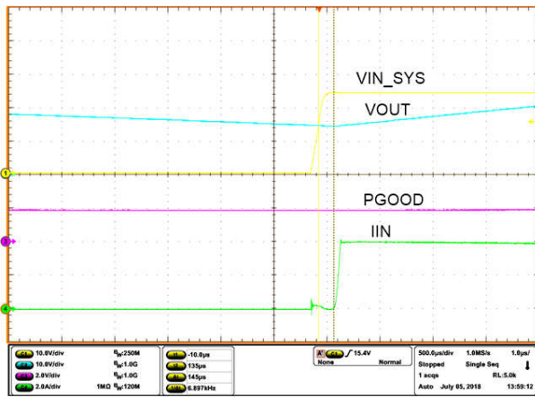
図 9-5. Voltage Interruption Response with TPS26630 (Zoomed)
