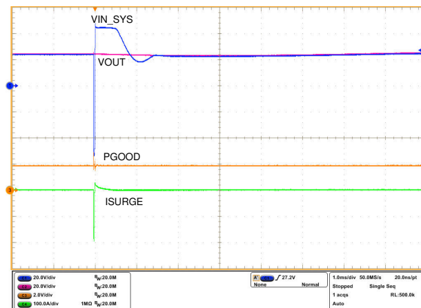
図 9-10. -500-V, 2-Ω Surge Response
