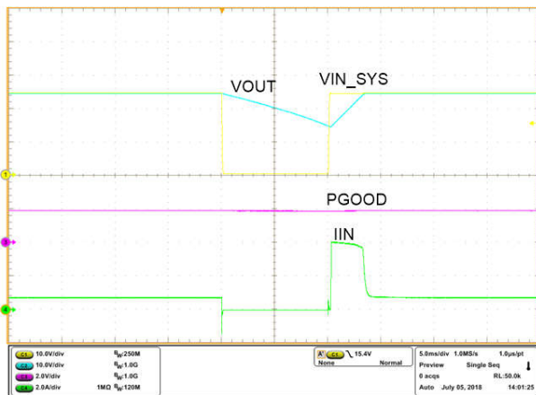
図 9-7. Voltage Interruption Performance with TPS26631
