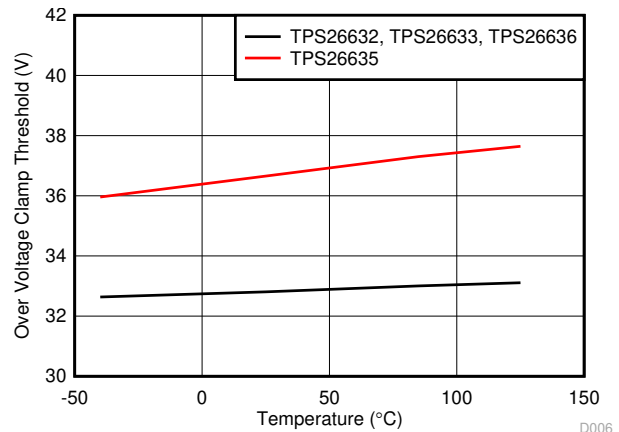
図 6-2. Overvoltage Clamp Threshold vs Temperature
