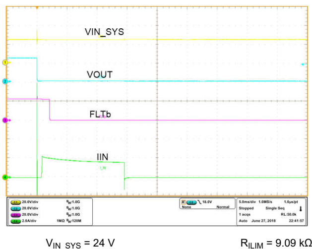
図 8-16. Output Hot-Short Response
