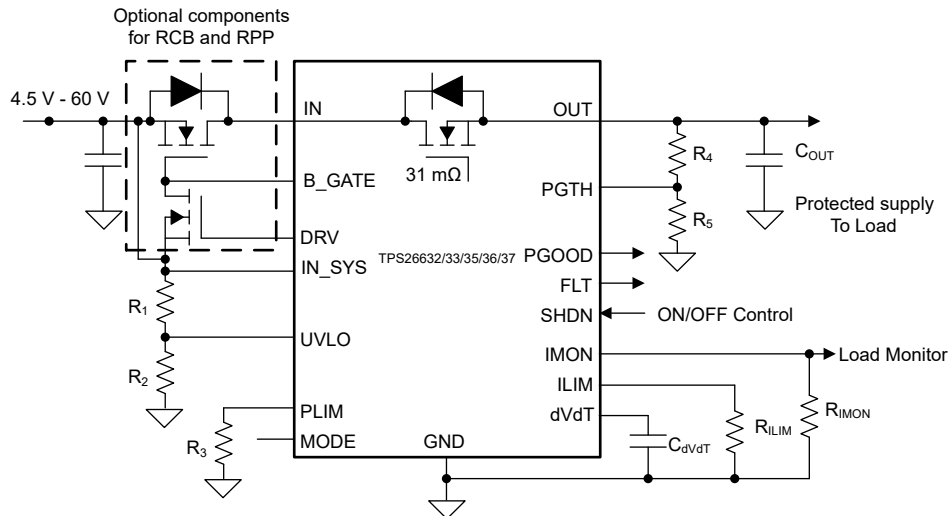
8-18. TPS26632, TPS26633, TPS26635, TPS26636, and TPS26637 Typical Application Schematic
