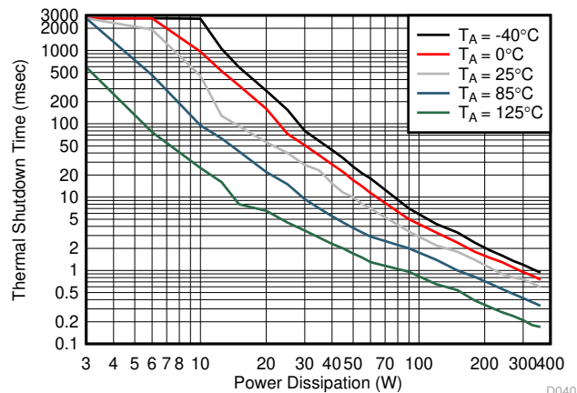
Figure 6-18. Thermal Shutdown Time vs Power Dissipation
