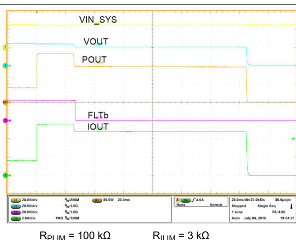
図 8-20. 100-W Class 2, Output Power Limiting Response of TPS26633
