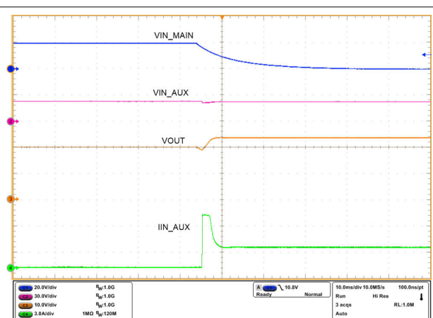
9-14. VIN_MAIN Brownout Condition: Change Over from Main VIN_MAIN to Auxiliary Power VIN_AUX
