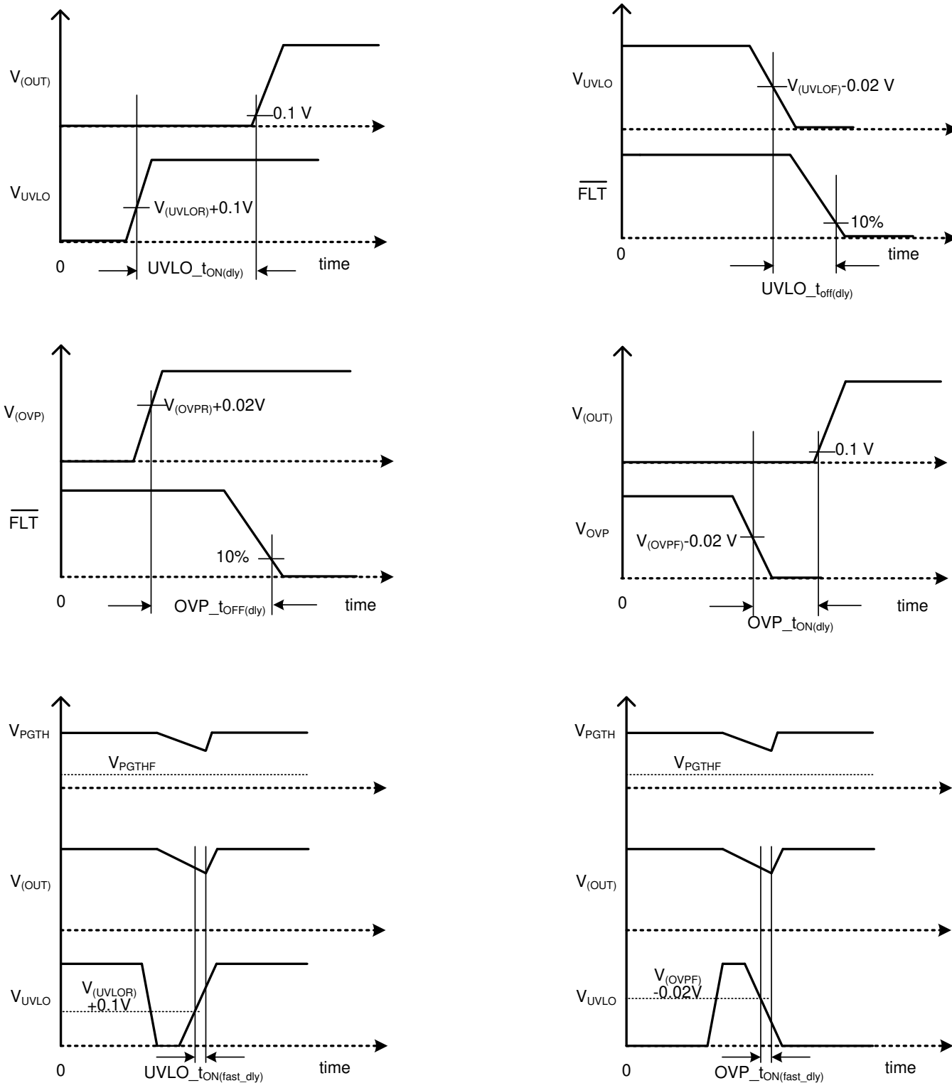
図 7-1. Timing Waveforms
