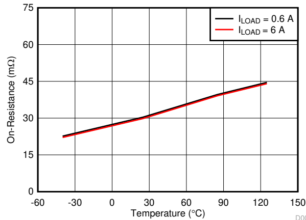
図 6-1. On-Resistance vs Temperature Across Load Current
