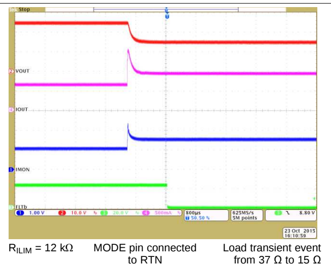
Figure 47. Output Turnoff Due to Thermal Shutdown With \overline{\text{FLT}} Asserted in Advance
