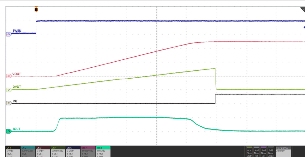
7-27. Inrush Current Control with Capacitive Load
