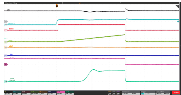
Figure 9-7. Power Up into Short: V_{IN} = 12 V, EN/UVLO Stepped Up From 0 V to 3 V, R_{REF} = 40.2 k \Omega , R_{LIM} on Each Device = 300 \Omega , and OUT Shorted to GND
