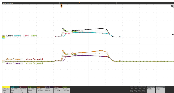
Figure 9-6. Start-up with EN/UVLO (Current distribution among five devices in parallel): V_{IN} = 12 V, EN/UVLO Stepped Up From 0 V to 3 V, C_{LOAD} = 55 mF, C_{DVRT} = 33 nF, R_{REF} = 40.2 k \Omega , and R_{LIM} on Each Device = 300 \Omega
