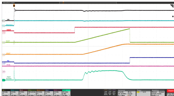
Figure 9-4. Input Hot Plug: V_{IN} Stepped Up from 0 V to 12 V, C_{LOAD} = 55 mF, C_{DVRT} = 33 nF, R_{REF} = 40.2 k \Omega , and R_{LIM} on Each Device = 300 \Omega
