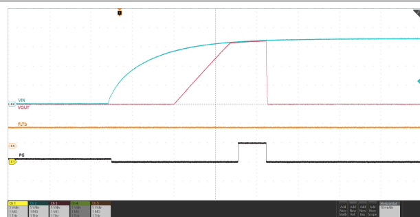
7-29. Input Overvoltage Protection Response
