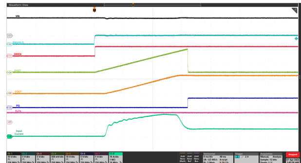
Figure 9-5. Start-up with EN/UVLO: V_{IN} = 12 V, EN/UVLO Stepped Up From 0 V to 3 V, C_{LOAD} = 55 mF, R_{LOAD(Start-up)} = 0.33 \Omega , C_{DVRT} = 33 nF, R_{REF} = 40.2 k \Omega , and R_{LIM} on Each Device = 300 \Omega
