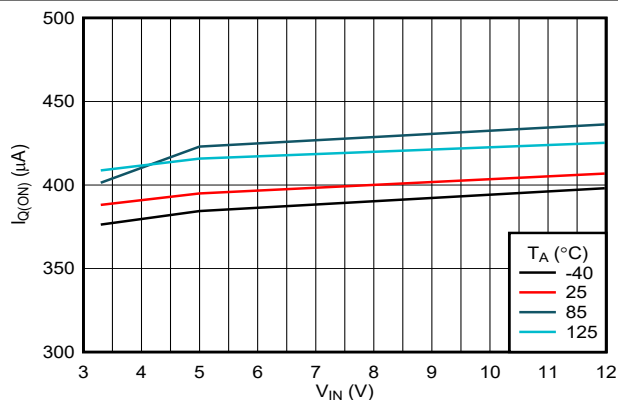
図 6-3. IN Quiescent Current vs Temperature (TPS25972x Variant)
