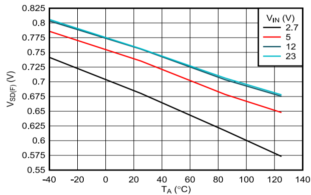
図 6-9. EN/UVLO Shutdown Falling Threshold vs Temperature
