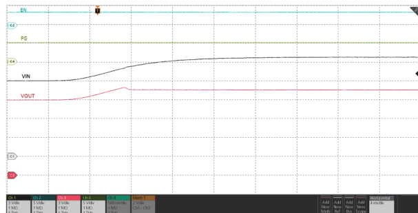
図 6-37. Overvoltage Clamp Response – TPS25972x
