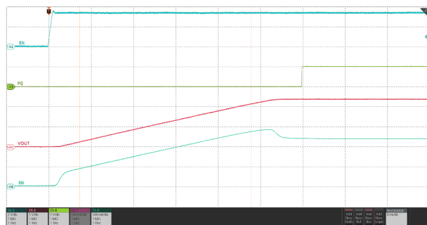
図 6-33. Inrush Current Without Slew Rate Control – Capacitive Load
