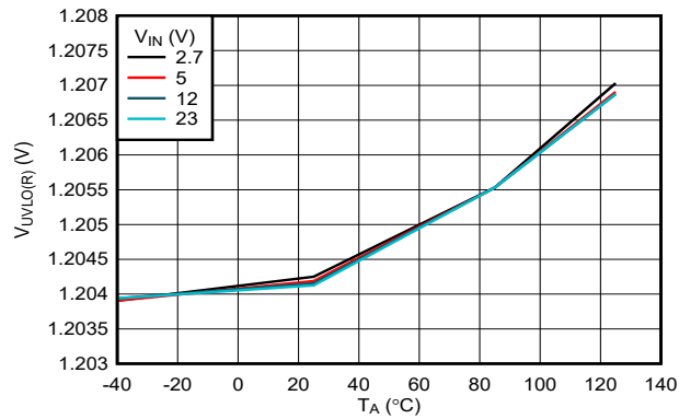
図 6-7. EN/UVLO Rising Threshold vs Temperature
