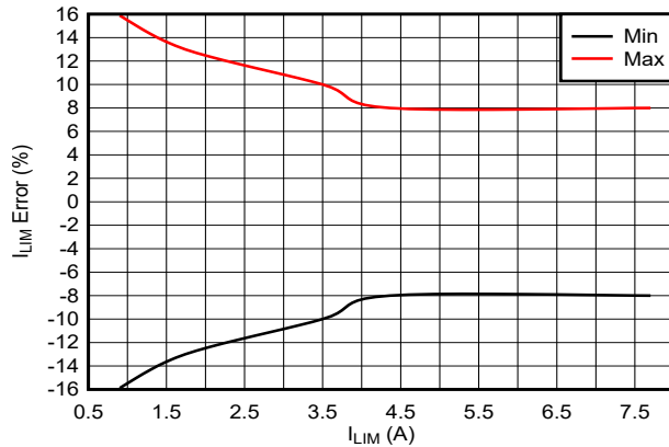
FIG 6-13. Overcurrent Threshold Accuracy (Across Process, Voltage and Temperature)
