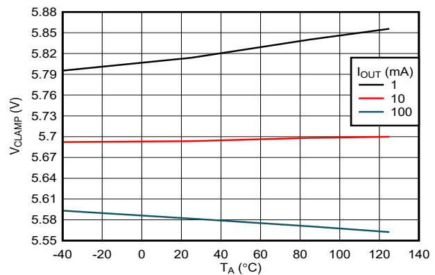
FIG 6-18. OVC Clamping Voltage (OVCSEL = OPEN) vs Load Current (TPS25972x Variant)
