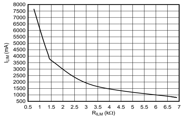
図 6-12. Overcurrent Threshold vs ILM Resistor
