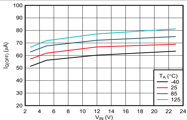
図 6-4. IN OFF State (UVLO) Current vs Temperature
