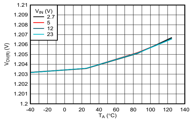
図 6-10. OVLO Rising Threshold vs Temperature (TPS25970x, TPS25974x Variants)
