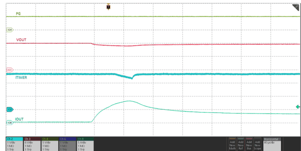
図 6-40. Active Current Limit Response – TPS25970x
