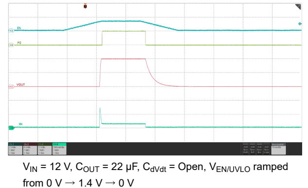
FIG 6-30. Power Up and Down With EN/UVLO Control
