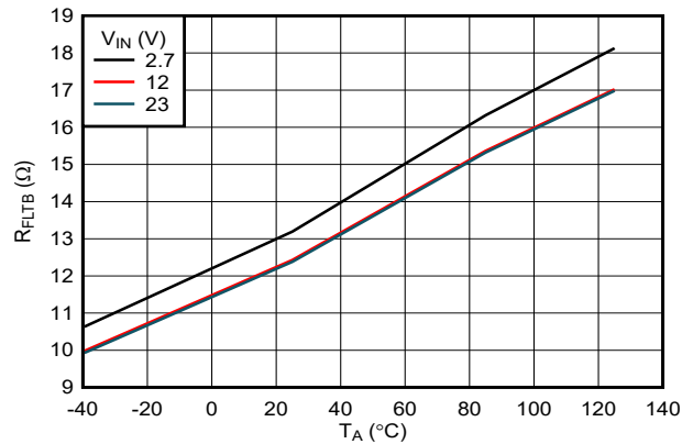
FIG 6-27. FLT Pin Pulldown Resistance vs Temperature
