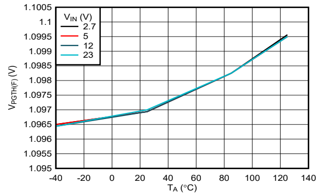
FIG 6-26. PGTH Threshold (Falling) vs Temperature (TPS25972x, TPS25974x Variants)
