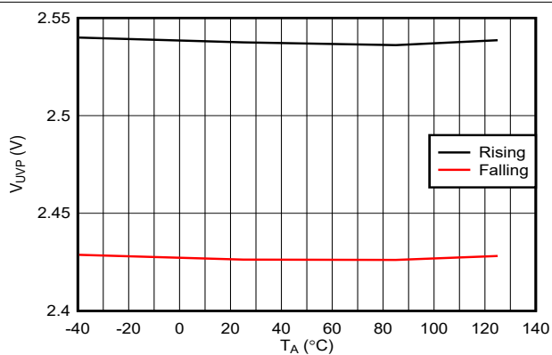
図 6-6. IN Undervoltage Threshold vs Temperature
