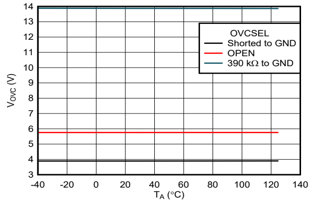
FIG 6-16. OVC Threshold vs Temperature (TPS25972x Variant)
