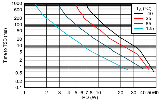
FIG 6-29. Time to Thermal Shut-Down During Steady State
