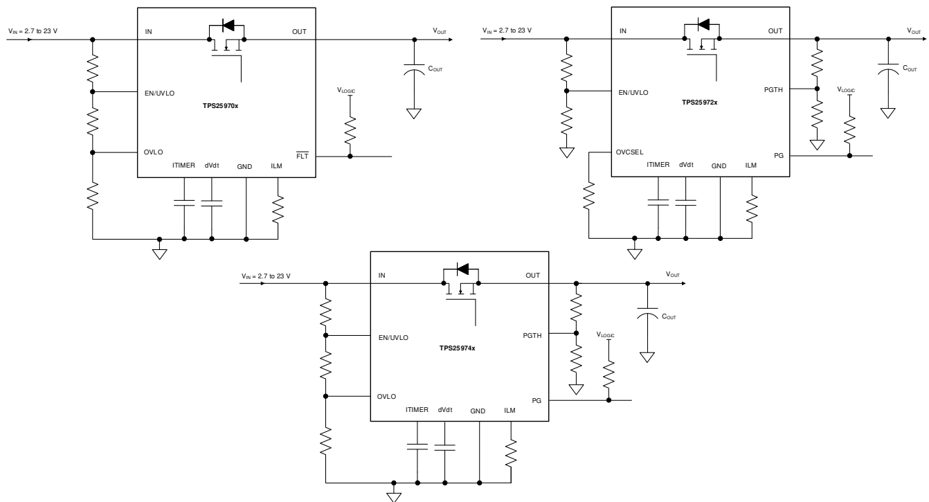
図 8-1. Single Device, Self-Controlled
