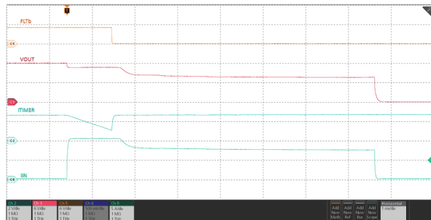
図 6-39. Overvoltage Clamp Response – TPS25972x
