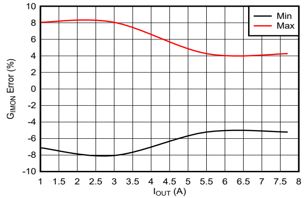
FIG 6-14. Analog Current Monitor Gain Accuracy
