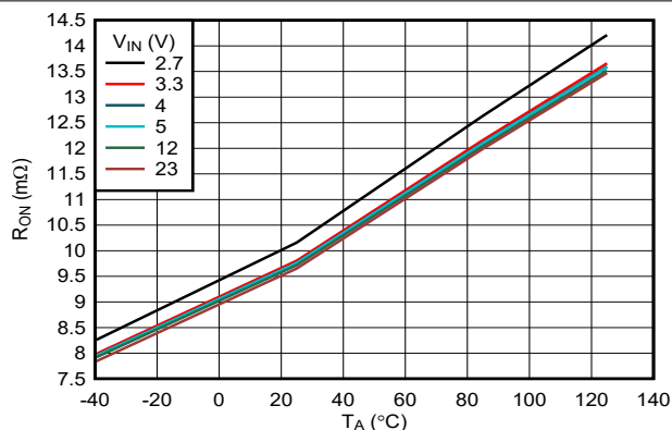
図 6-1. ON-Resistance vs Supply Voltage
