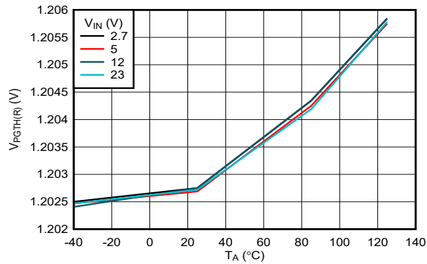
FIG 6-25. PGTH Threshold (Rising) vs Temperature (TPS25972x, TPS25974x Variants)
