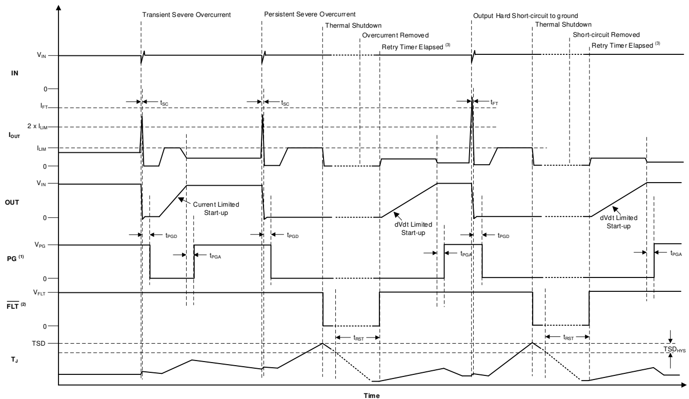
7-11. TPS2597xx Short-Circuit Response
