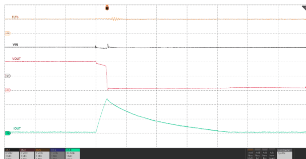
図 6-43. Circuit-Breaker Response TPS25974x
