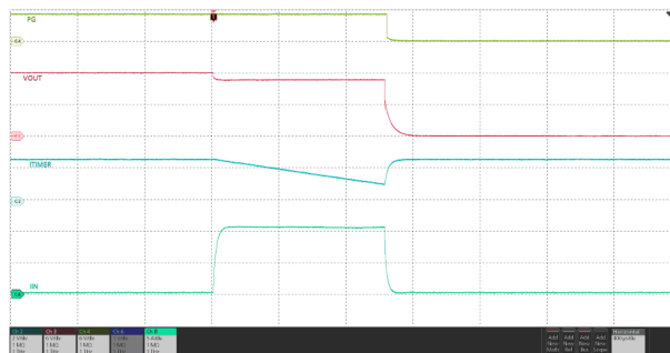
✎ 8-6. Circuit Breaker Response
