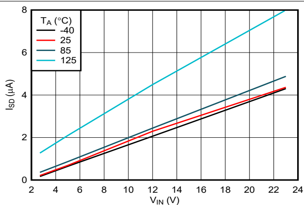
図 6-5. IN Shutdown Current vs Temperature
