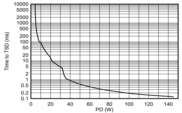
FIG 6-28. Time to Thermal Shut-Down During Inrush State
