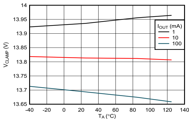
FIG 6-17. OVC Clamping Voltage (OVCSEL = 390 kΩ to GND) vs Load Current (TPS25972x Variant)
