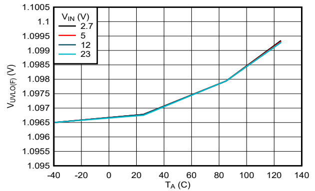
図 6-8. EN/UVLO Falling Threshold vs Temperature
