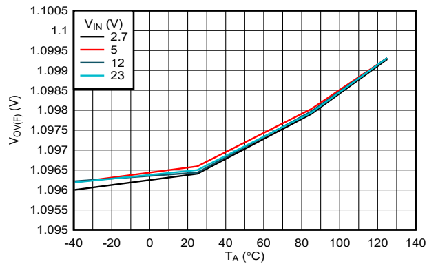
図 6-11. OVLO Falling Threshold vs Temperature (TPS25970x, TPS25974x Variants)
