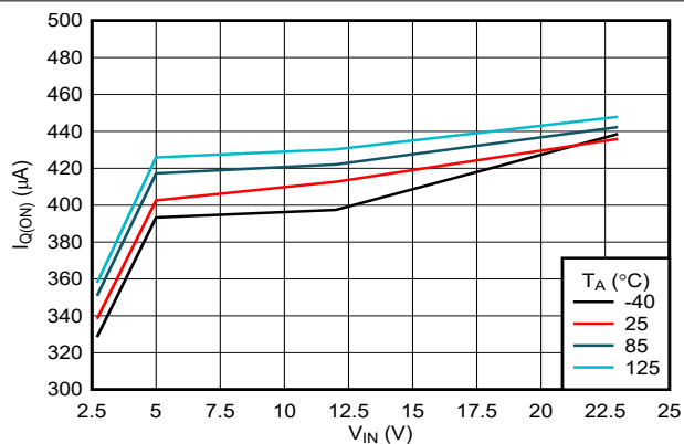
図 6-2. IN Quiescent Current vs Temperature (TPS25970x, TPS25974x Variants)
