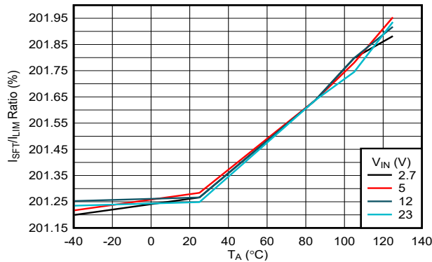
FIG 6-15. Scalable Fast-Trip Threshold: Current Limit Threshold ( I_{LIM} ) Ratio vs Temperature
