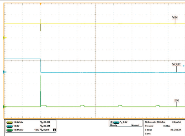
FIG 32. TPS2595x1, TPS2595x3, TPS2595x5 OverCurrent Response
