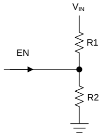
✎ 47. Undervoltage Lockout
