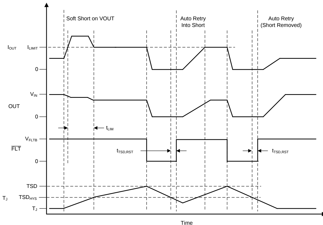
図 50. TPS2595x1, TPS2595x3, TPS2595x5 Overcurrent Response (Auto-Retry)
