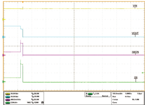
FIG 33. TPS2595x0 Overcurrent Response
