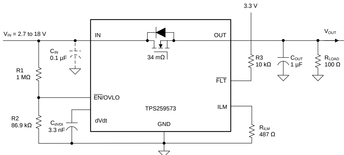
65. Circuit Implementation for Overvoltage Lockout using TPS259573
