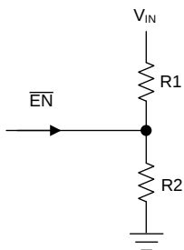
✎ 48. Overvoltage Lockout
