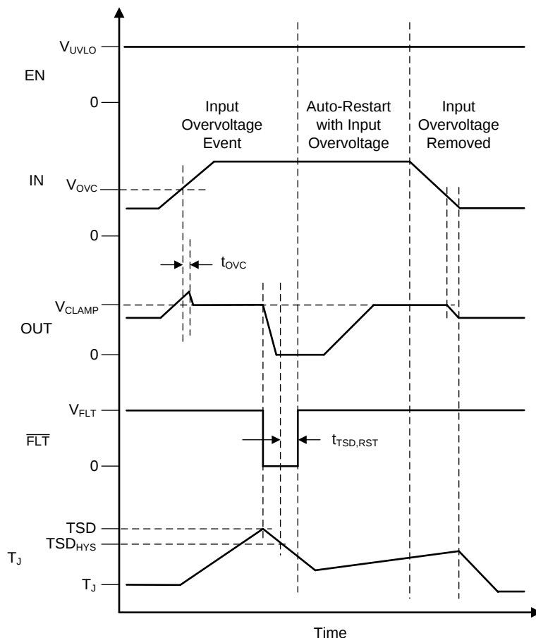
✶ 49. TPS2595xx Overvoltage Clamp Response (Auto-Retry)
