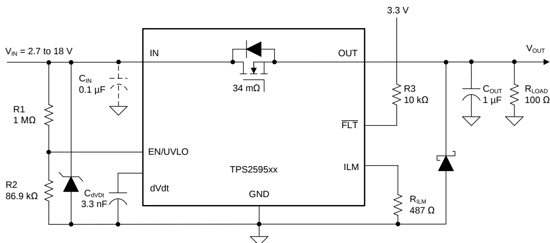
図 67. Circuit Implementation with Optional Protection Components
