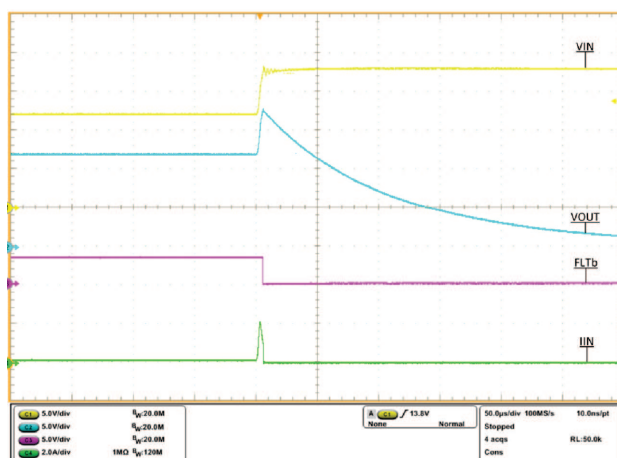
☒ 66. Overvoltage Lockout Response using TPS259573
