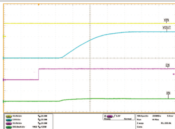
FIG 28. Output Voltage Ramp and Inrush Current at Start Up, C_{dvdt} = \text{Open}
