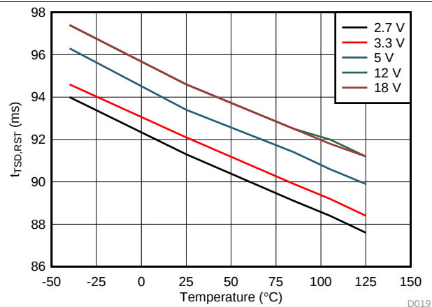
FIG 27. Thermal Shutdown Auto-Retry Interval vs Temperature
