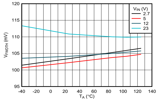
7-21. RCB - Forward Comparator Threshold vs Temperature
