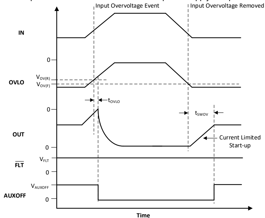
FIG 8-6. TPS259470x Overvoltage Lockout and Recovery
