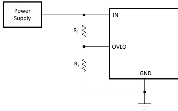
FIG 8-5. Adjustable Overvoltage Protection
