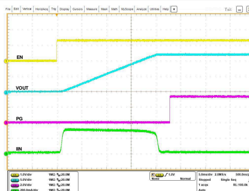
Figure 7-39. Start-Up with Supply
