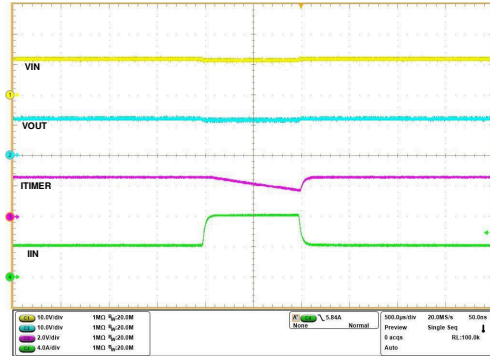
7-51. Transient Overcurrent Blanking Timer Response - TPS259474x
