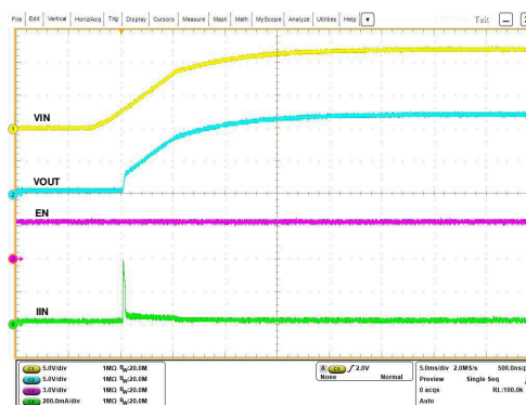
Figure 7-39. Start-Up with Supply
