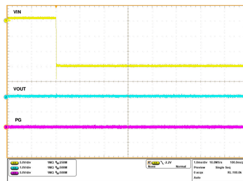
7-43. Input Reverse Polarity Protection - Fast Ramp
