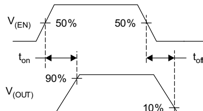
FIG 9-4. Enable Timing, Active-High Enable
