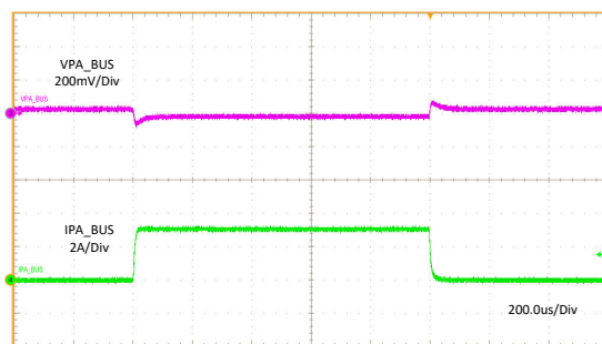
11-5. Load Regulation
