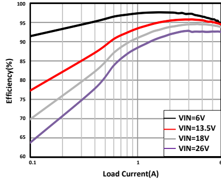
11-2. Buck Only Efficiency
