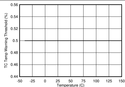
8-24. TS Temperature Wam Threshold vs Junction Temperature
