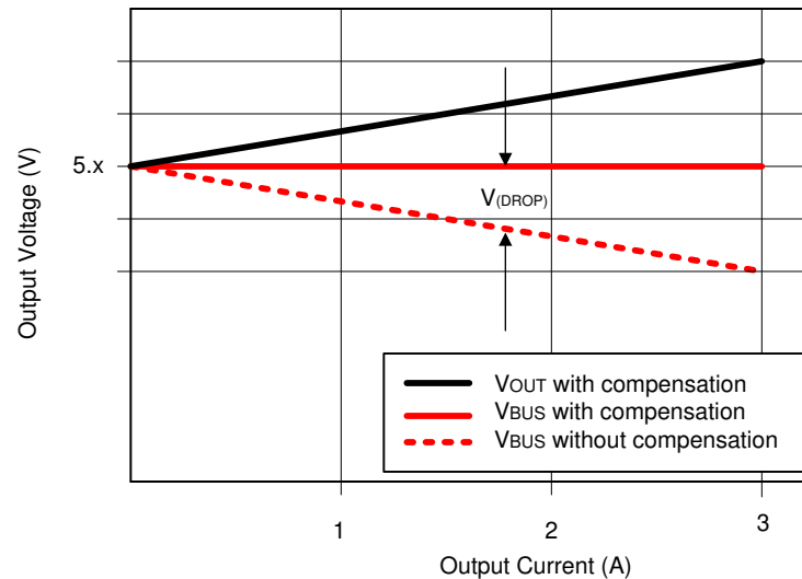
FIG 10-14. Voltage Drop
