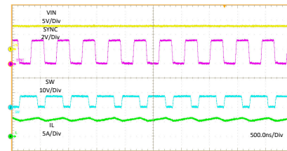
10-6. Switching Frequency When R_{FREQ} = 8.45 \text{ k}\Omega
