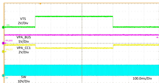
11-30. Thermal Sensing - NTC Temperature WARM Behavior
