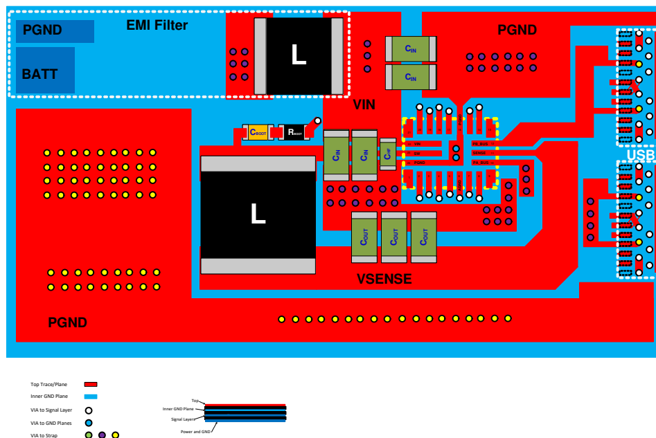
13-1. Layout Example
