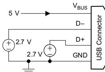
Figure 10-22. Divider 3 Mode
