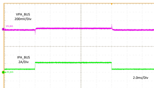
11-9. Load Transient Without Cable Compensation
