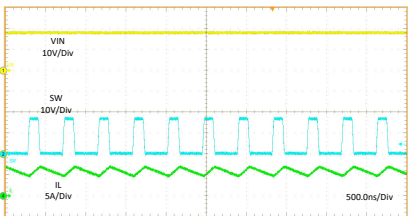
10-5. Switching Frequency When R_{FREQ} = 8.45 \text{ k}\Omega
