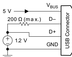
Figure 10-23. 1.2-V Mode
