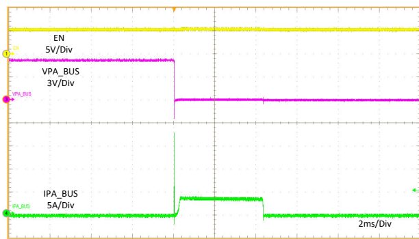
11-26. VBUS Hot Short to GND
