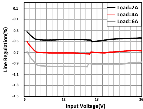
11-6. Line Regulation
