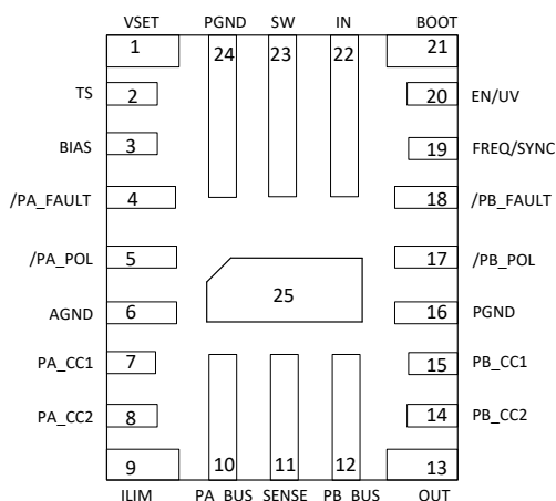
7-2. TPS25851-Q1 RPQ Package 25-Pin (QFN) Top View
