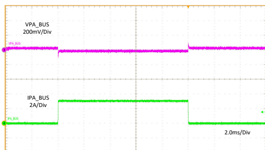
11-8. Load Transient Without Cable Compensation
