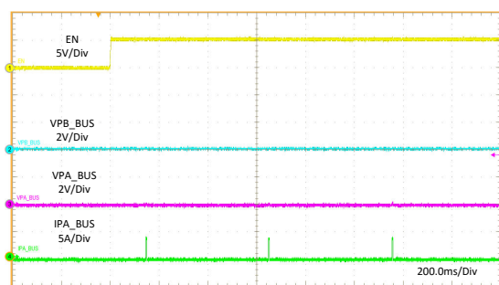
Figure 11-20. Rd Assert
