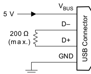
Figure 10-21. DCP Supporting BC1.2 and YD/T 1591-2009
