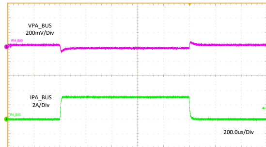
11-5. Load Regulation
