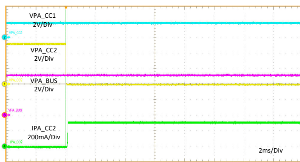
11-27. PA_CC2 Hot Short to GND
