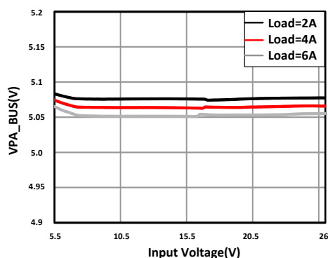
11-12. Dropout Characteristic
