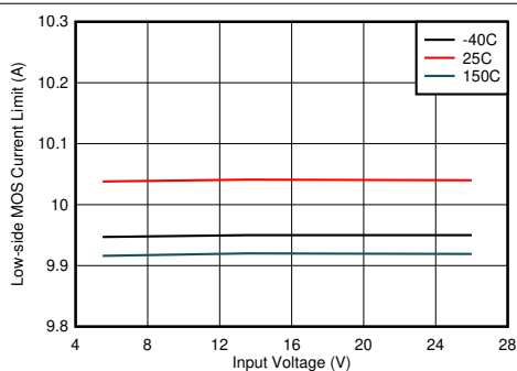
8-9. Low-side Current Limit vs Input Voltage
