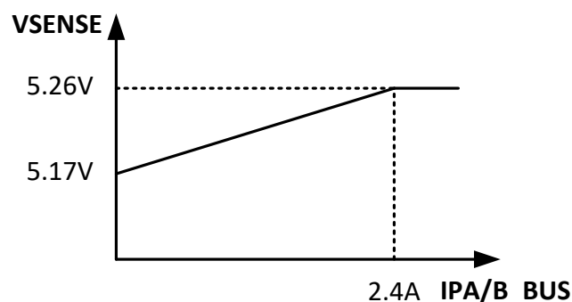
FIG 10-15. Dual Ports Cable Compensation
