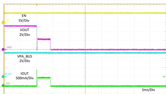
11-28. OUT short to 5.1- \Omega Load
