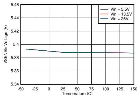
FIG 8-6. V_{SENSE} Voltage vs Junction Temperature
