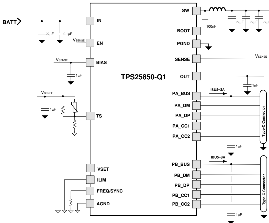
図 11-1. TPS25850-Q1 Typical Application Circuit for 2.1-MHz f_{sw}
