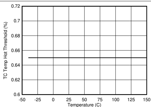
8-25. TS Temperature Hot Threshold vs Junction Temperature
