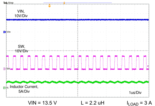
Figure 10-8. Switching Frequency when R_T = 8.87\text{ k}\Omega
