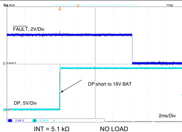
Figure 11-30. DP Short to BAT
