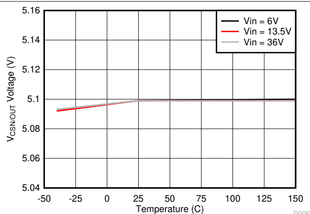
Figure 8-6. V_{CSN/OUT} Voltage vs Junction Temperature
