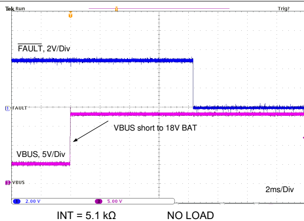
Figure 11-28. VBUS Short to BAT With External FET
