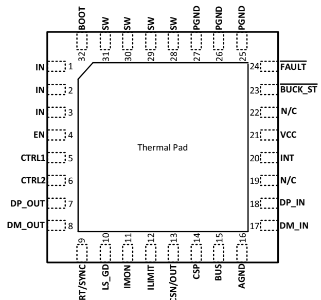
Figure 7-2. TPS25846QCWRHBRQ1 Package 32-Pin (VQFN) Top View (2)
