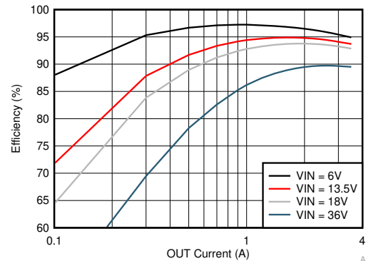
Buck Efficiency vs Output Current fsw = 400 kHz
