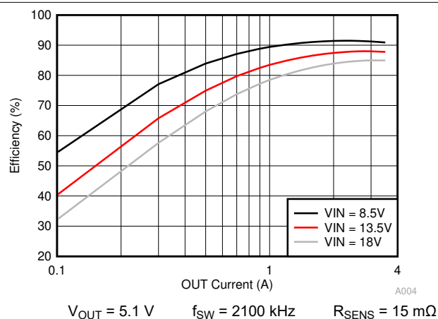
Figure 11-5. Efficiency With Sense Resistor
