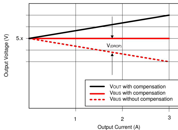
Figure 10-23. Voltage Drop
