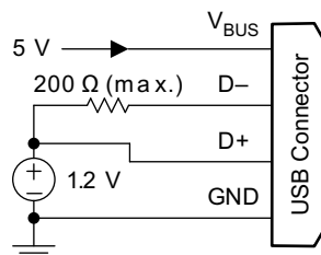
FIGURE 10-34. 1.2-V Mode
