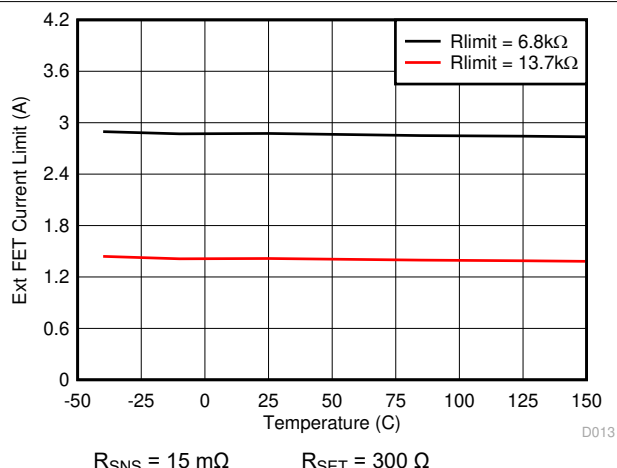
8-14. External FET Current Limit vs Junction Temperature
