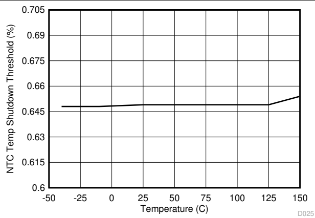
8-28. NTC Temperature Shutdown Threshold (TPS25833-Q1)
