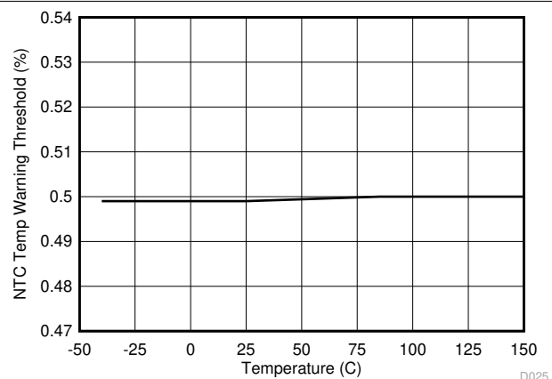
8-27. NTC Temperature Warning Threshold (TPS25833-Q1)
