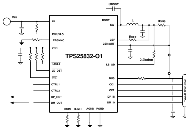
10-18. TPS25832-Q1 Buck Average Current Limit
