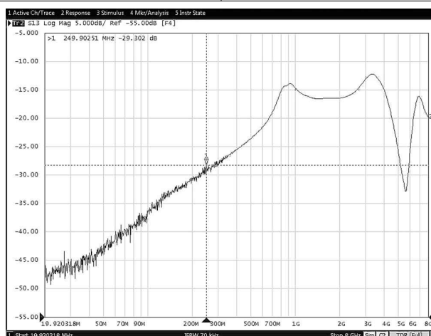
8-33. On-State Cross-Channel Isolation vs Frequency (TPS25832-Q1)
