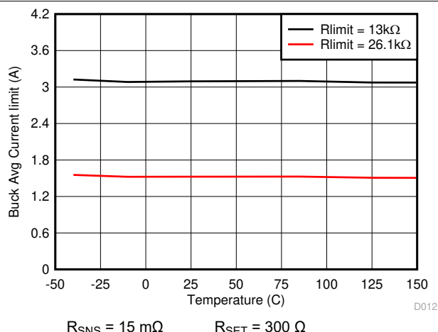
8-13. Buck Average Current Limit vs Junction Temperature
