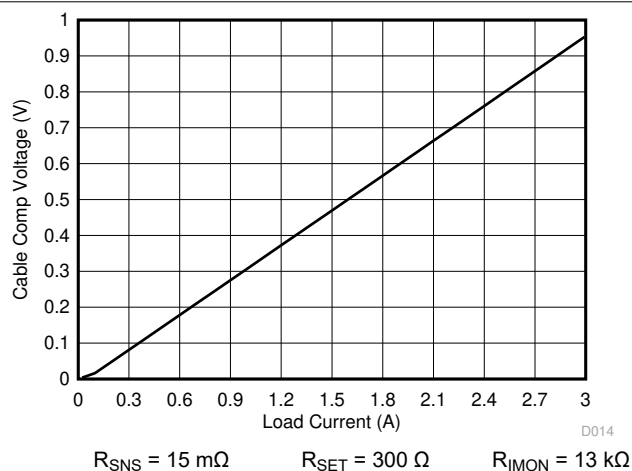
8-18. Cable Compensation Voltage vs Load Current
