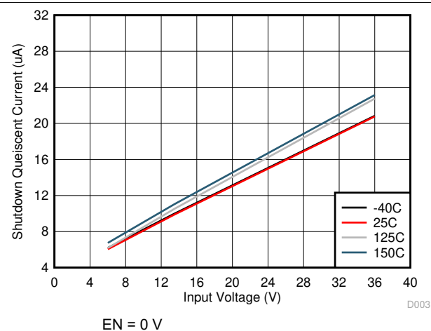
8-3. Shutdown Quiescent Current
