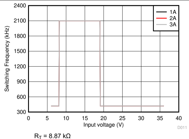
8-12. Switching Frequency vs VIN Voltage
