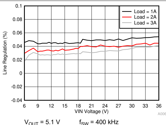
11-7. Line Regulation
