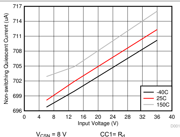
8-1. Non-Switching Quiescent Current
