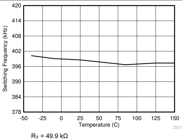
8-11. Switching Frequency vs Junction Temperature
