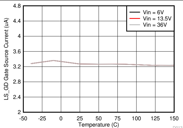
8-15. LS_GD Gate Source Current vs Junction Temperature
