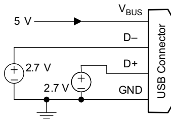
FIGURE 10-33. Divider 3 Mode
