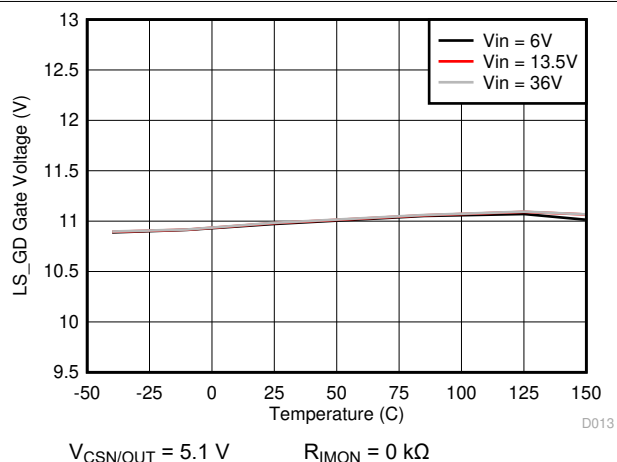
8-16. LS_GD Gate Voltage vs Junction Temperature
