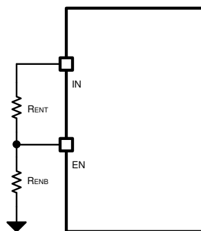
FIG 10-3. System UVLO by Enable Divider
