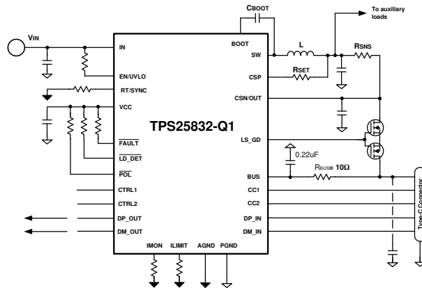
Figure 10-20. Current Limit with External MOSFET
