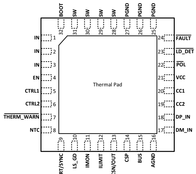
FIG 7-4. TPS25831QCWRHBRQ1 Package 32-Pin (VQFN) Top View
