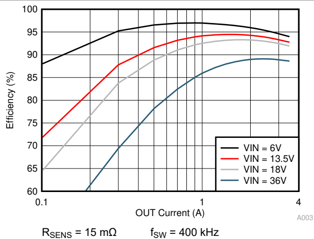
FIG 11-4. Efficiency With Sense Resistor
