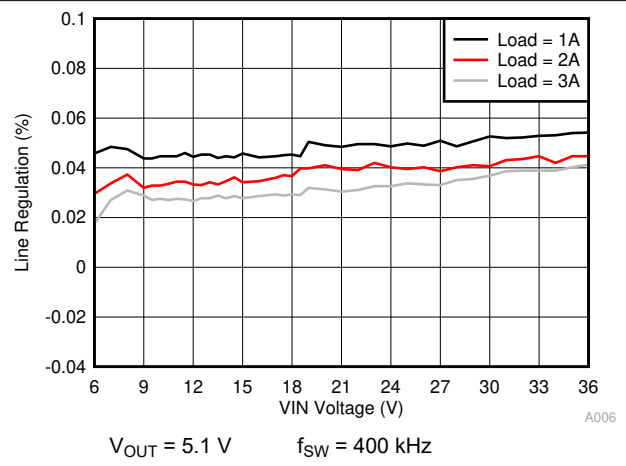
FIG 11-7. Line Regulation
