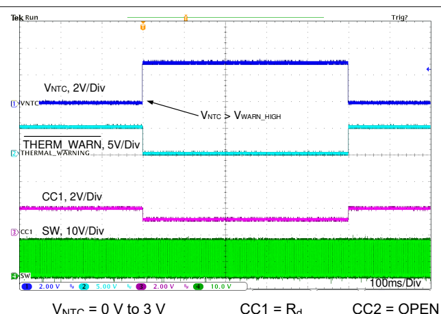
11-37. Thermal Sensing With NTC Behavior 1
