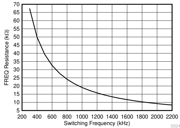
图 10-6. RT Set Resistor vs Switching Frequency
