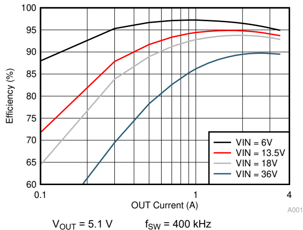
FIG 11-2. Buck Only Efficiency
