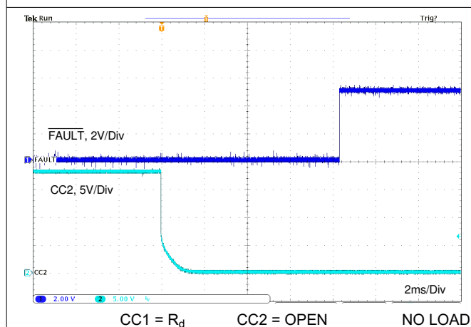
11-34. CC Short to BAT Recovery
