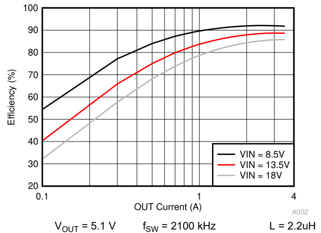
FIG 11-3. Buck Only Efficiency
