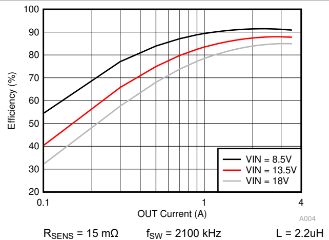
FIG 11-5. Efficiency With Sense Resistor
