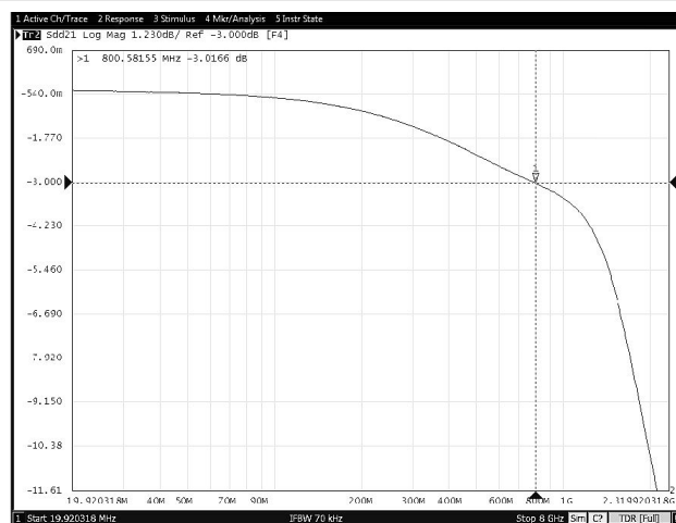
8-31. Data Transmission Characteristics vs Frequency (TPS25830-Q1)
