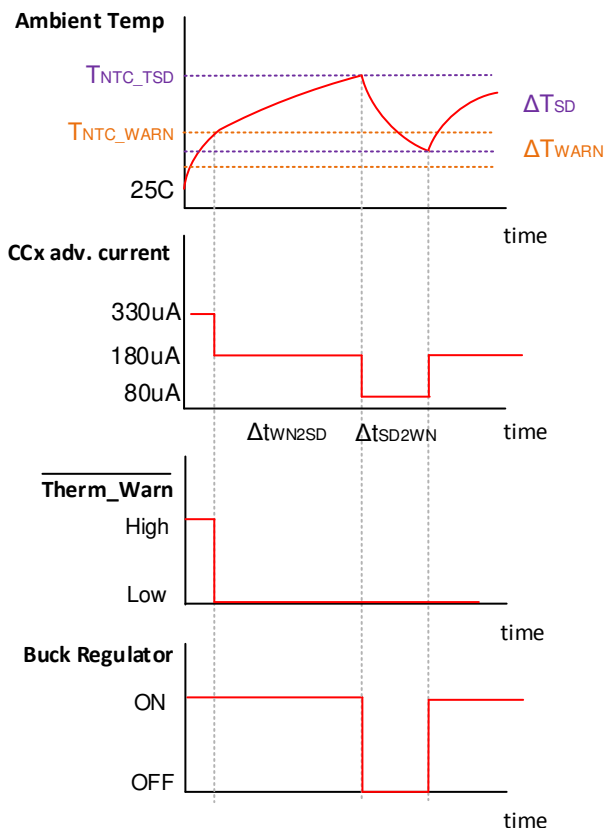
FIG 10-29. TPS25831-Q1 Behavior When Trigger NTC Threshold
