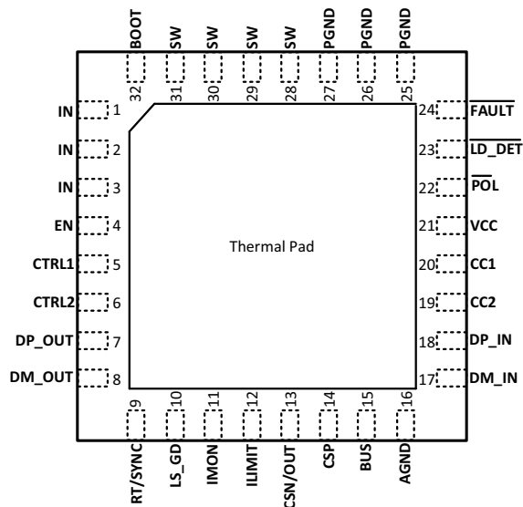
FIG 7-3. TPS25830QCWRHBRQ1 Package 32-Pin (VQFN) Top View
