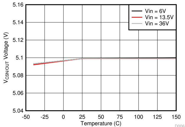
8-7. V_{CSN/OUT} Voltage vs Junction Temperature
