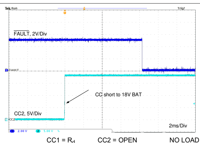
11-33. CC Short to BAT
