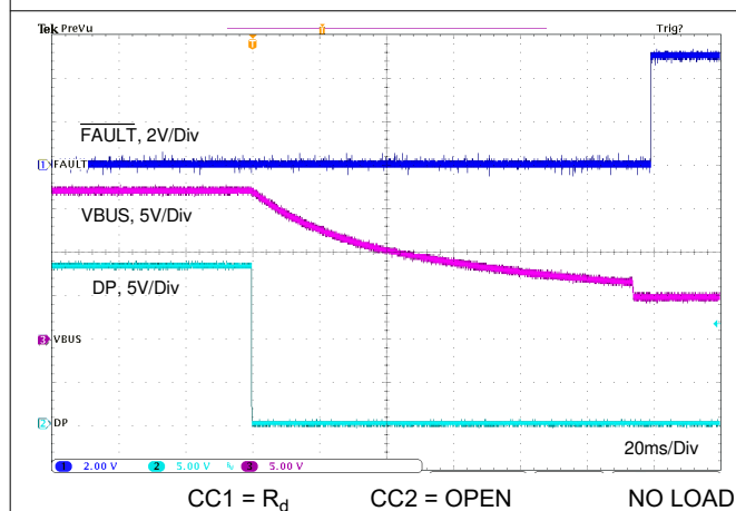
11-36. DP Short to BAT Recovery
