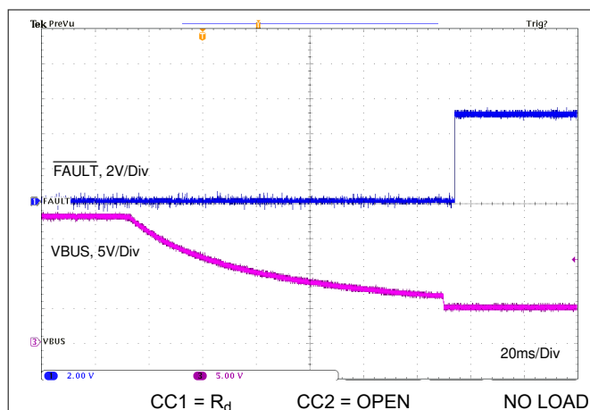
11-32. VBUS Short to BAT Recovery With External FET
