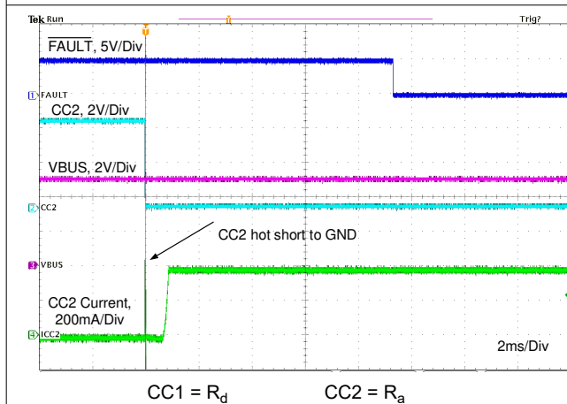
11-30. CC2 Hot Short to GND
