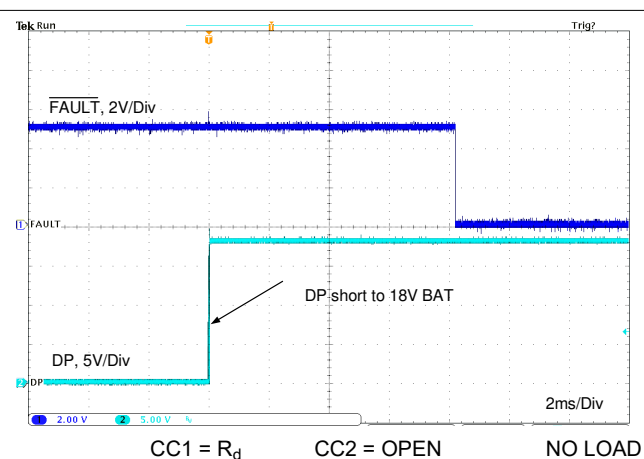
11-35. DP Short to BAT
