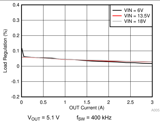
FIG 11-6. Load Regulation
