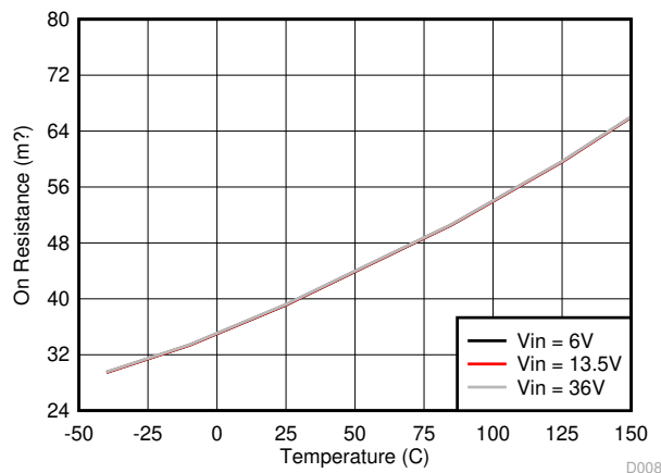
8-9. High-Side MOSFET on Resistance vs Junction Temperature
