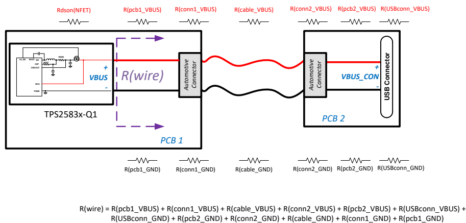
10-24. Automotive USB Resistances
