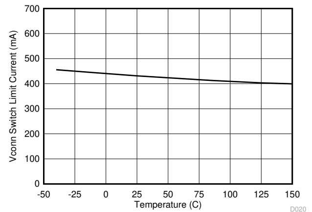
8-24. V CONN Switch Current Limit vs Junction Temperature V_{CONN} = 5\text{ V}
