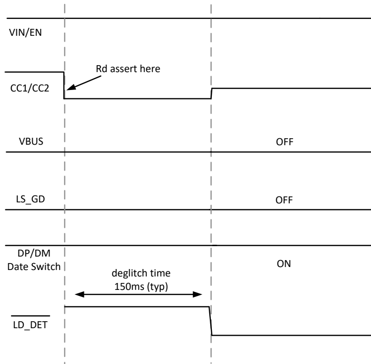
図 10-31. TPS2583xA-Q1 Startup Behavior Under Client Mode
