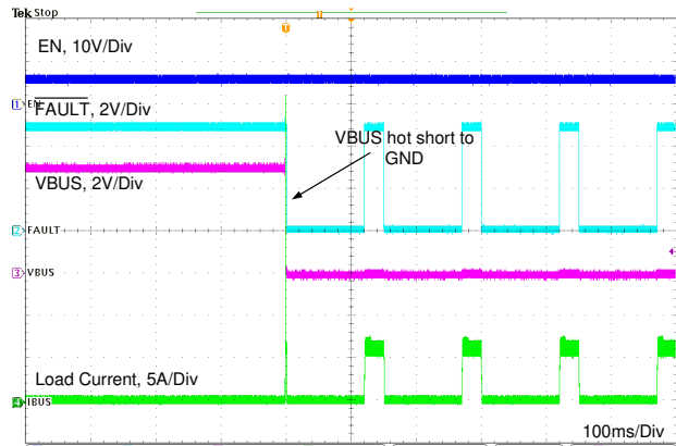
11-32. VBUS Hot Short to GND Without External FET
