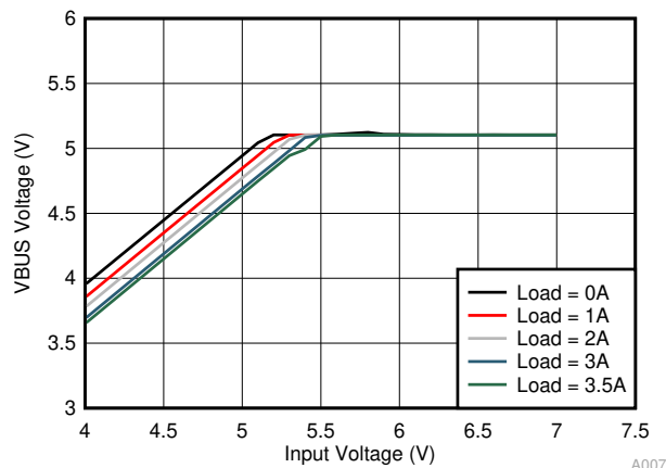
11-12. Dropout Characteristic
