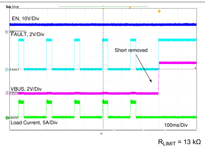
11-23. Short Circuit Recovery Without External FET
