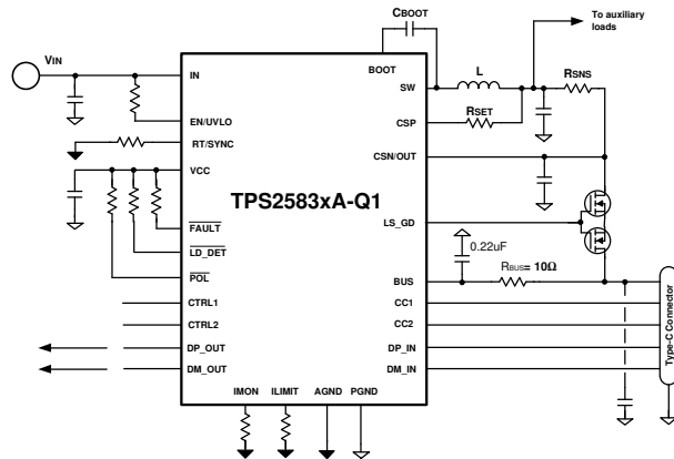
10-22. Current Limit with External MOSFET
