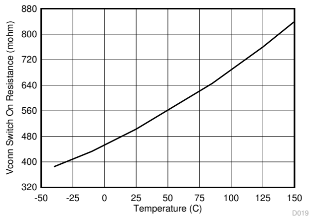
8-23. V CONN Current Limiting Switch On Resistance vs Junction Temperature V_{CONN} = 5\text{ V}
