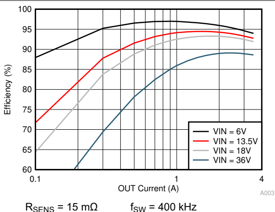
11-4. Efficiency With Sense Resistor
