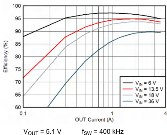
11-2. Buck Only Efficiency
