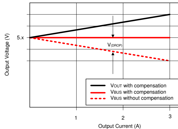
10-25. Voltage Drop
