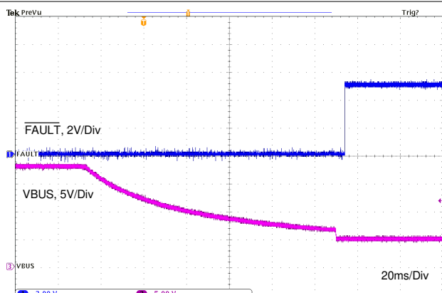
11-34. CC2 Hot Short to GND
