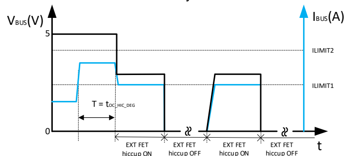
FIG 10-19. Two Level Current Limit Methodology with ext MOSFET Case 2
