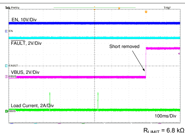
11-27. Short Circuit Recovery With External FET
