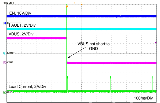
11-33. VBUS Hot Short to GND with External FET
