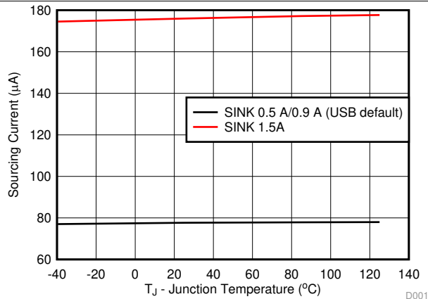
FIG 2. CC Sourcing Current to SINK vs Temperature
