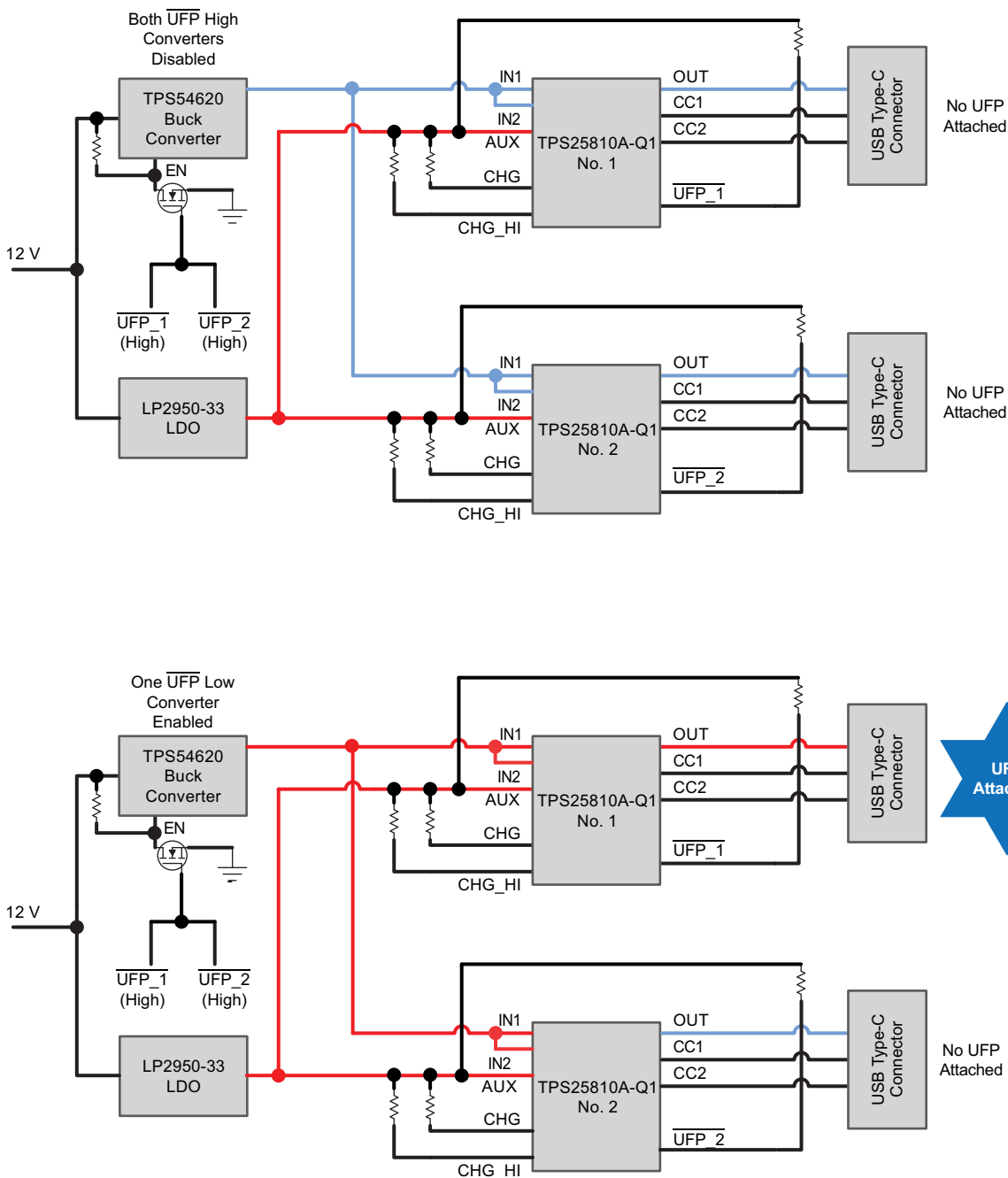
Figure 18. Power-Wake Implementation
