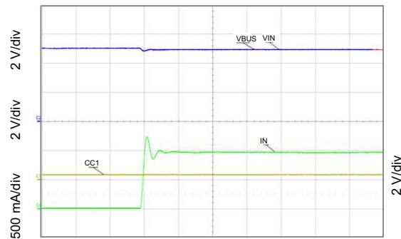
Figure 20. Basic Start-Up
