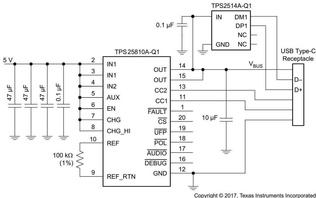
Figure 27. Type-C DFP Port Implementation With BC 1.2 (DCP Mode) Support
