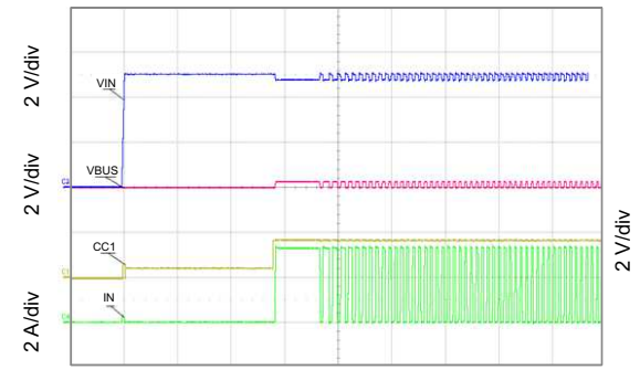
Figure 21. Start-Up
