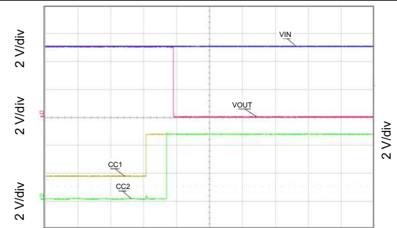
Figure 23. Hot-Plug to Short
