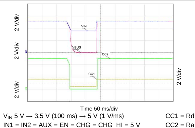
Figure 26. Brown-Out Test
