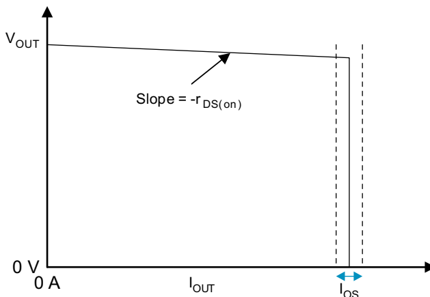
Figure 13. Current-Limit Profile
