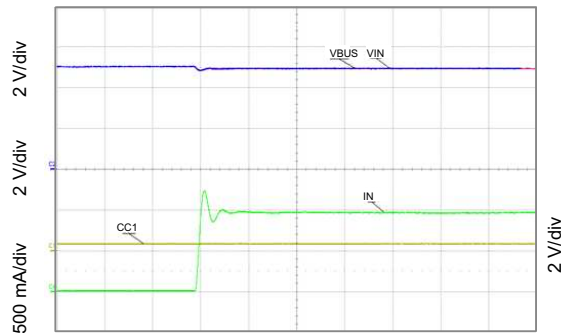
Figure 21. Basic Start-Up
