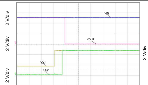
Figure 24. Hot-Plug to Short
