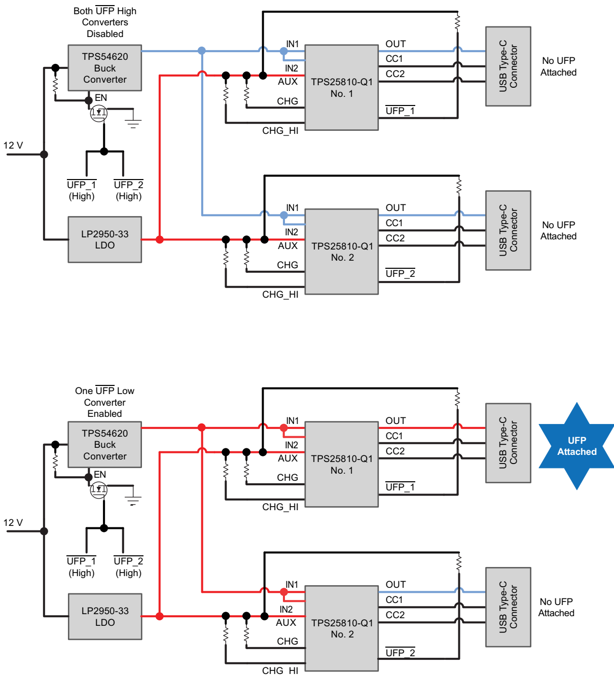
Figure 16. Power-Wake Implementation
