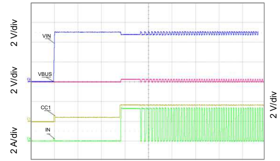
Figure 22. Start-Up
