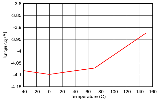
図 6-21. Buck Negative Current Limit vs Temperature
