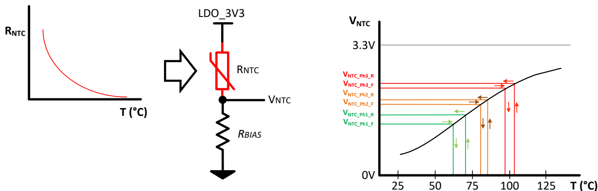
図 8-44. NTC Response Curve
