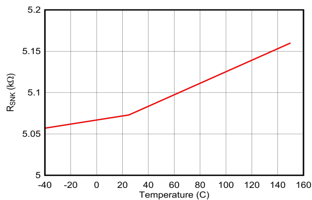
Figure 6-38. Type-C Cable Detect: R_{SNK} vs Temperature
