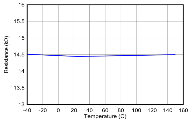
図 6-43. USB BC1.2: DM to AGND 15 kΩ Resistance, R_{DM\_DWN\_15k}
