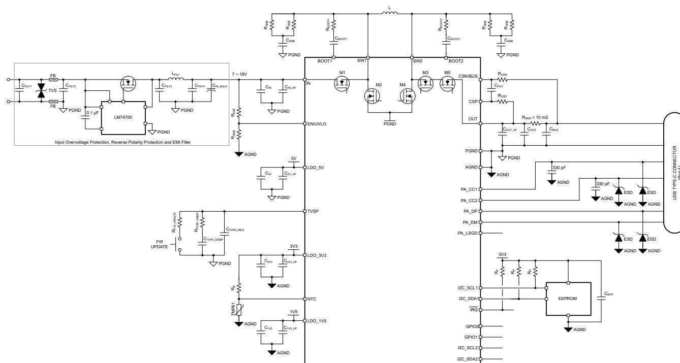
9-3. TPS25762-Q1 Application Schematic
