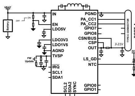
図 9-1. Simplified Single USB PD Charger
