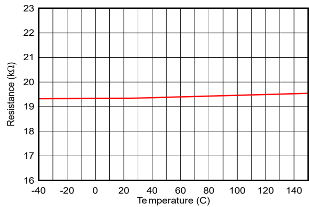
図 6-44. USB BC1.2: DM to AGND 20 kΩ Resistance, R_{DM\_DWN\_20k}
