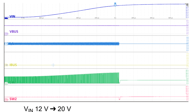
9-27. V_{IN(OVP)} Entry
