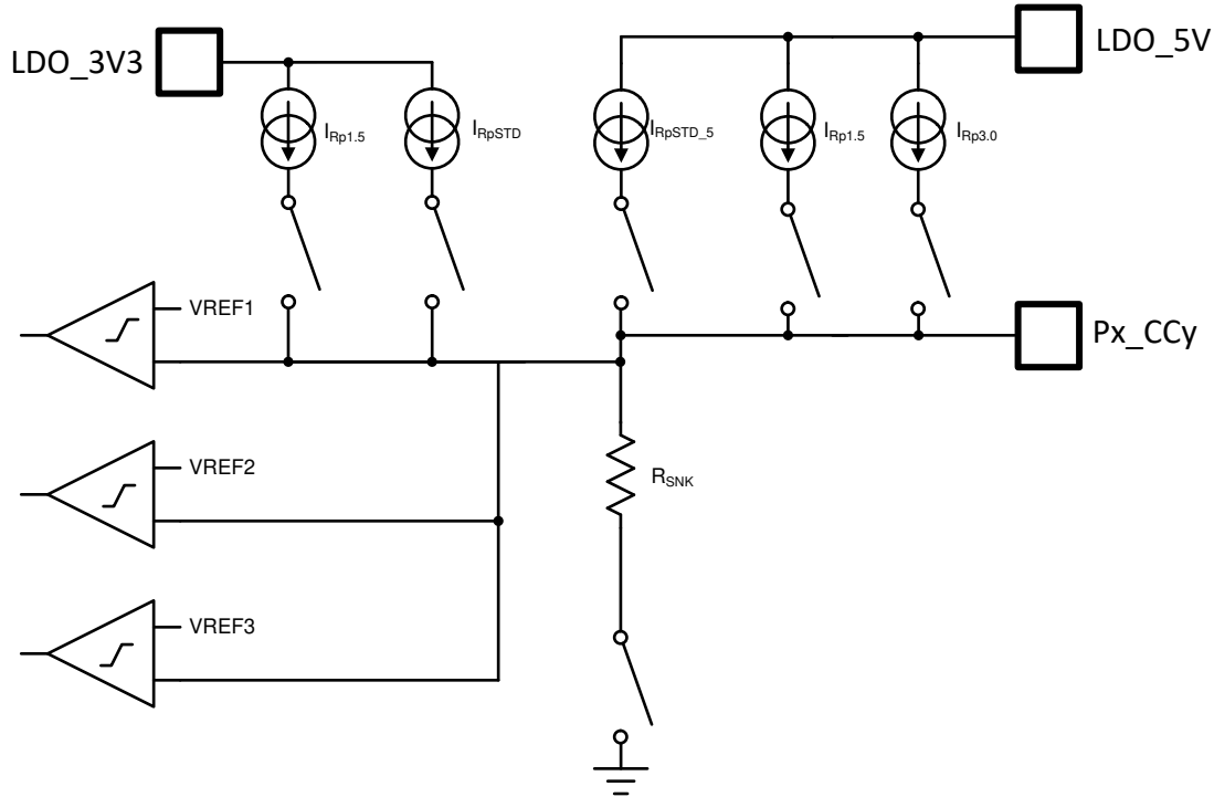
8-27. Plug and Orientation Detection Block
