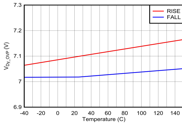
図 6-45. USB BC1.2: DP and DM Pin Over-voltage Protection Thresholds vs Temperature
