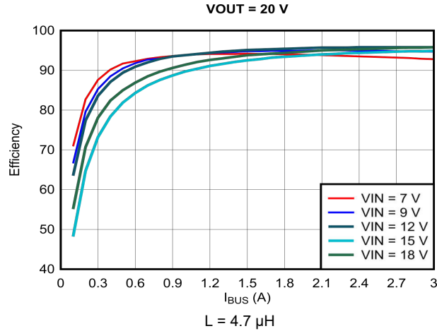
9-10. Efficiency vs Output Current ( I_{OUT} ), V_{OUT} = 20\text{ V}
