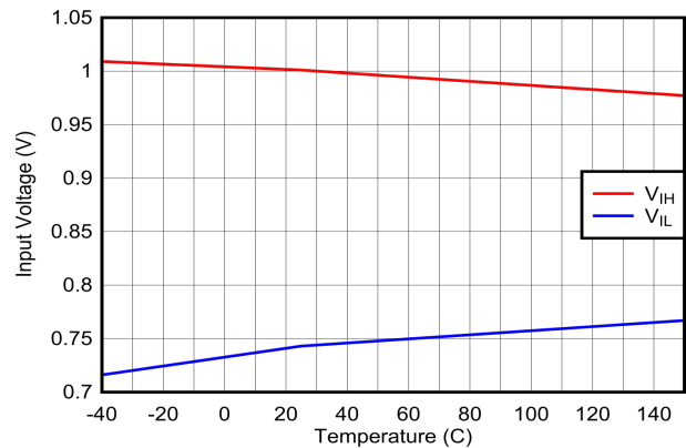
図 6-48. GPIO: Input Voltage Thresholds vs Temperature
