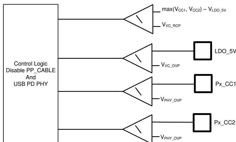
图 8-29. Over-voltage and Reverse Current Protection
