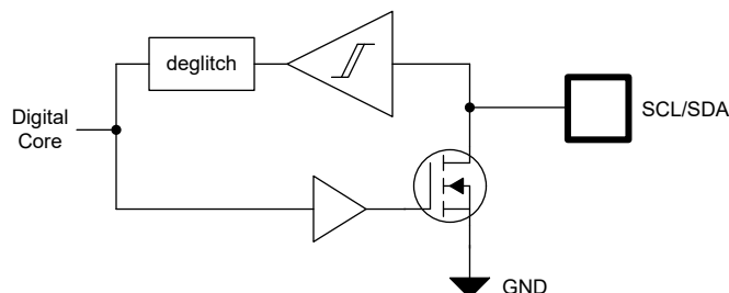
8-34. I 2 C Driver
