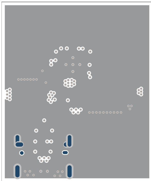
図 9-39. TPS25751S PCB Layout - GND Layer
