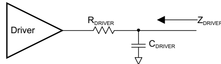
✎ 8-9. Z DRIVER Circuit
