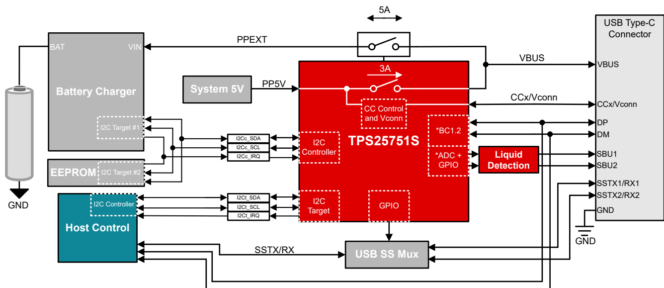
図 9-13. TPS25751S USB Data Support
