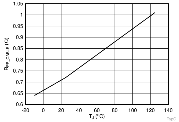
図 6-2. PP_CABLE Rdson vs. Temperature
