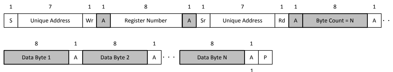
図 8-31. I²C Unique Address Read Register Protocol
