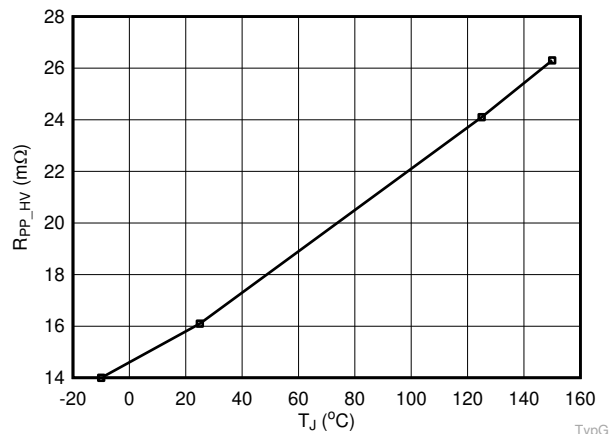
図 6-5. R PPHV vs. Temperature for TPS25751D
