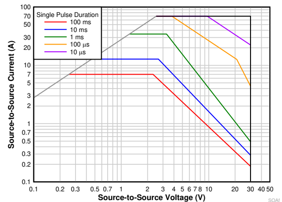
図 6-6. Safe-Operating-Area (SOA) of PPHV for TPS25751D
