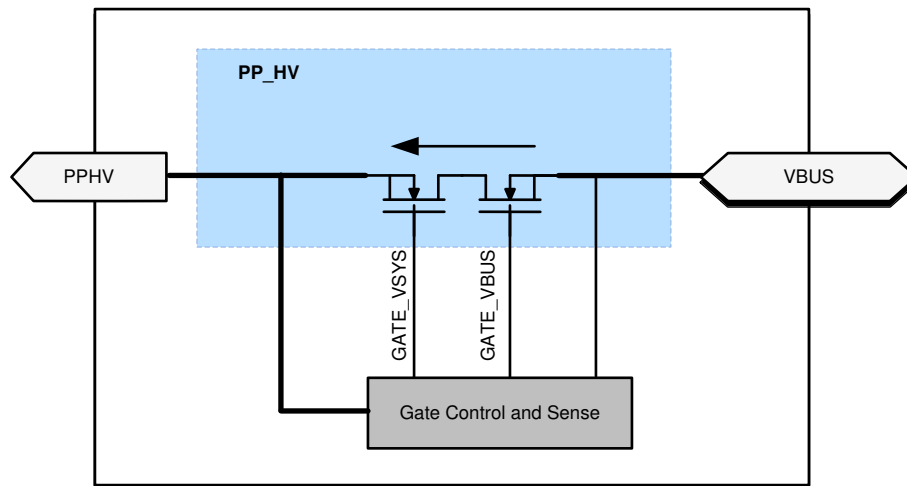
図 8-13. Internal Sink Path
