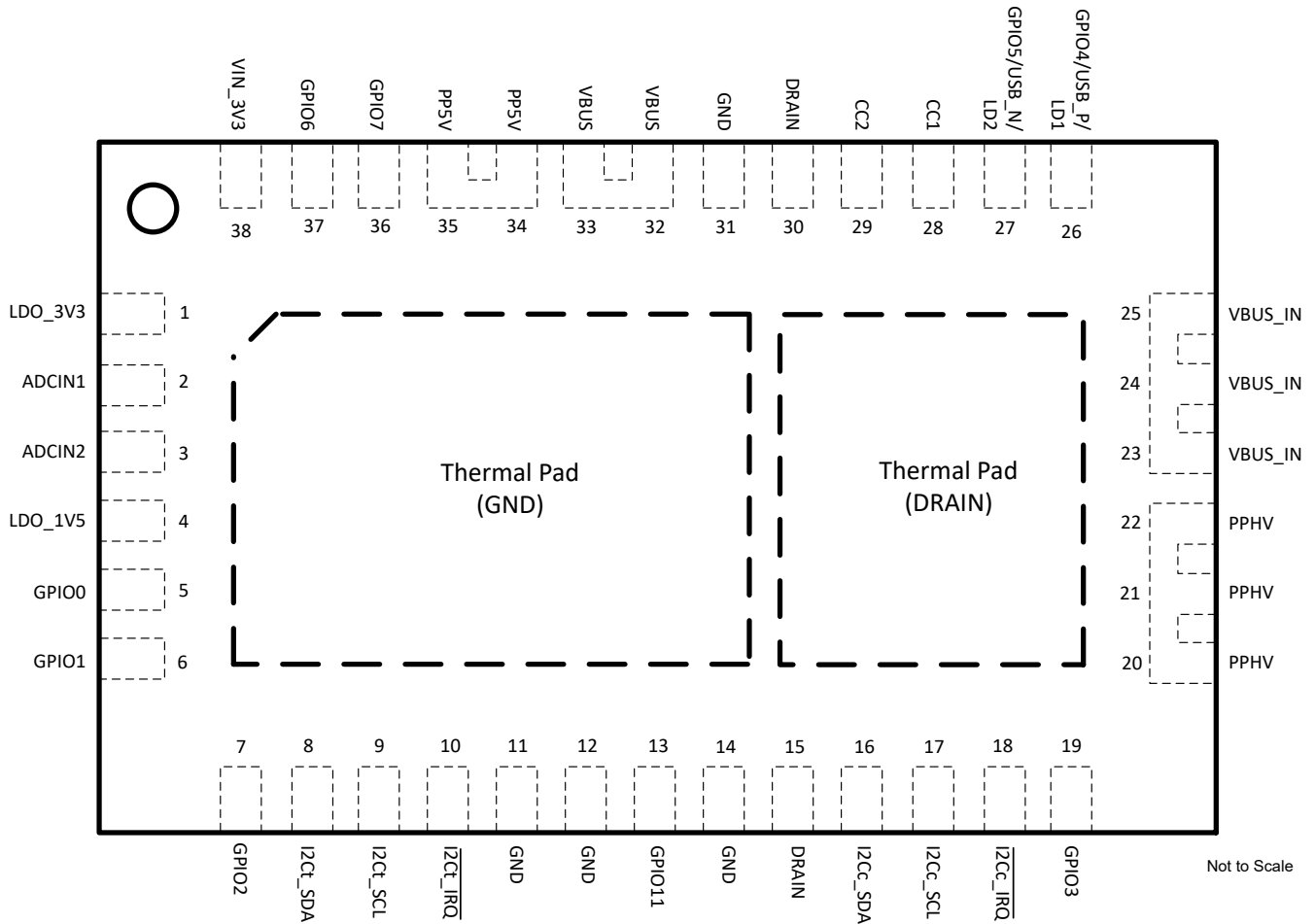
図 5-1. Top View of the TPS25751D 38-pin QFN Package
