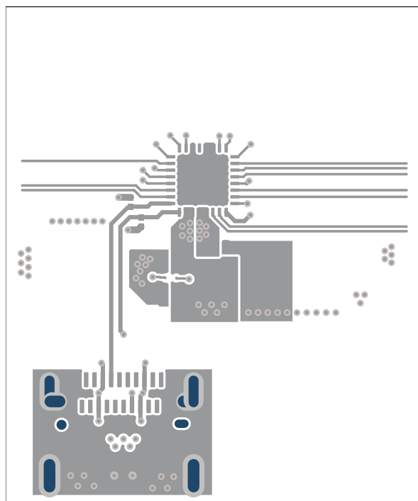
図 9-37. TPS25751S PCB Layout - Top Layer Routing
