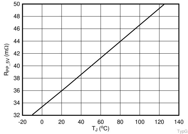
図 6-1. PP_5V Rdson vs. Temperature.
