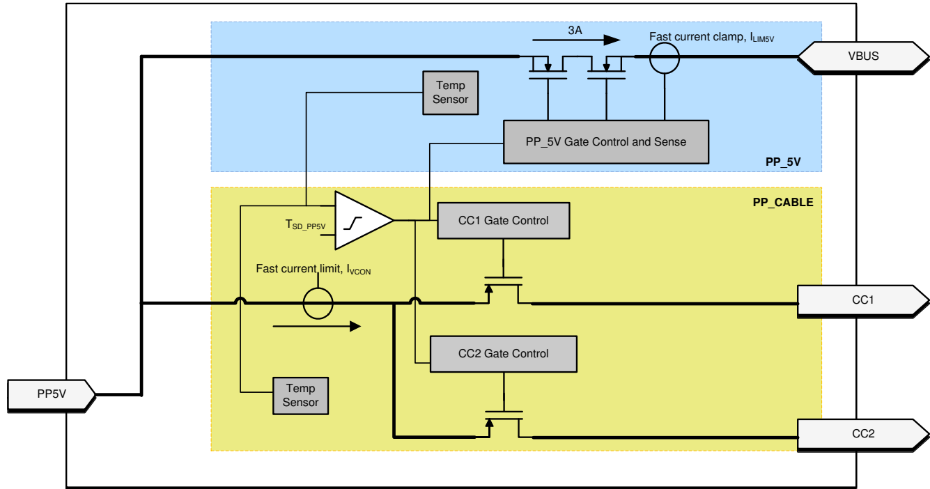
図 8-12. Port Power Switches
