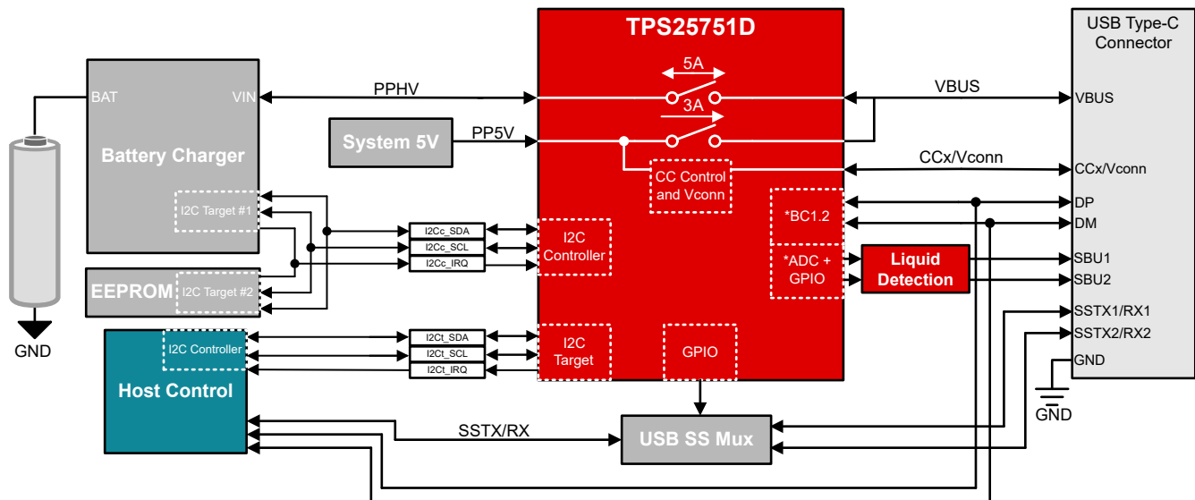
図 9-12. TPS25751D USB Data Support
