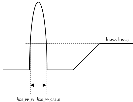
図 7-2. Short-circuit Response Time for Internal Power Paths PP_5V and PP_CABLE
