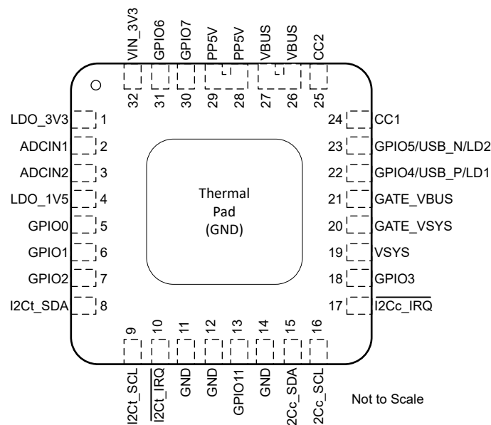
図 5-2. Top View of the TPS25751S 32-pin QFN Package
