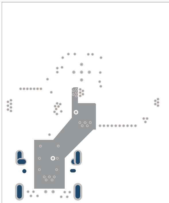
図 9-38. TPS25751S PCB Layout - Internal Power Layer
