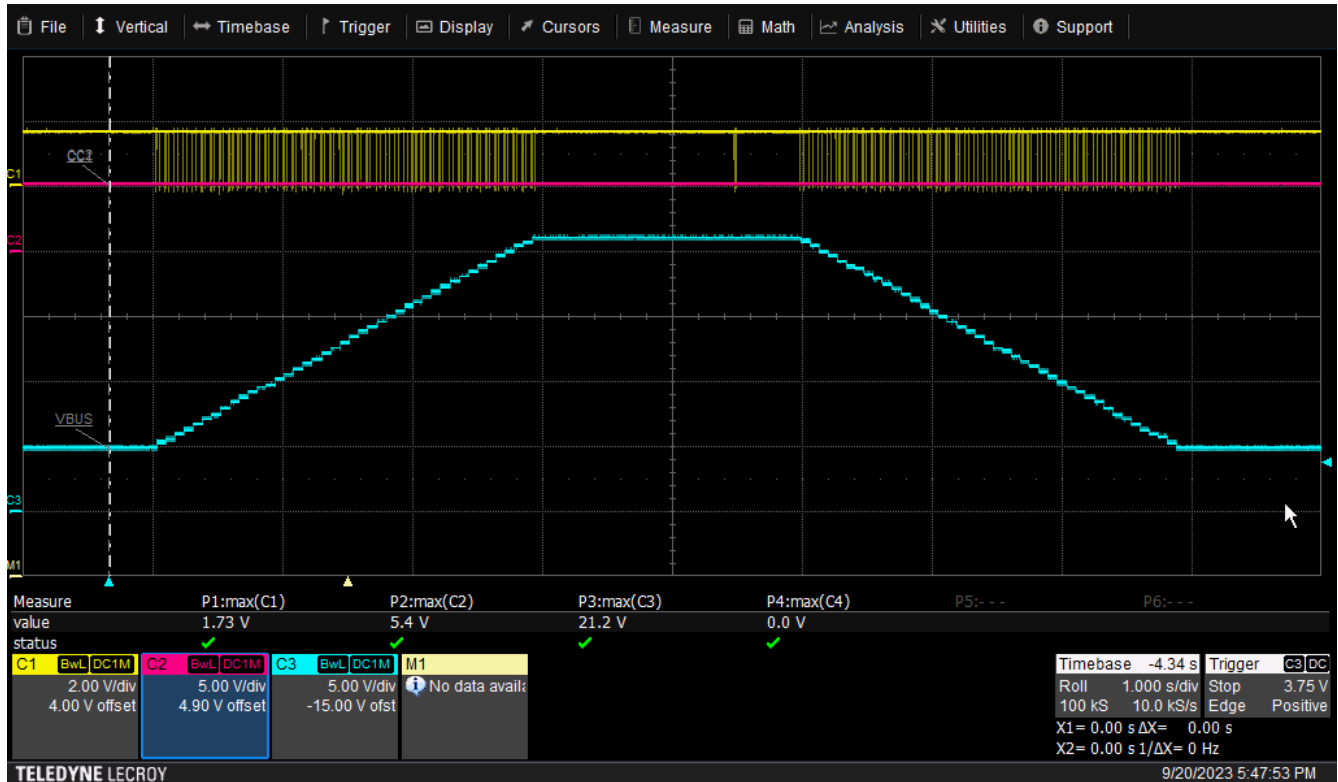
図 9-14. PPS PD Negotiation VBUS Increasing/Decreasing
