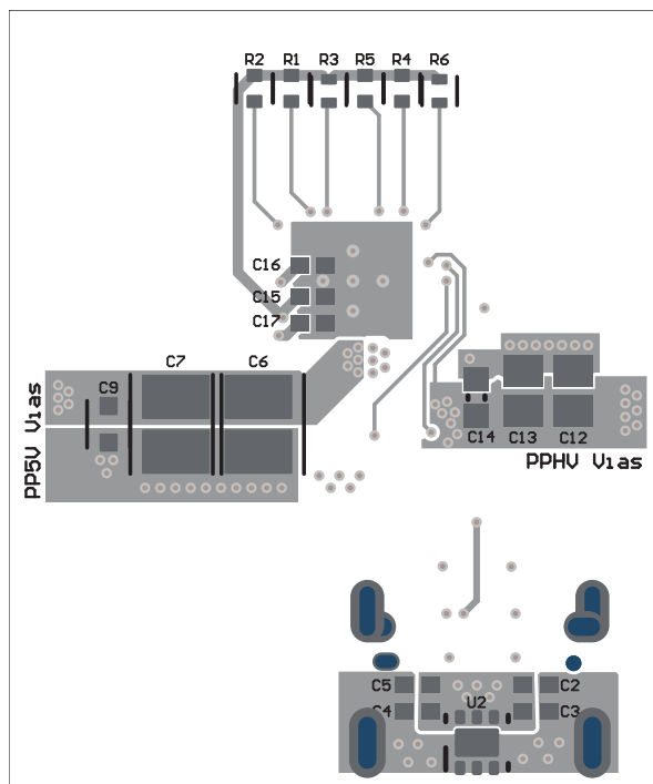
図 9-36. TPS25751S PCB Layout - Bottom Composite
