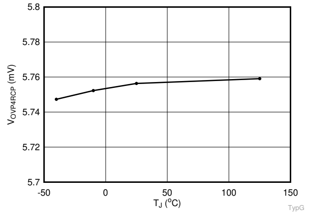
図 6-4. V OVP4RCP (Setting 2) vs. Temperature
