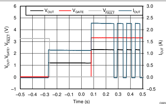
9-13. Auto-Retry Cycle
