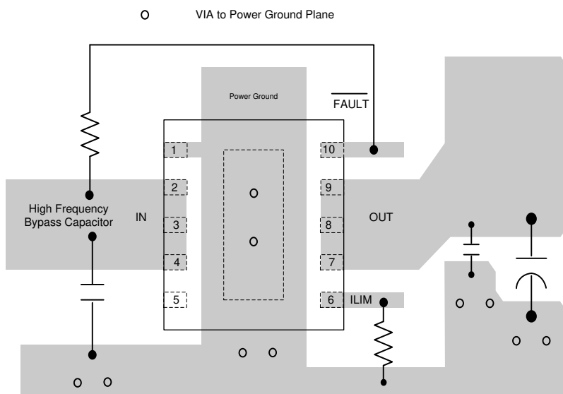
11-1. TPS2559 Board Layout
